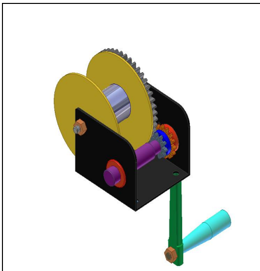
Fig 2a Gear box assembly
