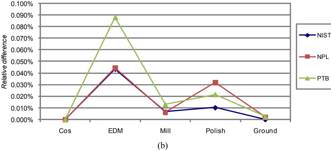
Figure 23: R_{ku} parameter analysis
