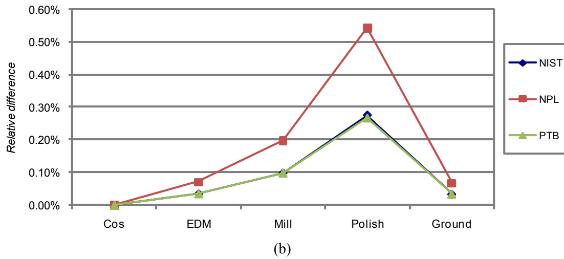
Figure 25: R_p parameter analysis
