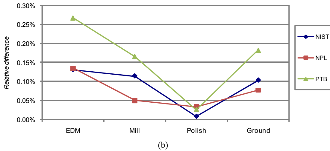
Figure 21: R_{sk} parameter analysis
