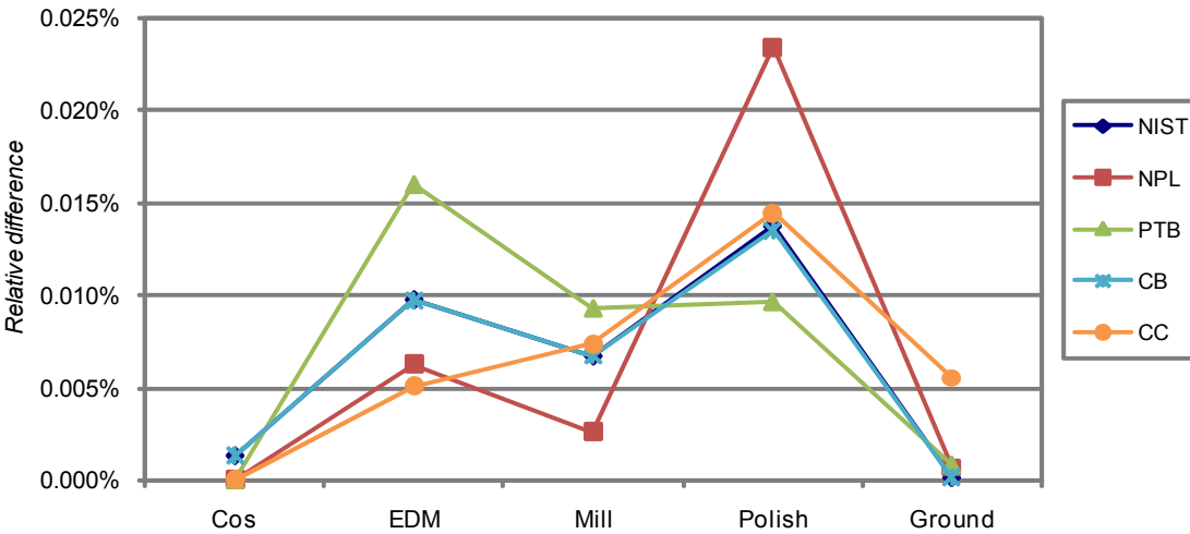
Figure 24: P_{ku} parameter analysis
