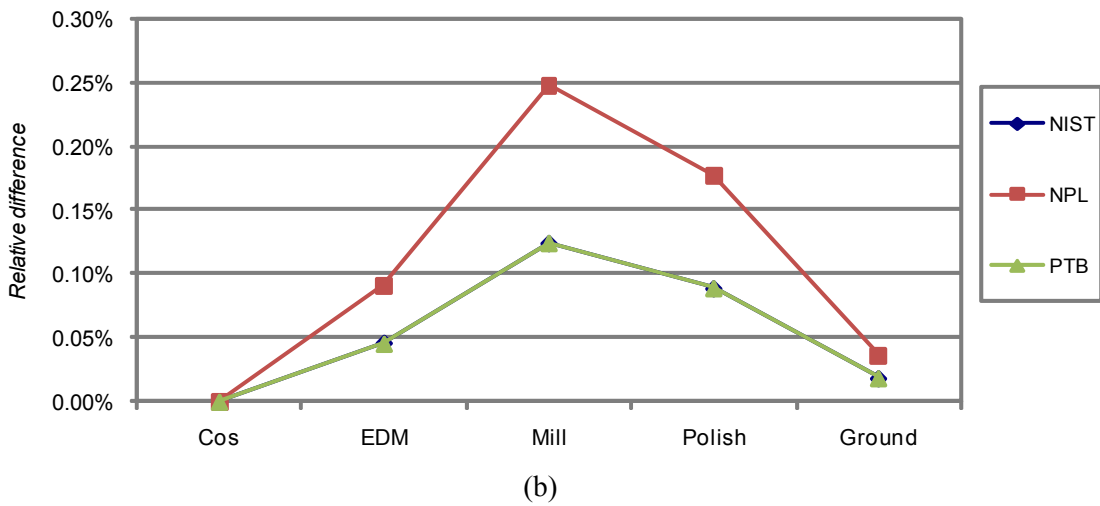
Figure 27: R_v parameter analysis
