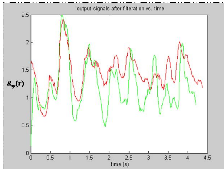
Figure 3 Film thickness signals from both upstream and downstream sensors
