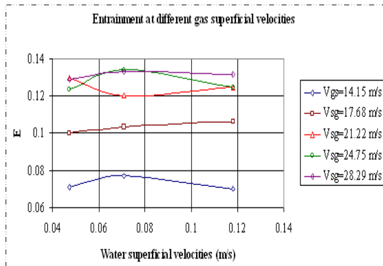
Figure 9 Entrainment at different gas superficial velocities
