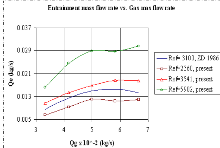
Figure 7 Entrainment mass flow rate at different liquid feed Reynolds number
