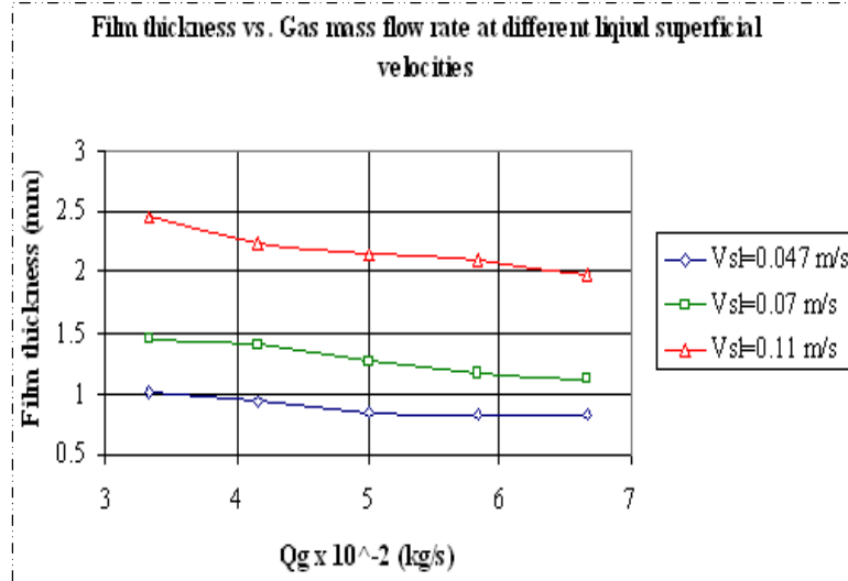
Figure 6 Liquid film thicknesses at different liquid superficial velocities
