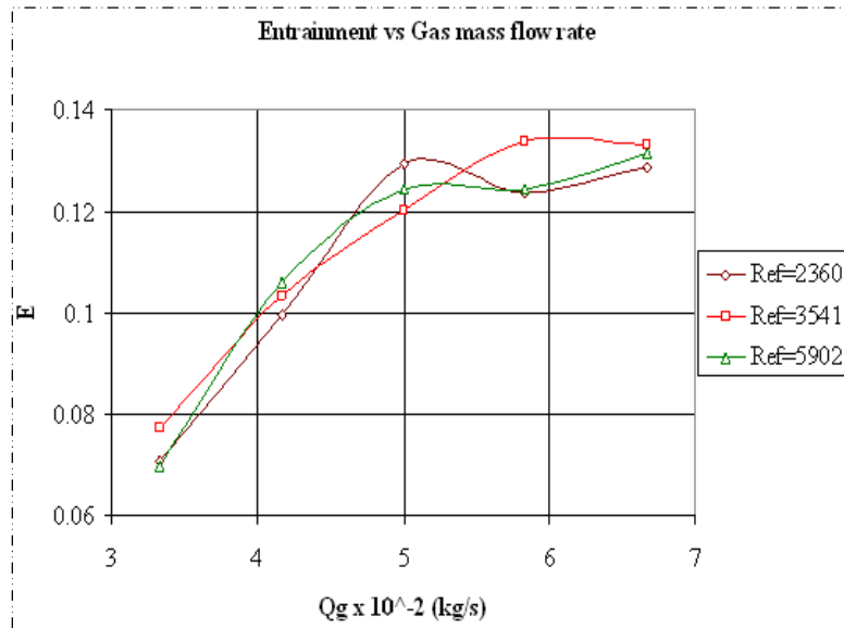
Figure 8 Entrainment at different liquid feed Reynolds number
