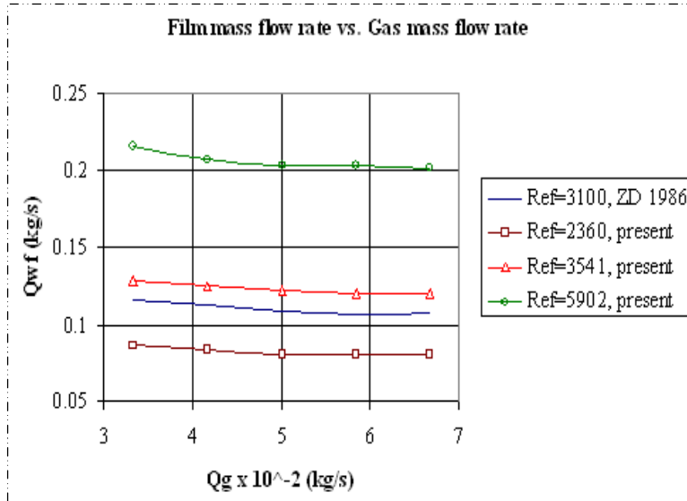
Figure 10 Liquid film mass flow rate at different liquid feed Reynolds number
