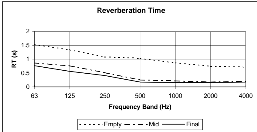
Figure 5 - Reverberation Time of Control Room
