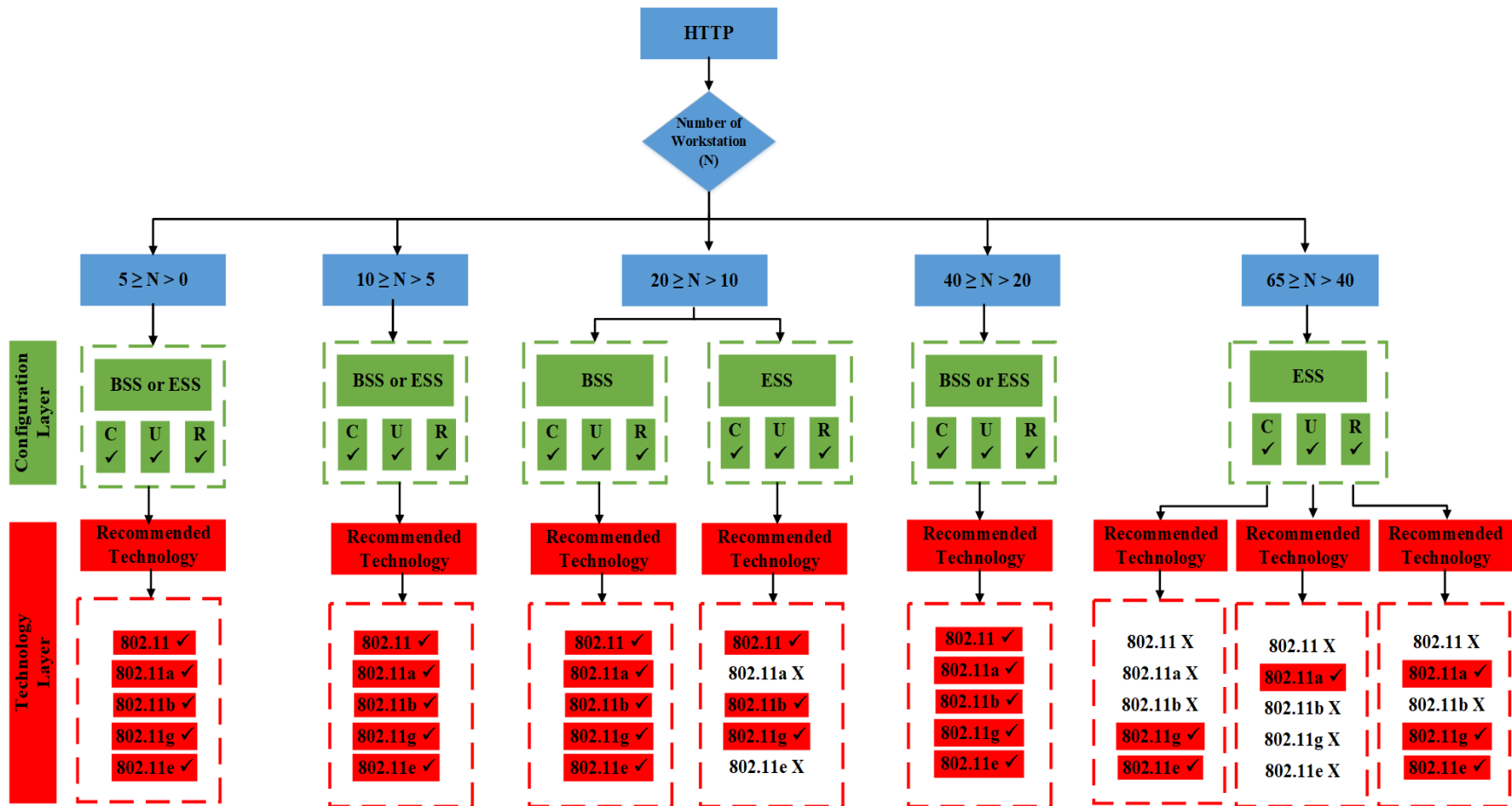
Figure 5. 5 Generic flowchart of the proposed algorithm for HTTP
