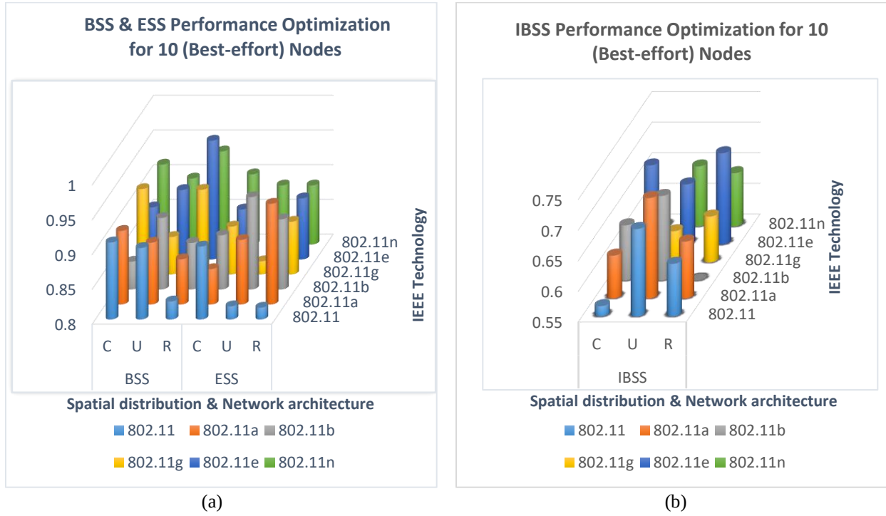
Figure 6. 11 Performance Optimization for 10 (Best-effort) nodes.
