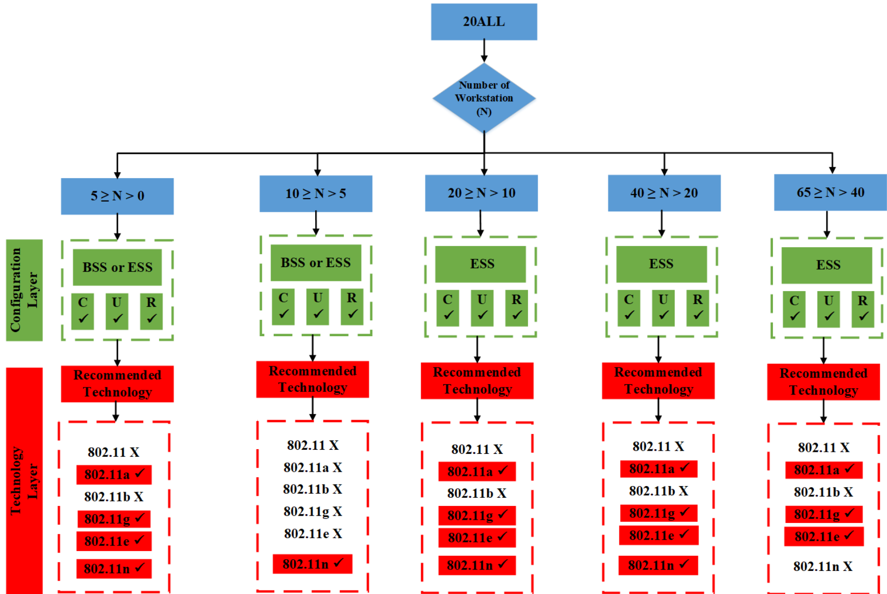
Figure 6. 17 Generic flowchart of the proposed algorithm for 20ALL
