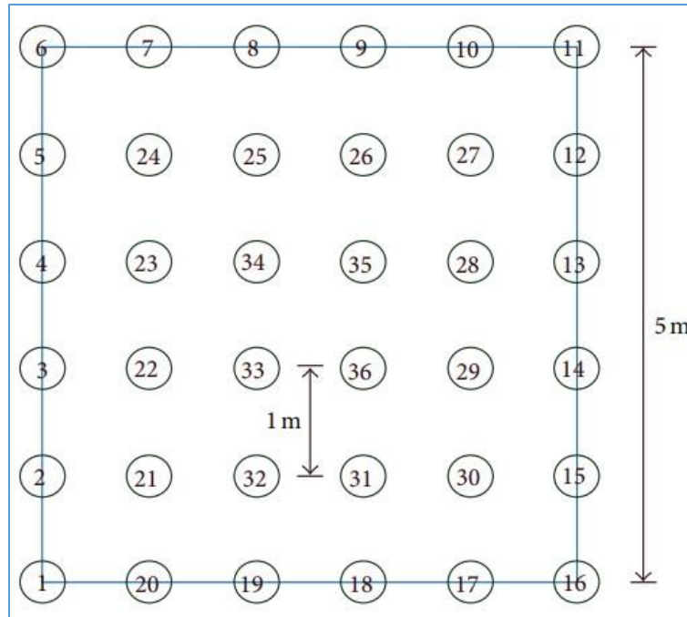
Figure 3. 14 Uniform/ Grid layout of WLAN nodes (Norouz & Zaim, 2014)
