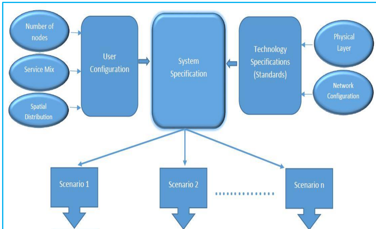
Figure 3. 16 Algorithm's Inputs
