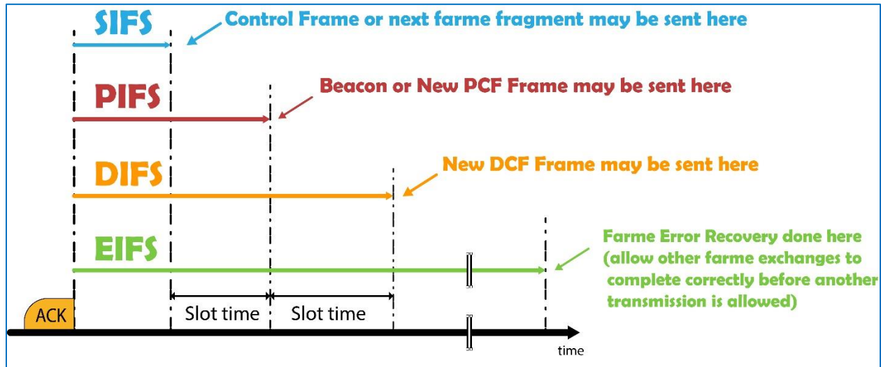
Figure 2. 8 Inter frame Spacing (Refaet, Amed, Abed, & Aish, 2020)
