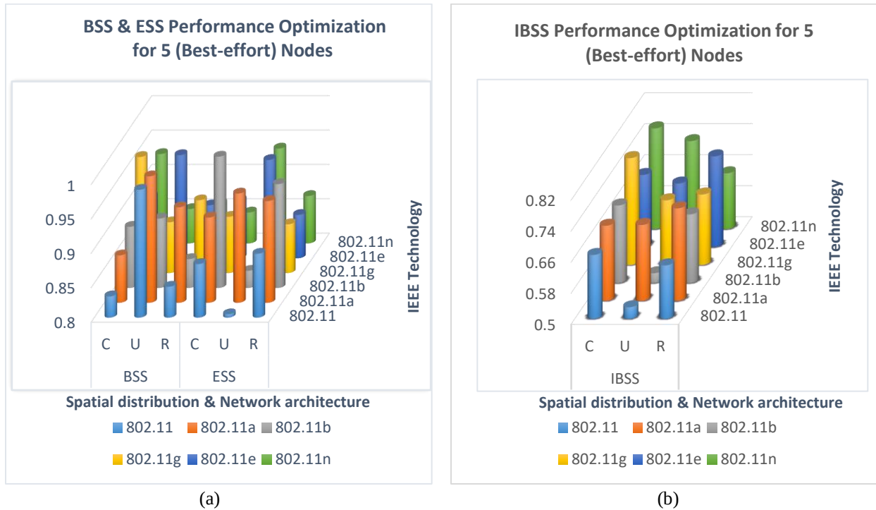
Figure 6. 10 Performance Optimization for 5 (Best-effort) nodes.
