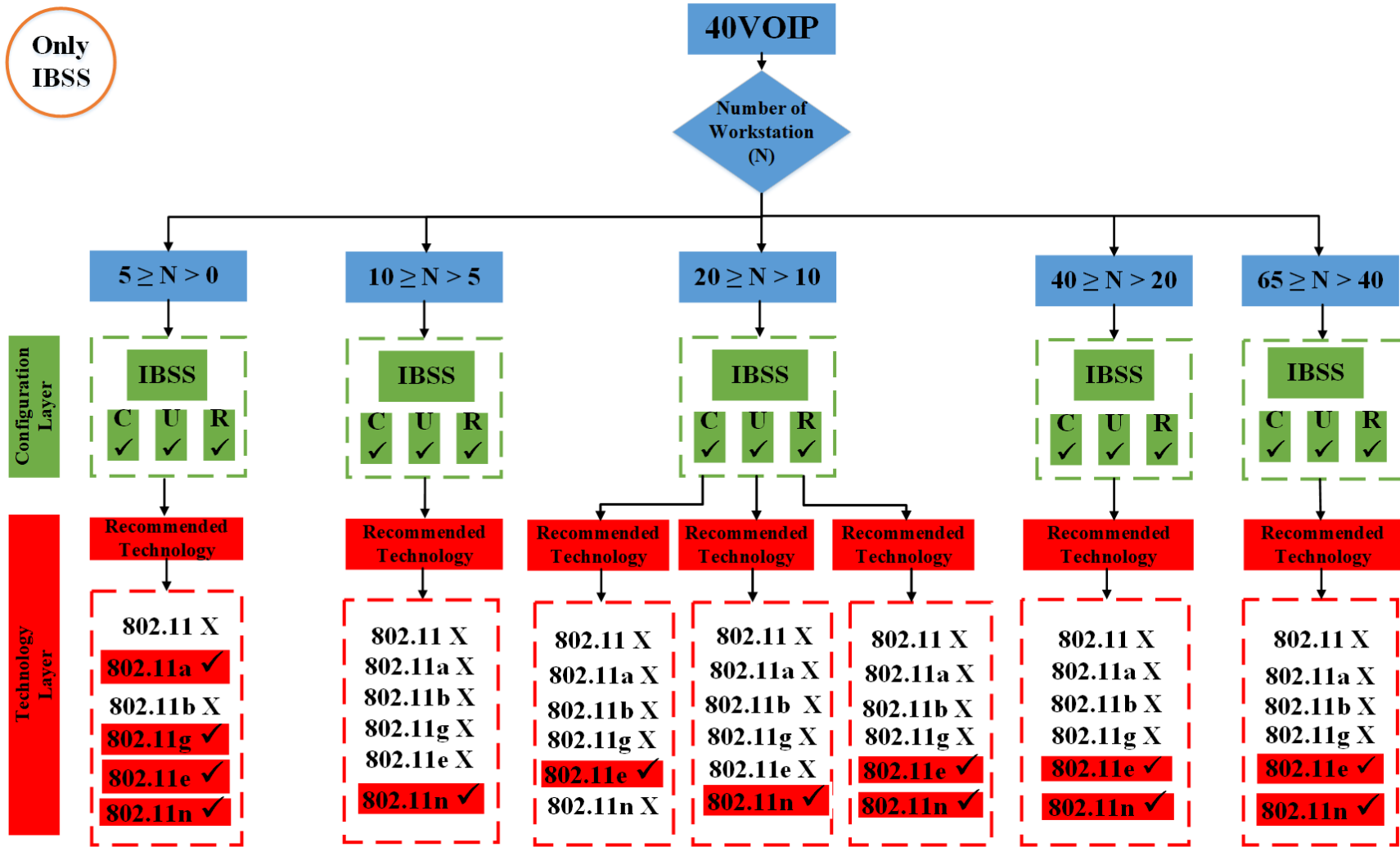
Figure 6. 28 Flowchart of only IBSS's results for 40VOIP
