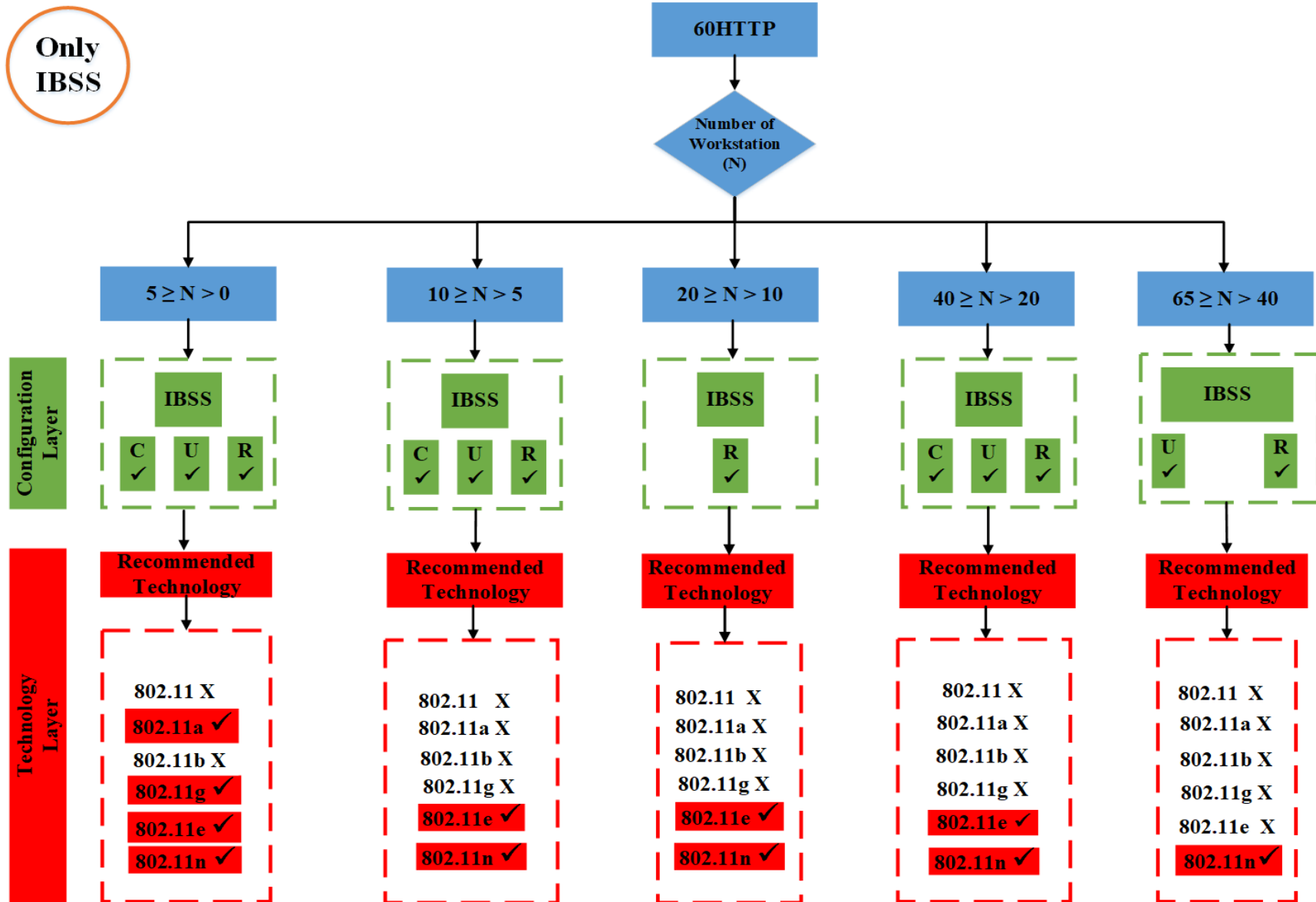
Figure 6. 22 Flowchart of only IBSS's results for 60HTTP
