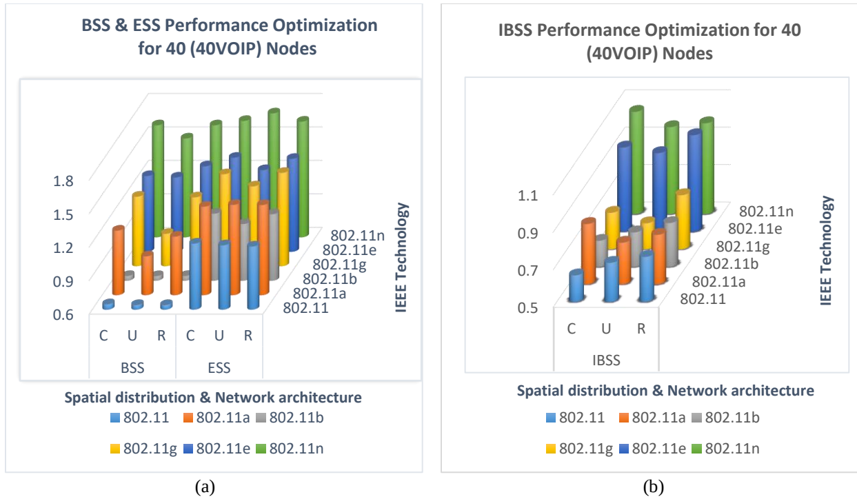
Figure 6. 33 Performance Optimization for 40 (40VOIP) nodes. (a) BSS & ESS, (b) only IBSS
