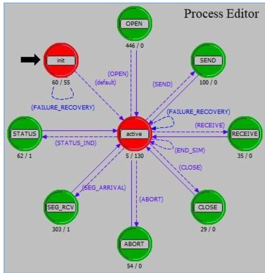
Figure 3. 9 Process Editor View (Riverbed, 2017)
