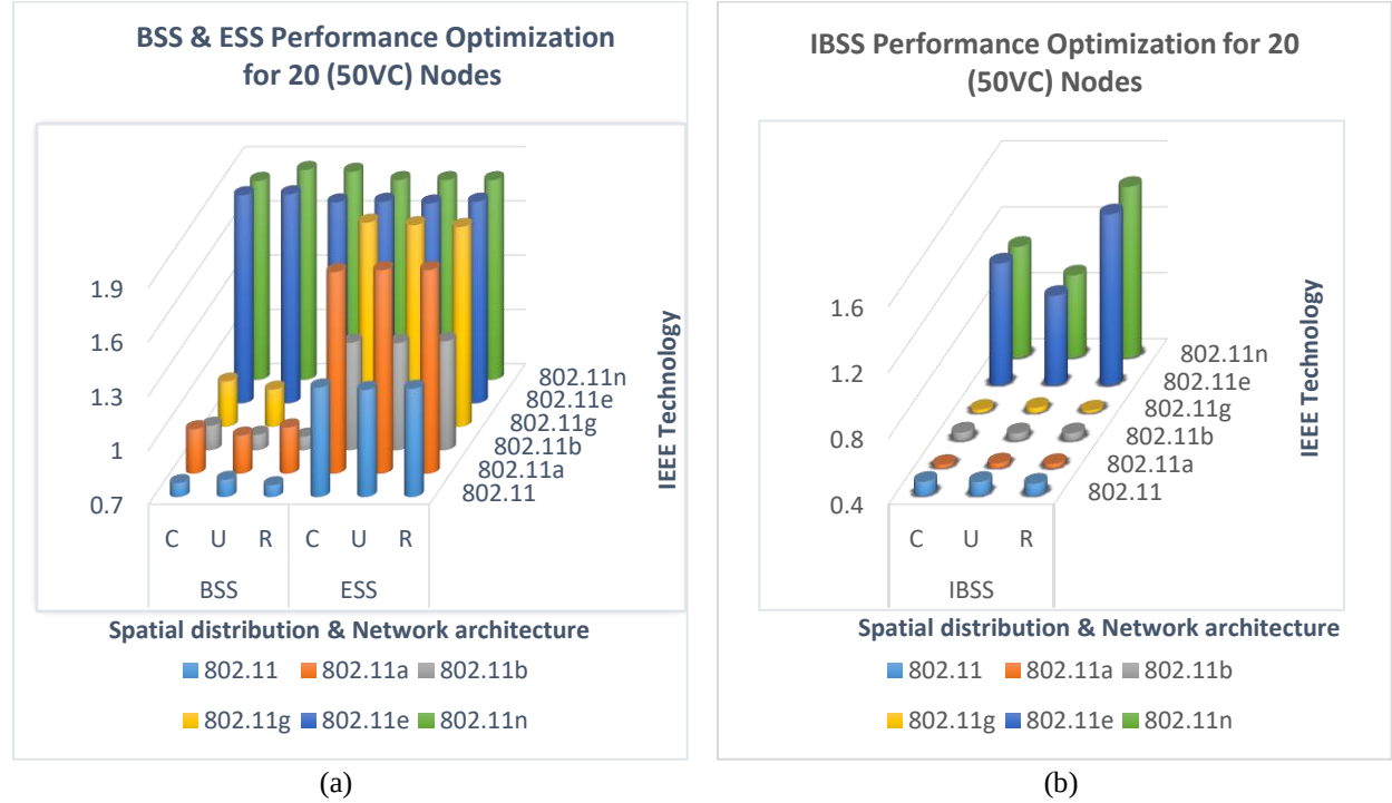
Figure 6. 5 Performance Optimization for 20 (50%VC nodes). (a) BSS & ESS, (b) only IBSS
