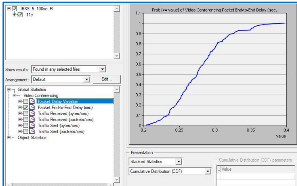
Figure 4.11 Delay result of IBSS_5_100VC_R
