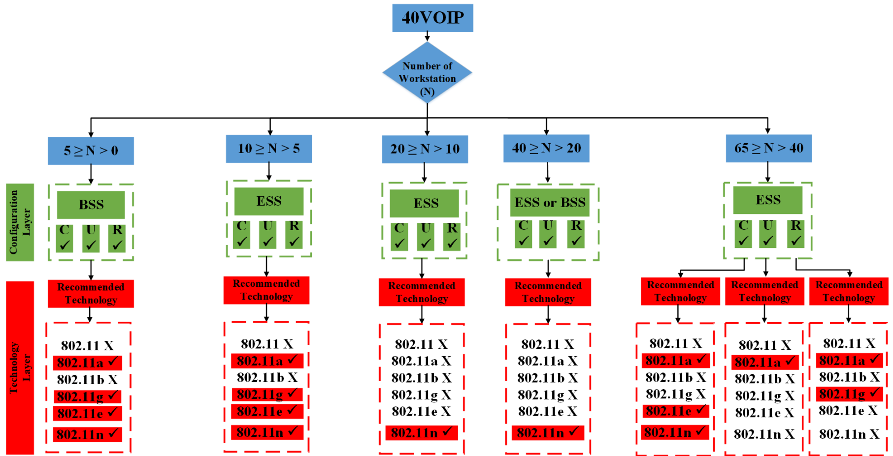
Figure 6. 27 Generic flowchart of the proposed algorithm for 40VOIP
