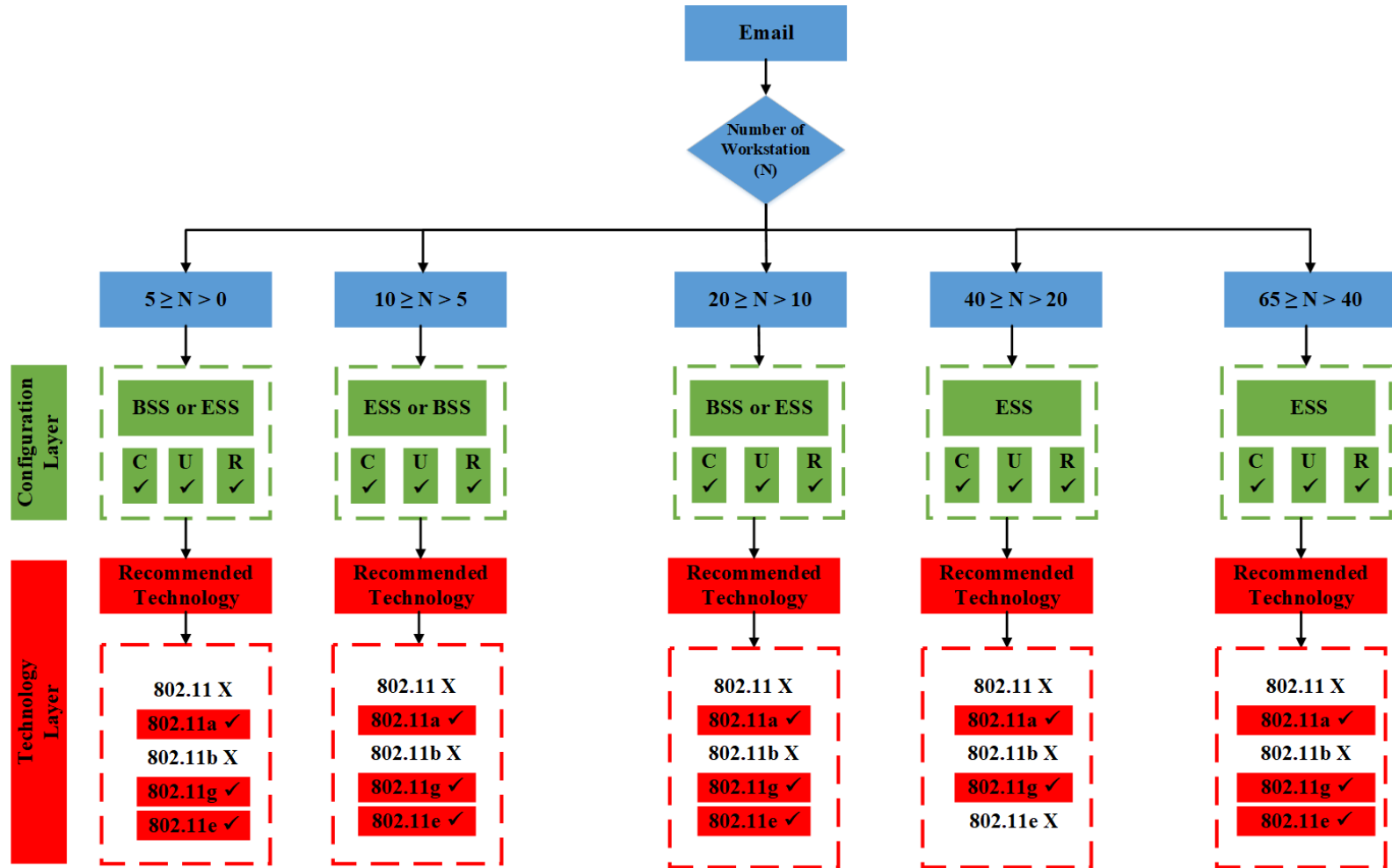
Figure 5. 9 Generic flowcharts of the proposed algorithm for Email
