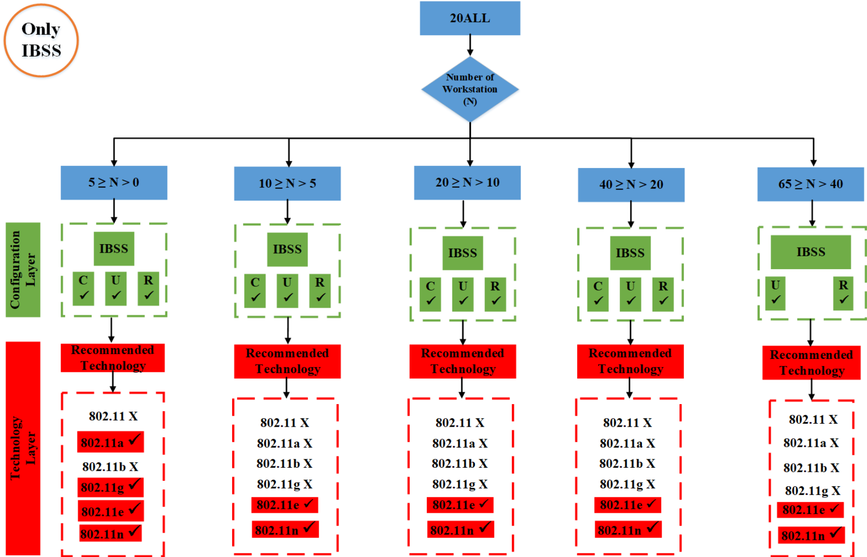
Figure 6. 18 Flowchart of only IBSS's results for 20ALL
