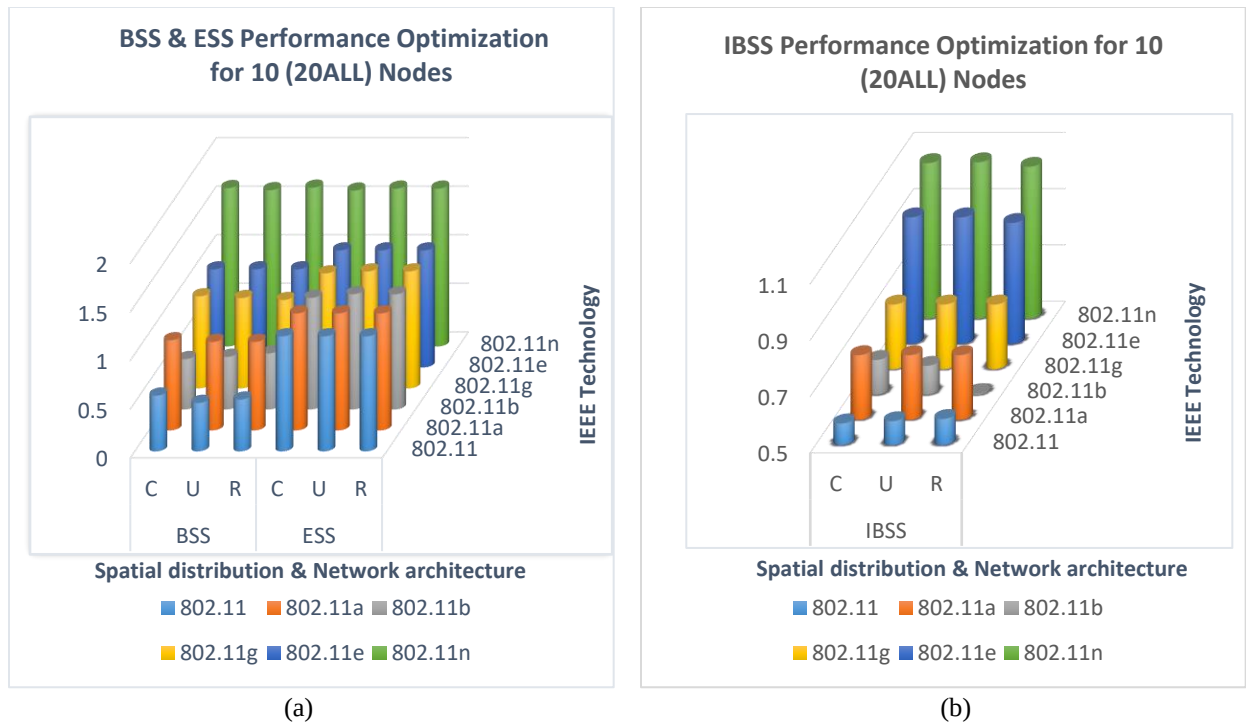
Figure 6. 16 Performance Optimization for 10 (20 ALL) nodes. (a) BSS & ESS, (b) only IBSS
