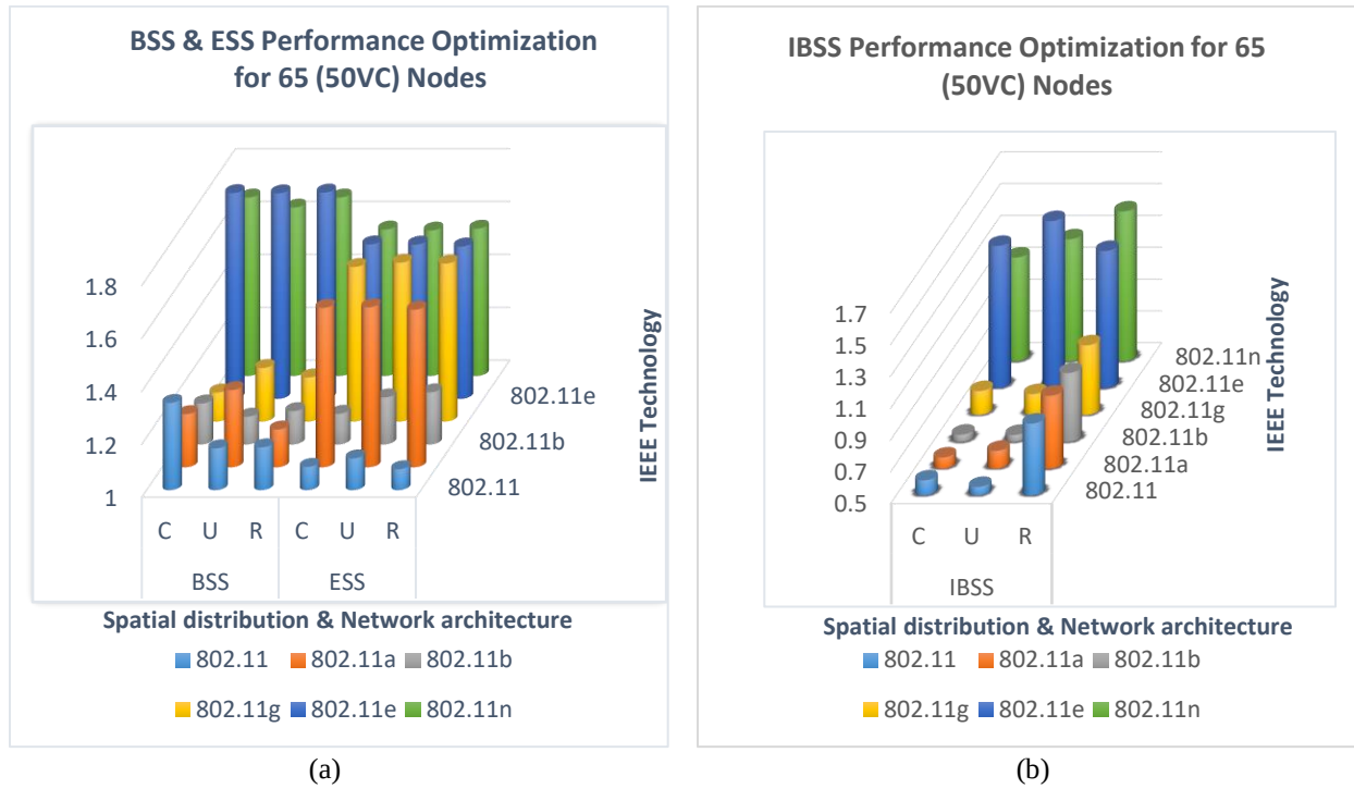
Figure 6. 7 Performance Optimization for 65 (50%VC nodes).
