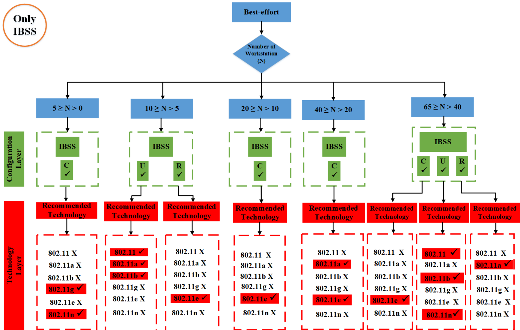
Figure 6. 9 Flowchart of only IBSS's results for Best-effort
