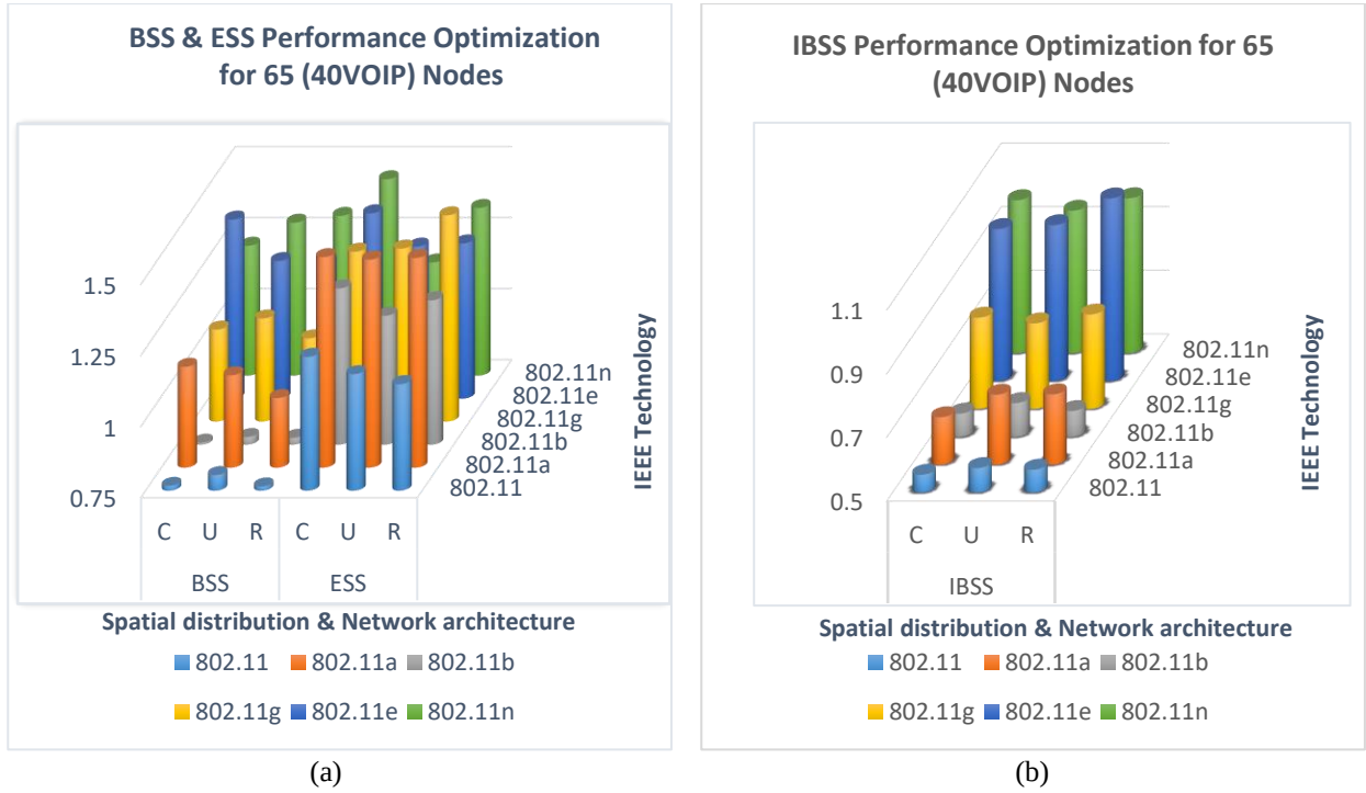
Figure 6. 32 Performance Optimization for 65 (40VOIP) nodes. (a) BSS & ESS, (b) only IBSS
