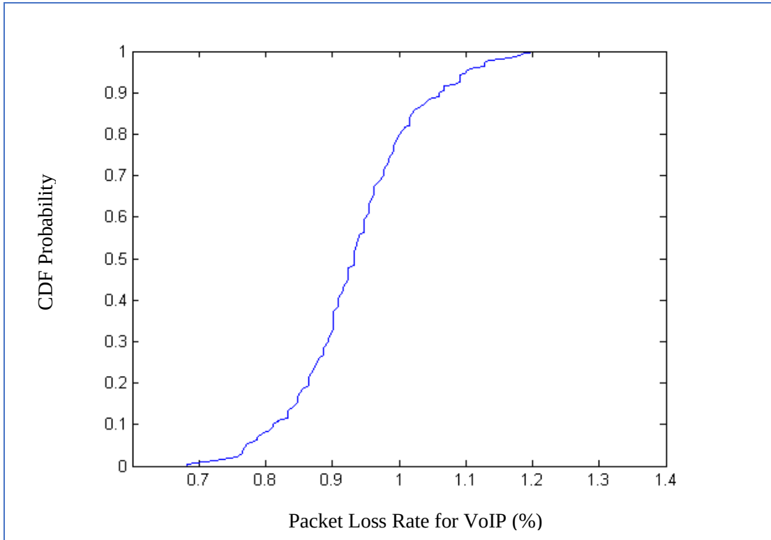
Figure 4. 8 CDF distribution of Packet loss
