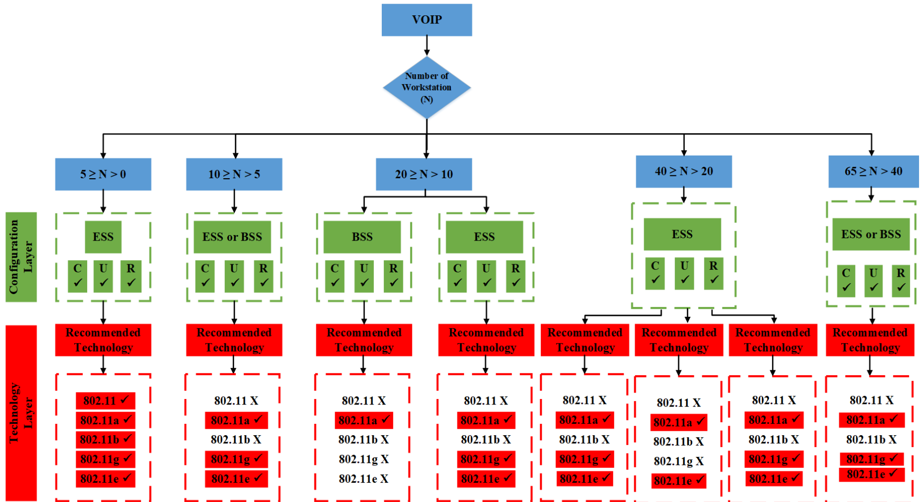
Figure 5. 1 Generic flowchart of the proposed algorithm for VoIP
