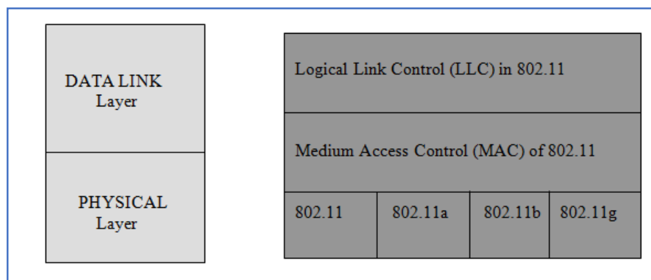
Figure 2. 1 Wireless LAN 802.11 MAC and PHY Layers (Oliveira, Rodrigues, Kozlov, Rabêlo, & Albuquerque, 2019)
