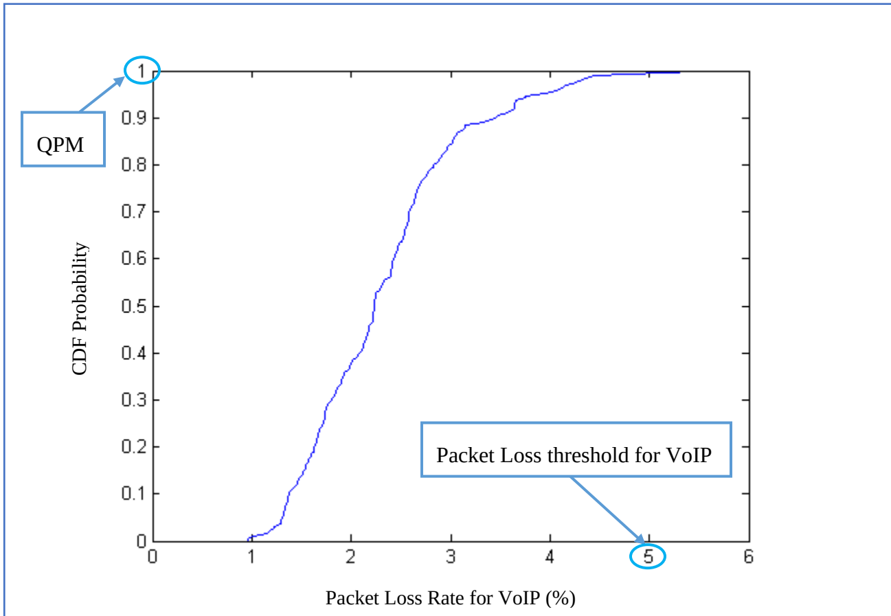
Figure 3.36 CDF distribution of Packet Loss
