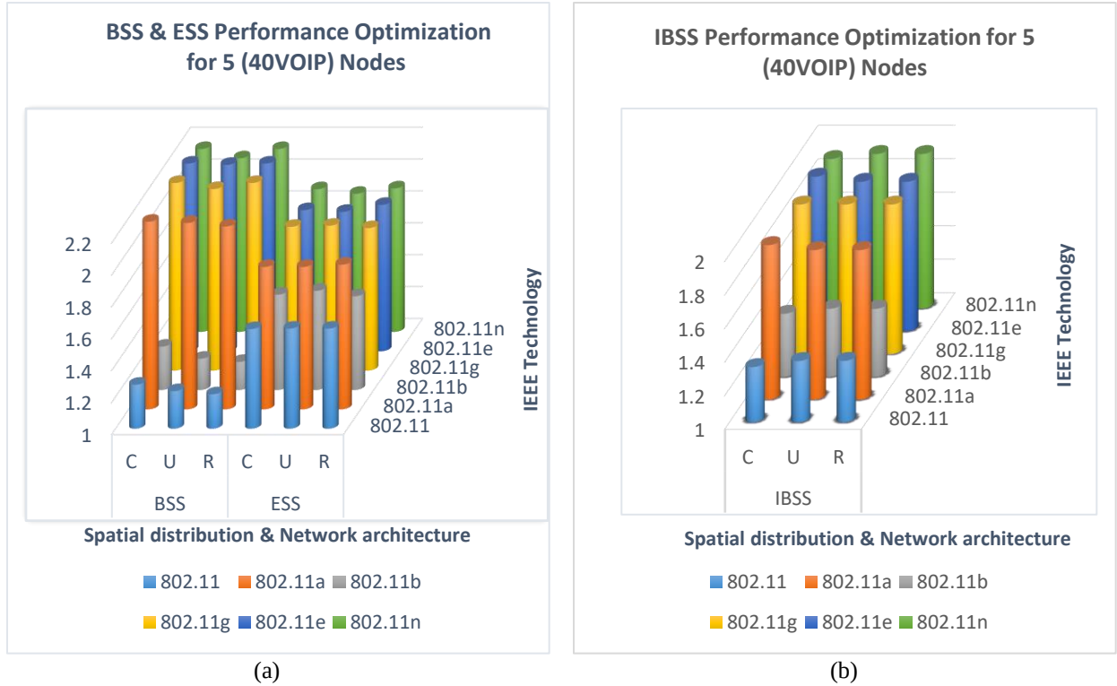
Figure 6. 29 Performance Optimization for 5 (40VOIP) nodes. (a) BSS & ESS, (b) only IBSS
