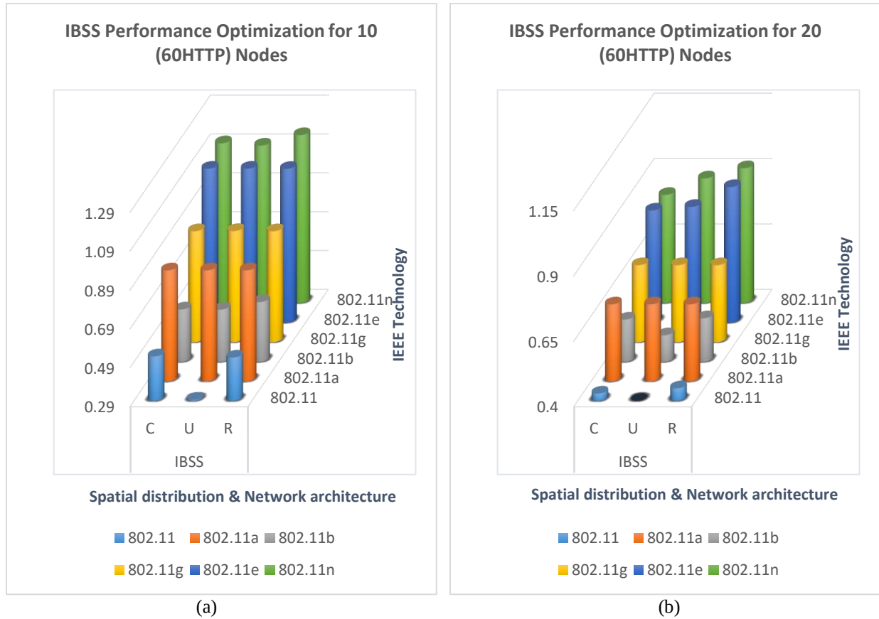
Figure 6. 26 60HTTP's IBSS Performance Optimization for various nodes. (a) 10 nodes, (b) 20 nodes
