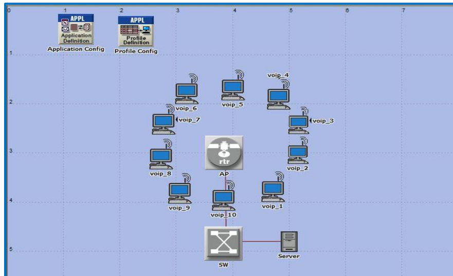
Figure 4. 1 Circular Distribution of 10 workstations and one AP
