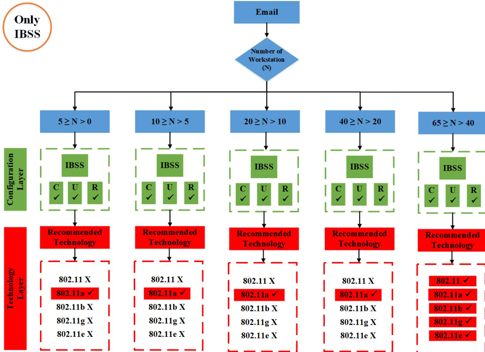
Figure 5. 10 Flowchart of only IBSS's results for Email
