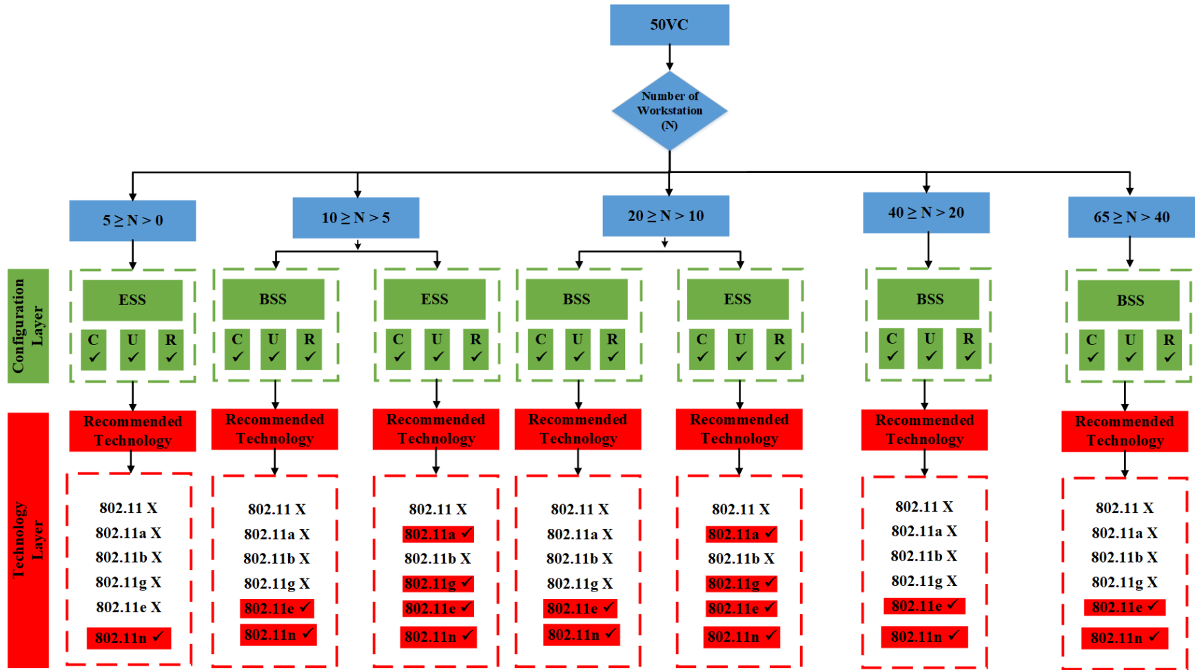
Figure 6. 1 Generic flowchart of the proposed algorithm for 50%VC
