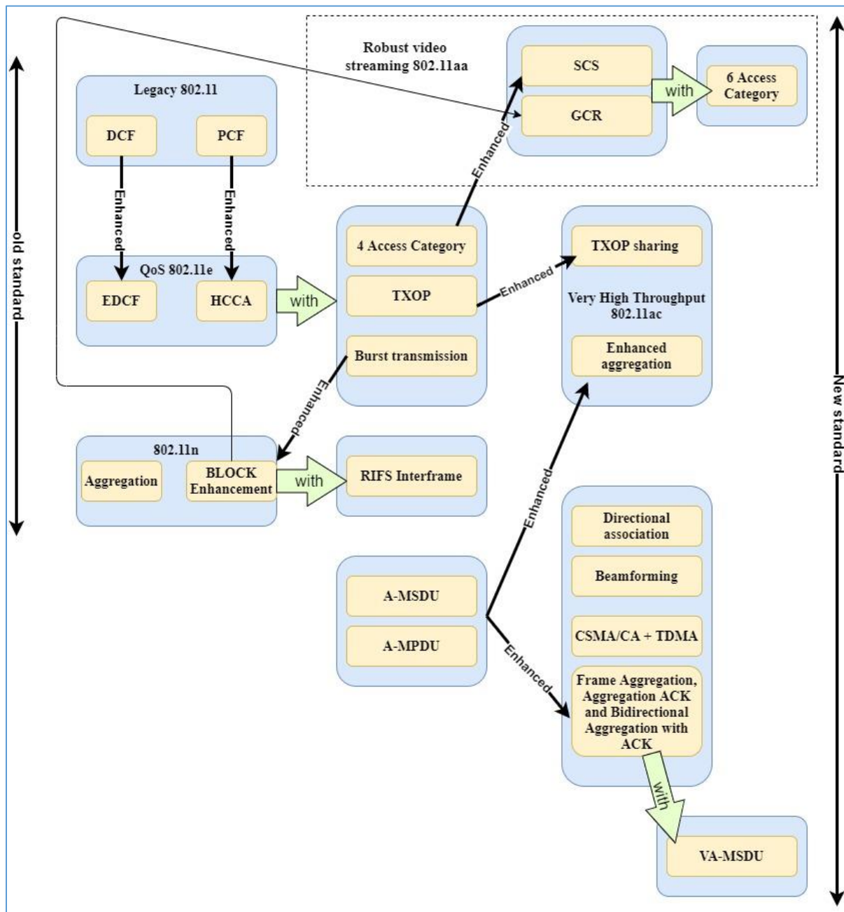
Figure 3. 3 IEEE 802.11 enhancement mechanisms (Zawia, Hassan, & Dahnil, 2018)
