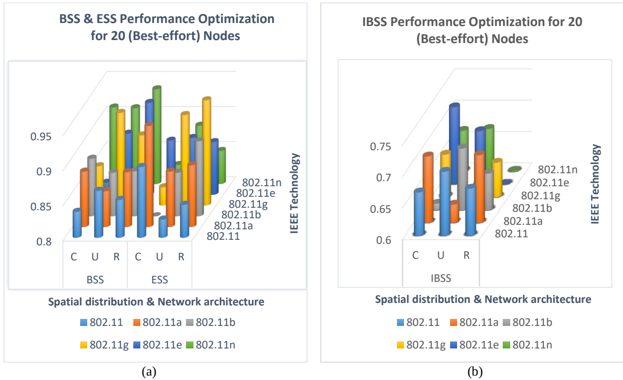
Figure 6.12 Performance Optimization for 20 (Best-effort) nodes. (a) BSS & ESS, (b) only IBSS
