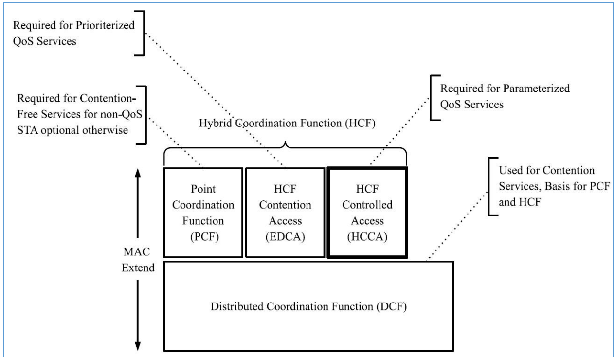
Figure 3. 4 MAC IEEE 802.11e (AL-Maqri, Alrshah, & Othman, 2018)
