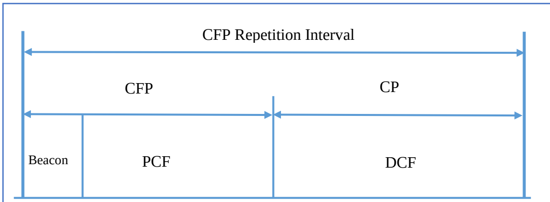
Figure 2. 9 CFP repetition interval (Refaet, Amed, Abed, & Aish, 2020)
