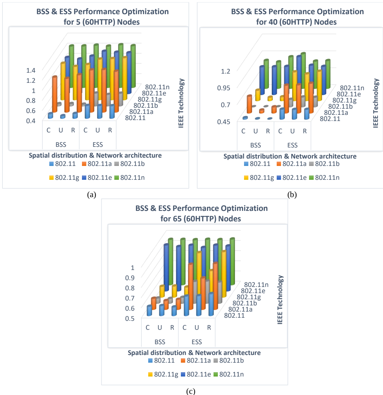
Figure 6. 23 60HTTP's BSS & ESS Performance Optimization for various nodes. (a) 5 nodes, (b) 40 nodes, (c) 65 nodes
