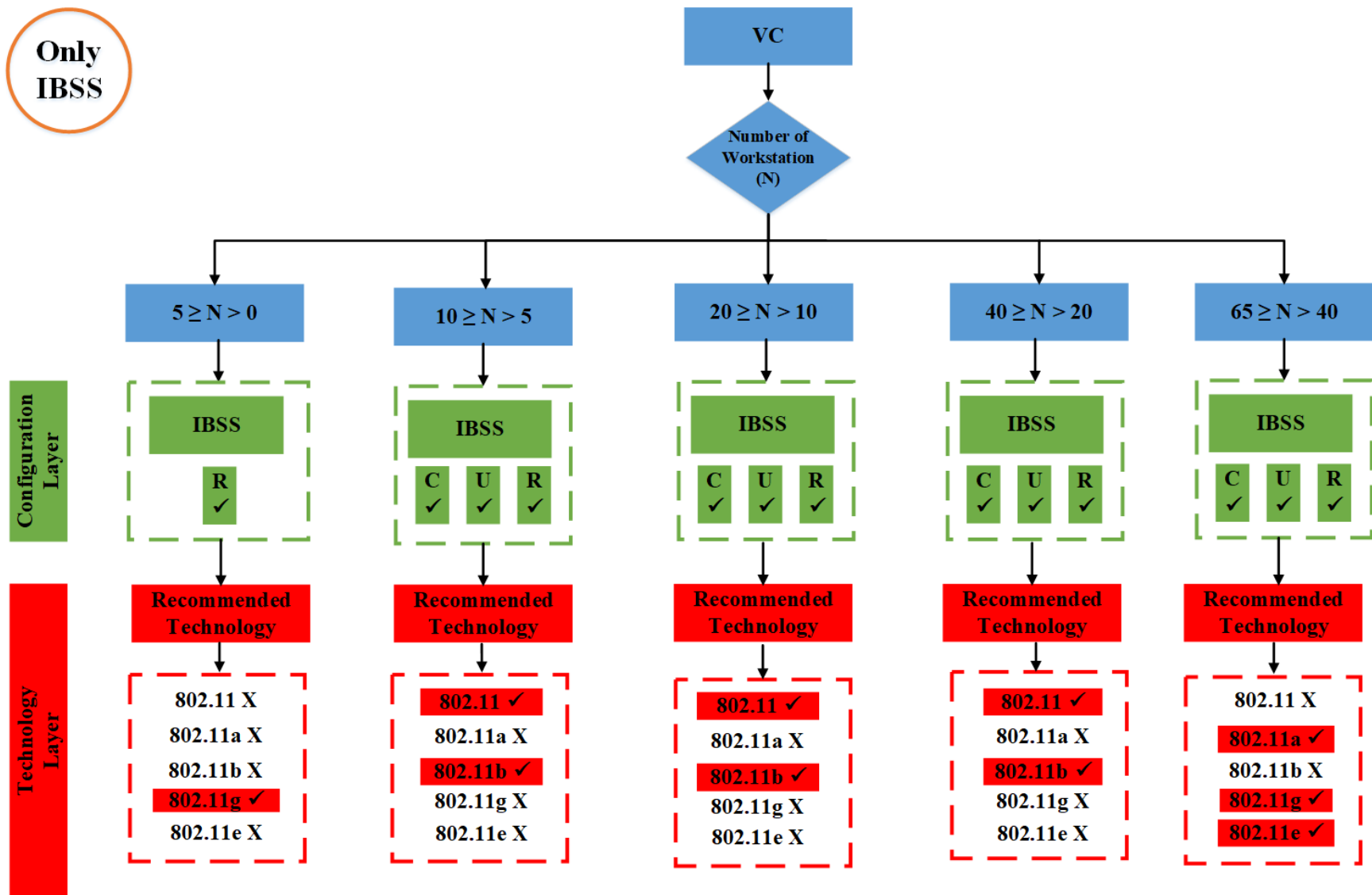
Figure 5. 4 Flowchart of only IBSS's results for VC
