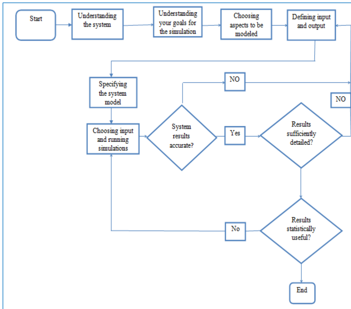
Figure 3. 5 Proposed Technique Simulation Flow Chart
