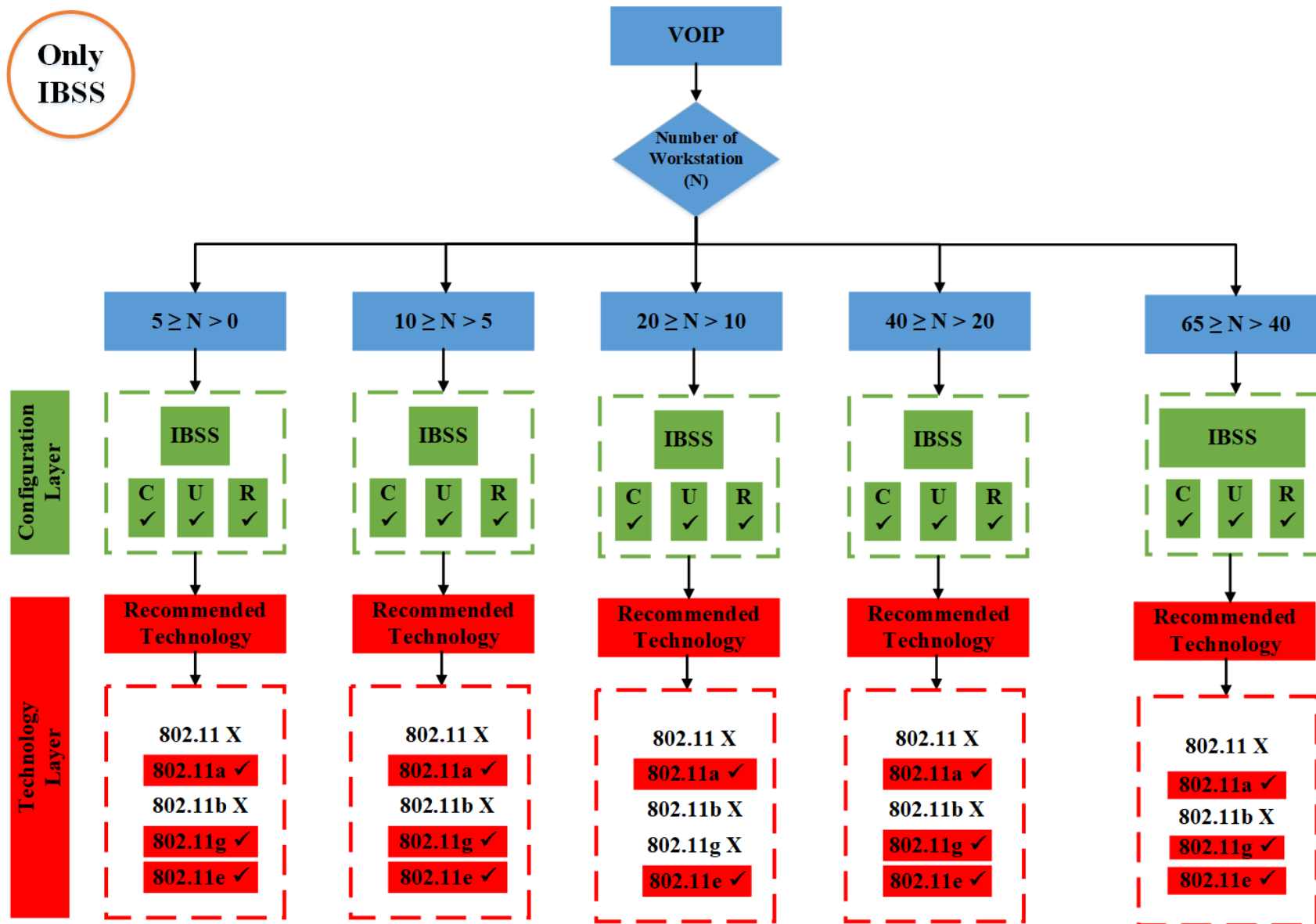
Figure 5. 2 Flowchart of only IBSS's results for VoIP
