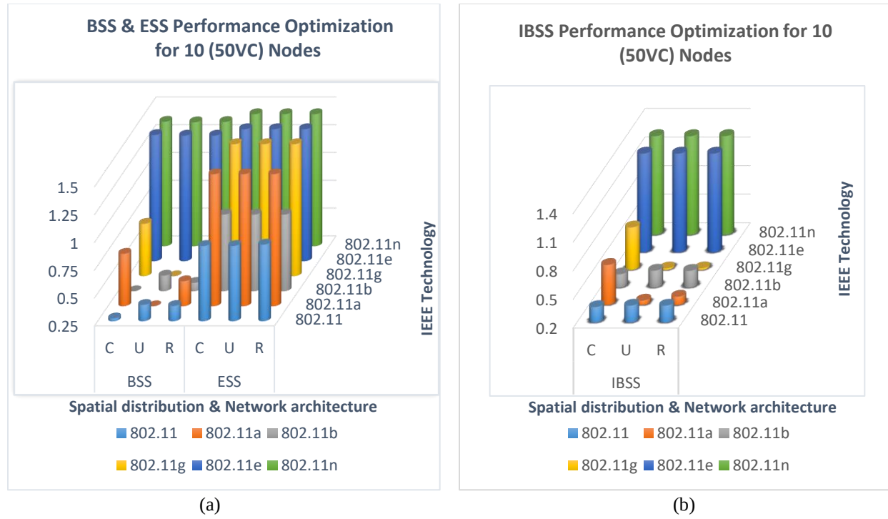
Figure 6. 4 Performance Optimization for 10 (50%VC nodes). (a) BSS & ESS, (b) only IBSS
