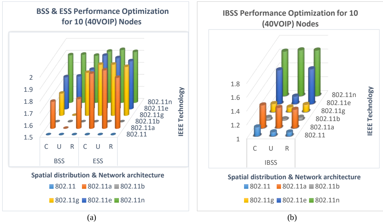
Figure 6.30 Performance Optimization for 10 (40VOIP) nodes. (a) BSS & ESS, (b) only IBSS
