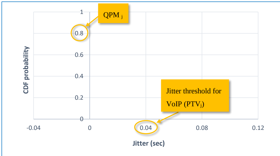
Figure 3. 35 QPM for Jitter
