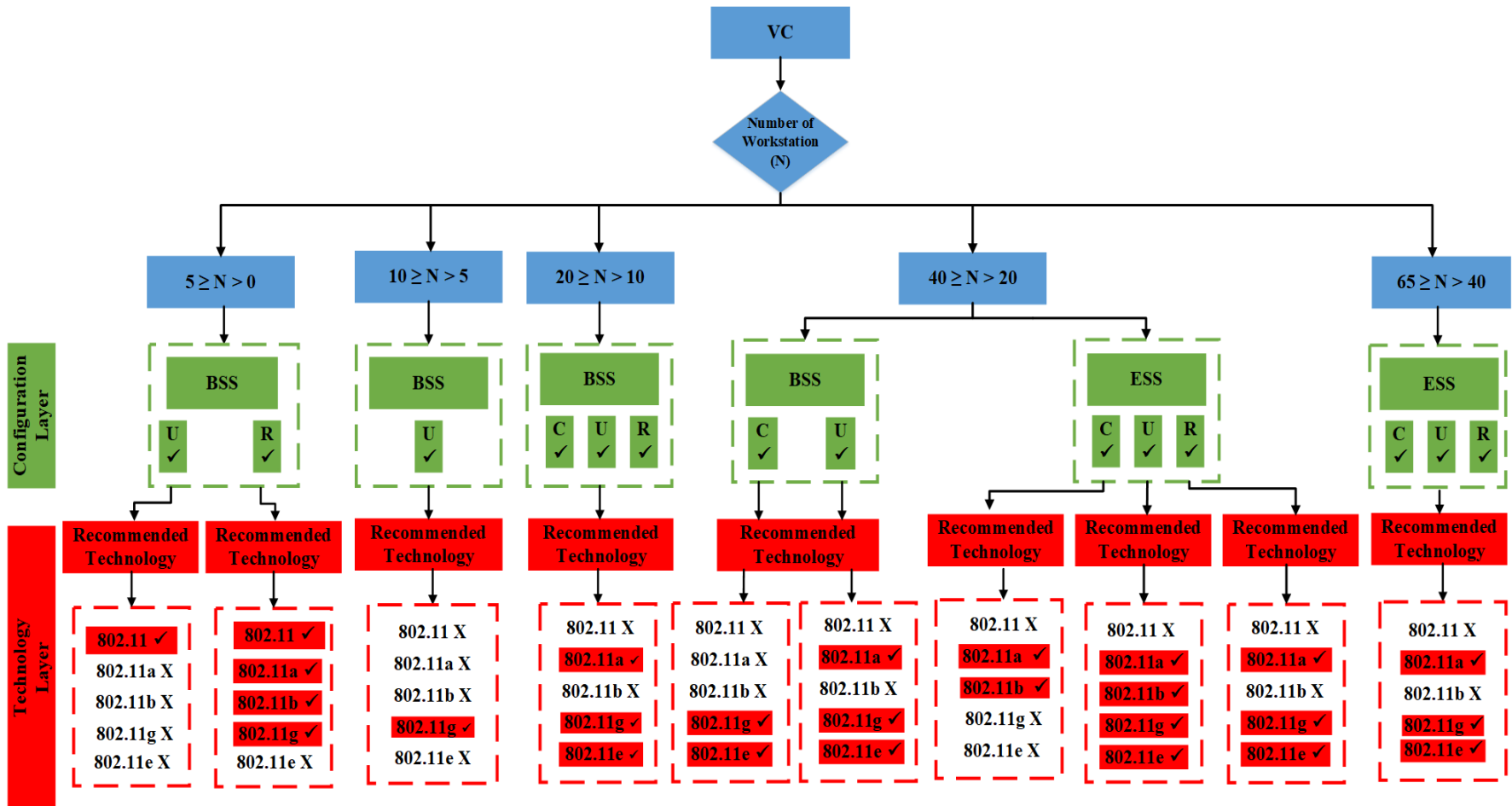
Figure 5. 3 Generic flowchart of the proposed algorithm for VC
