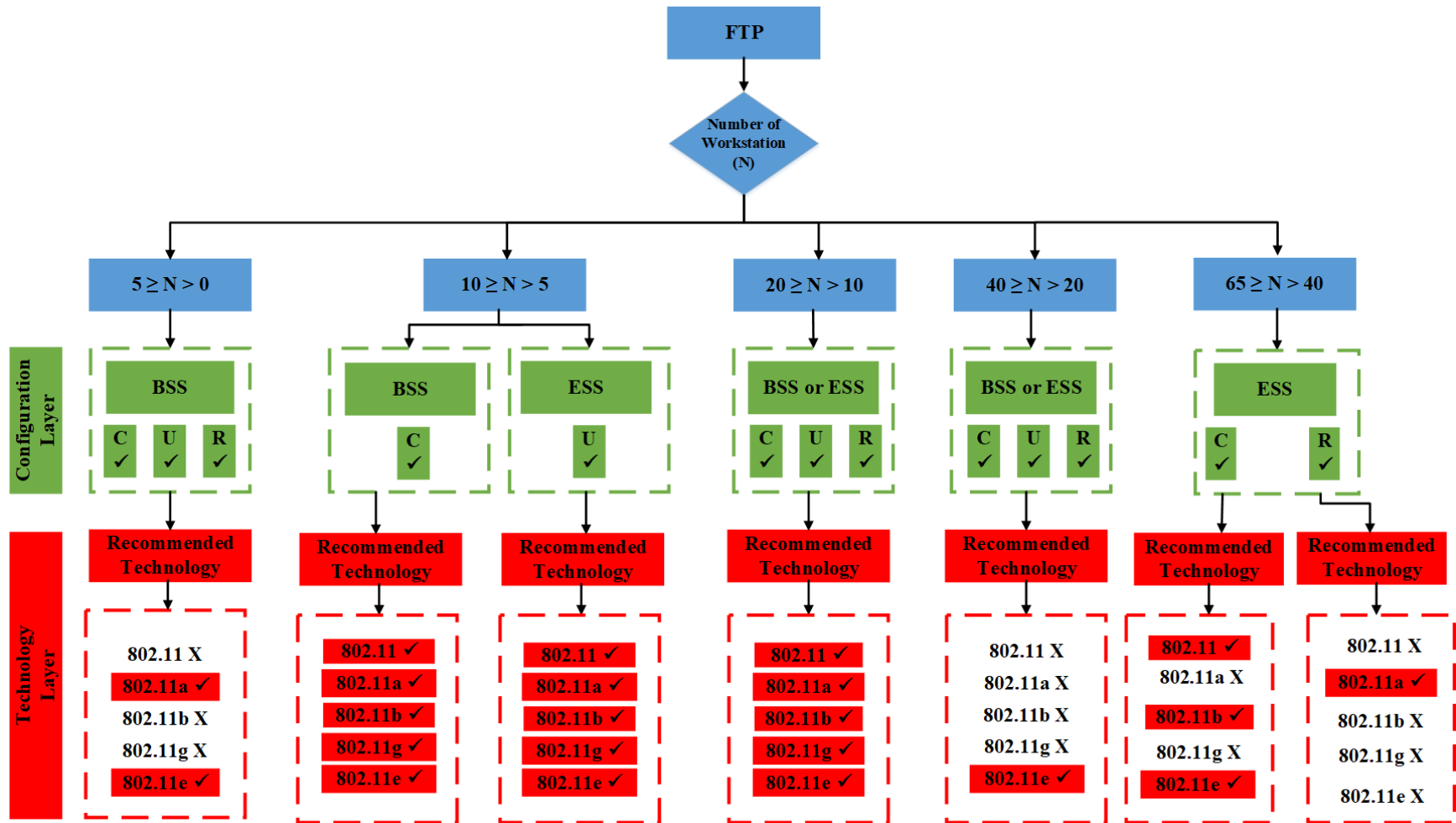
Figure 5. 7 Generic flowchart of the proposed algorithm for FTP
