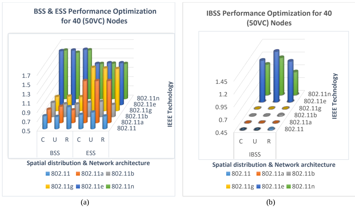
Figure 6. 6 Performance Optimization for 40 (50%VC nodes).
