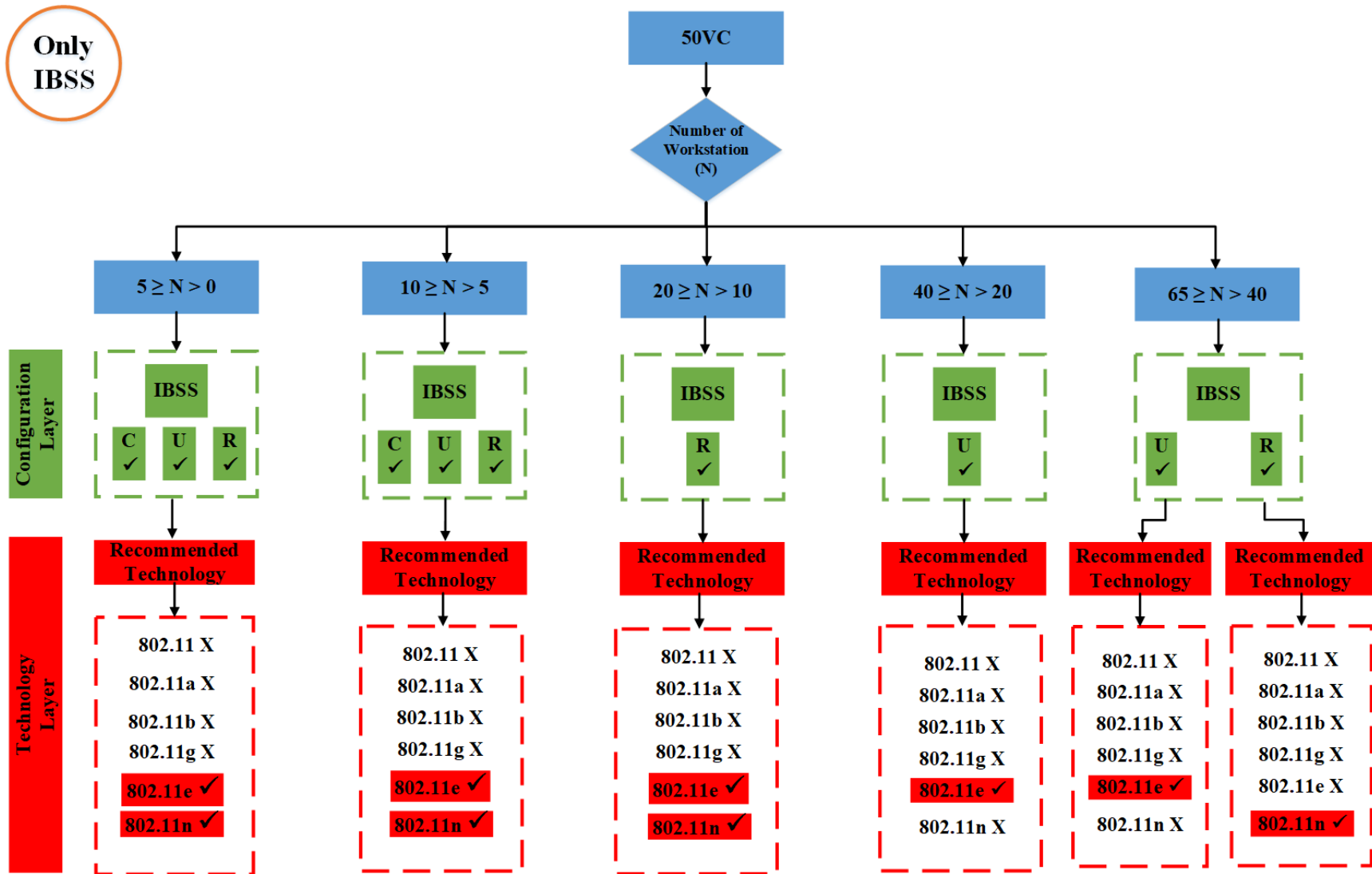
Figure 6. 2 Flowchart of only IBSS's results for 50VC
