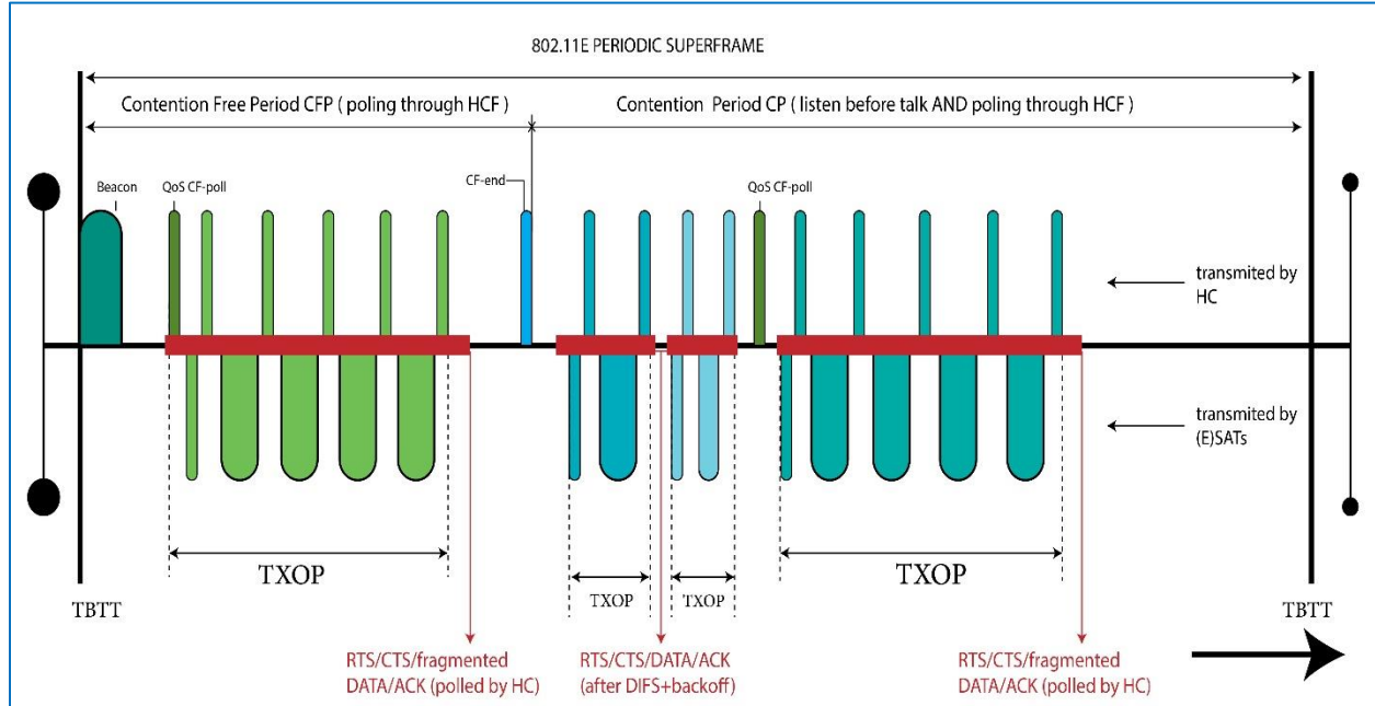
Figure 2. 11 802.11e superframe, HCF pooling (Feng, Jayasundara, Nirmalathas, & Wong, 2019)
