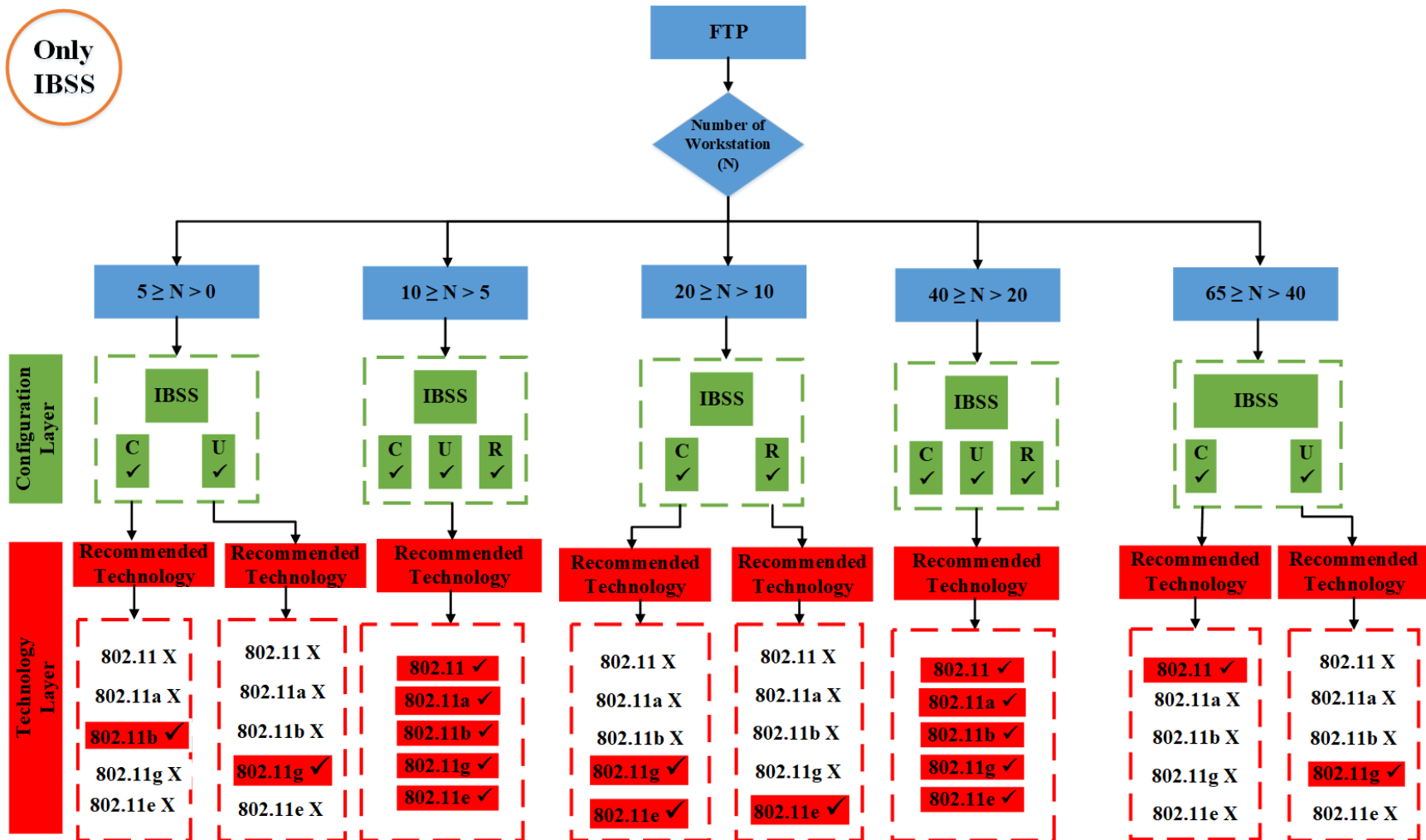
Figure 5. 8 Flowchart of only IBSS's results for FTP
