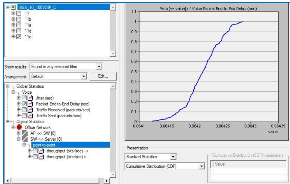
Figure 4. 3 Delay result of BSS_10_100VOIP_C
