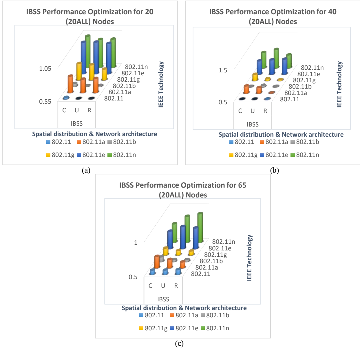
Figure 6. 20 20ALL's IBSS Performance Optimization for various nodes. (a) 20 nodes, (b) 40 nodes, (c) 65 nodes
