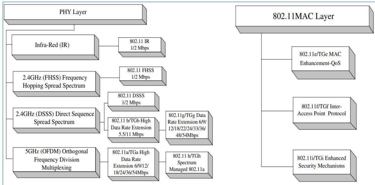
Figure 3. 2 PHY and MAC standard operations (Zawia, Hassan, & Dahnil, 2018)
