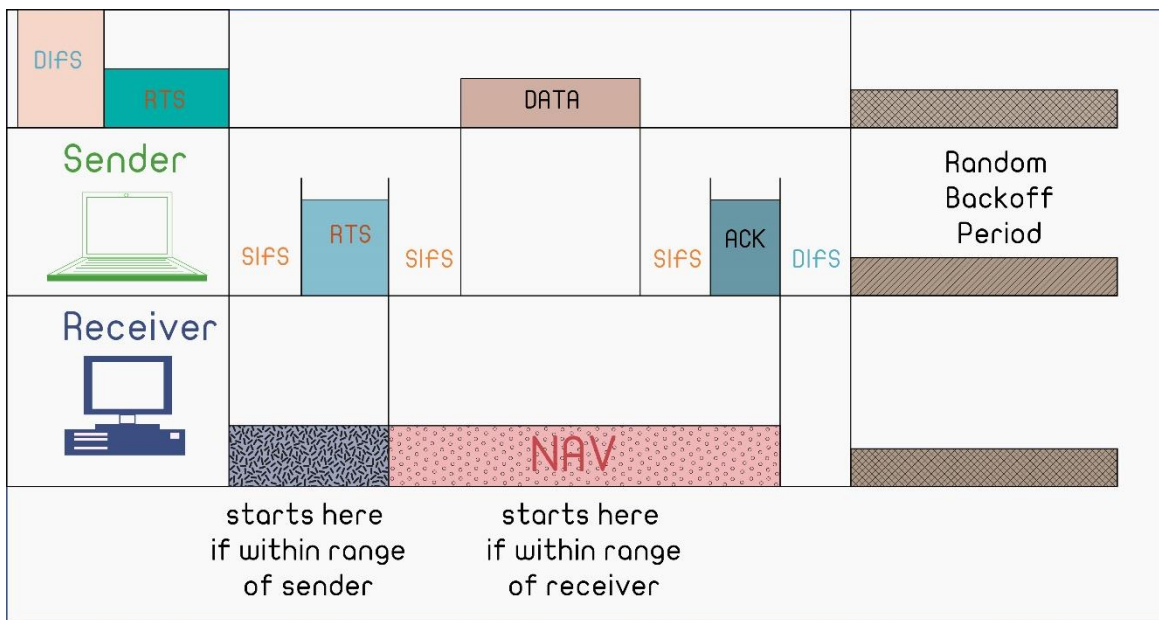
Figure 2. 6 DCF process (Coronado, Valero, Orozco-Barbosa, Cambronero, & Pelayo, 2020)
