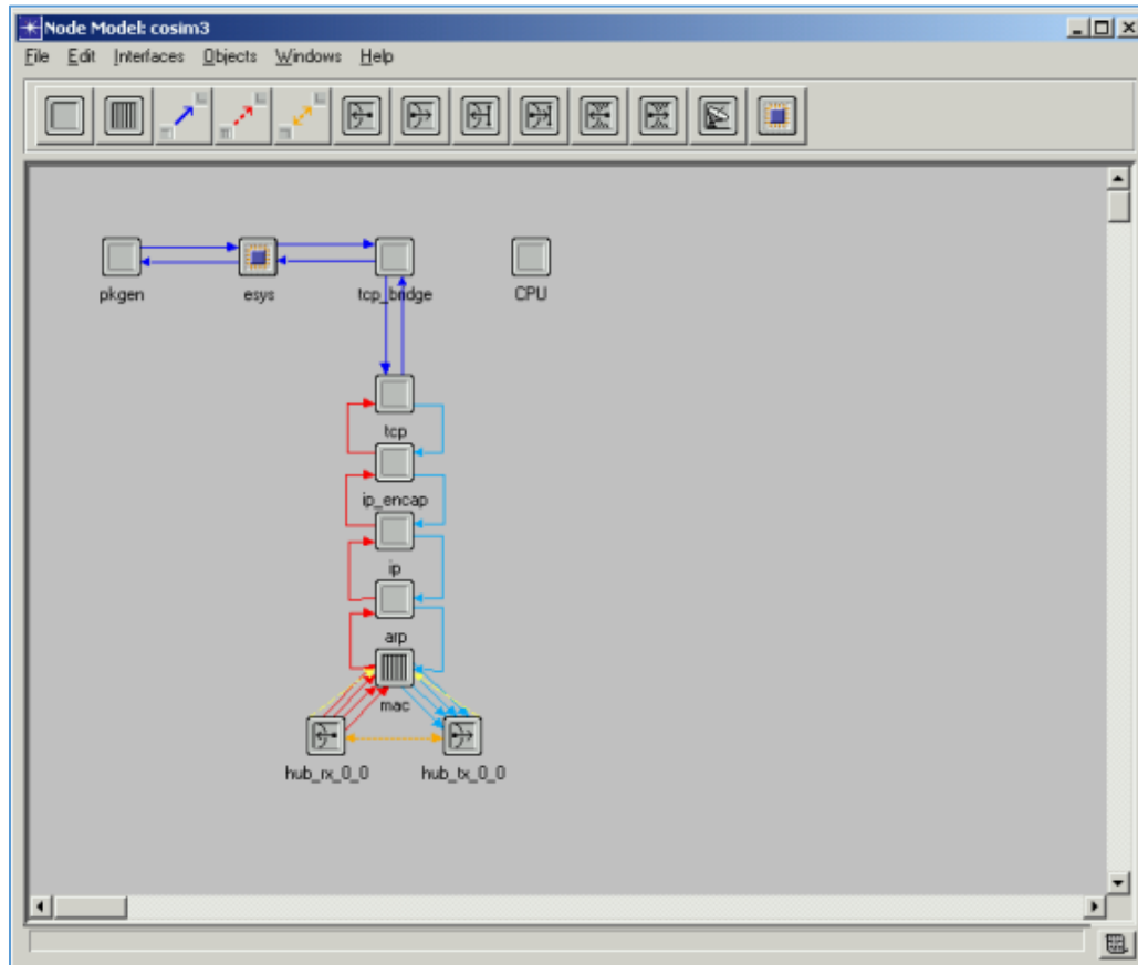
Figure 3. 7 Node Editor View (Riverbed, 2017)
