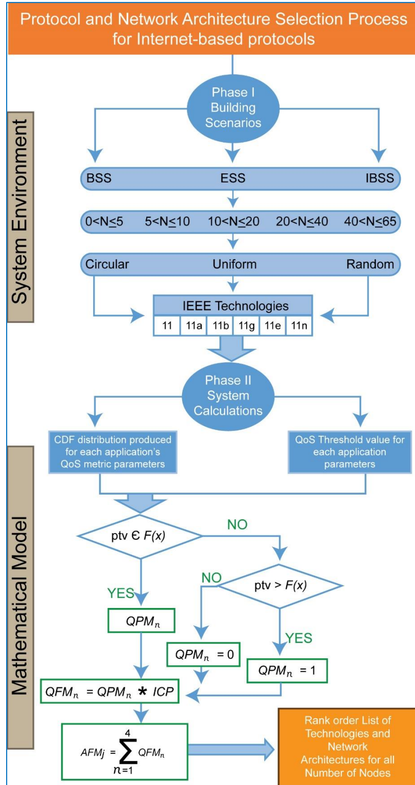
Figure 3. 34 Flow chart of Research Algorithm Process
