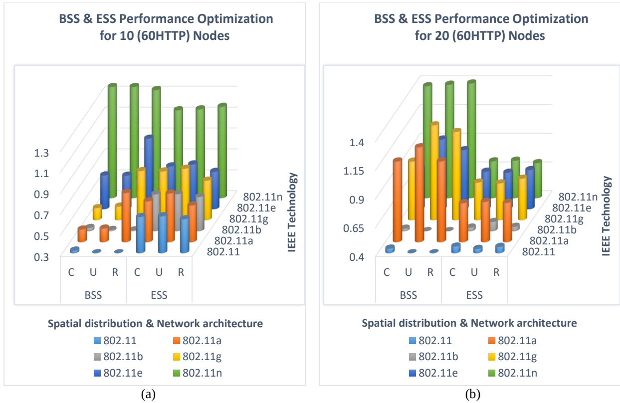
Figure 6. 25 60HTTP's BSS & ESS Performance Optimization for various nodes. (a) 10 nodes, (b) 20 nodes
