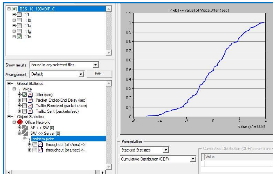
Figure 4. 2 Jitter result of BSS_10_100VOIP_C
