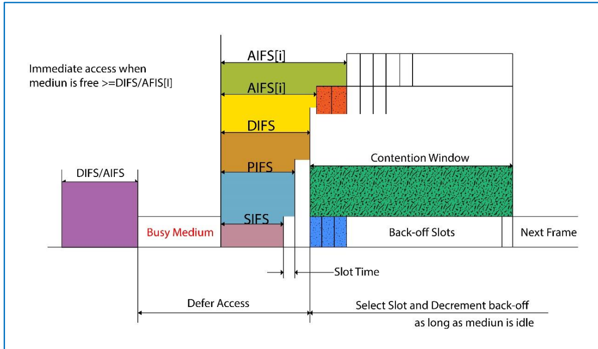
Figure 2. 10 Arbitration Inter Frame Space (AIFS) (Farej & Jasim, 2020)
