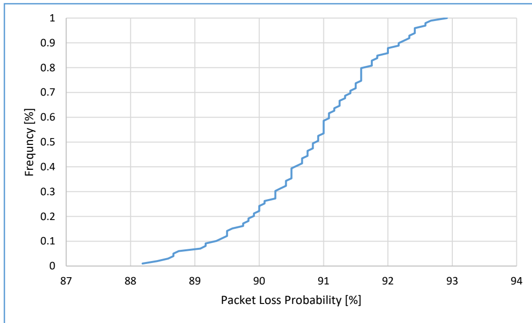
Figure 4. 13 Packet Loss result of IBSS_5_100VC_R
