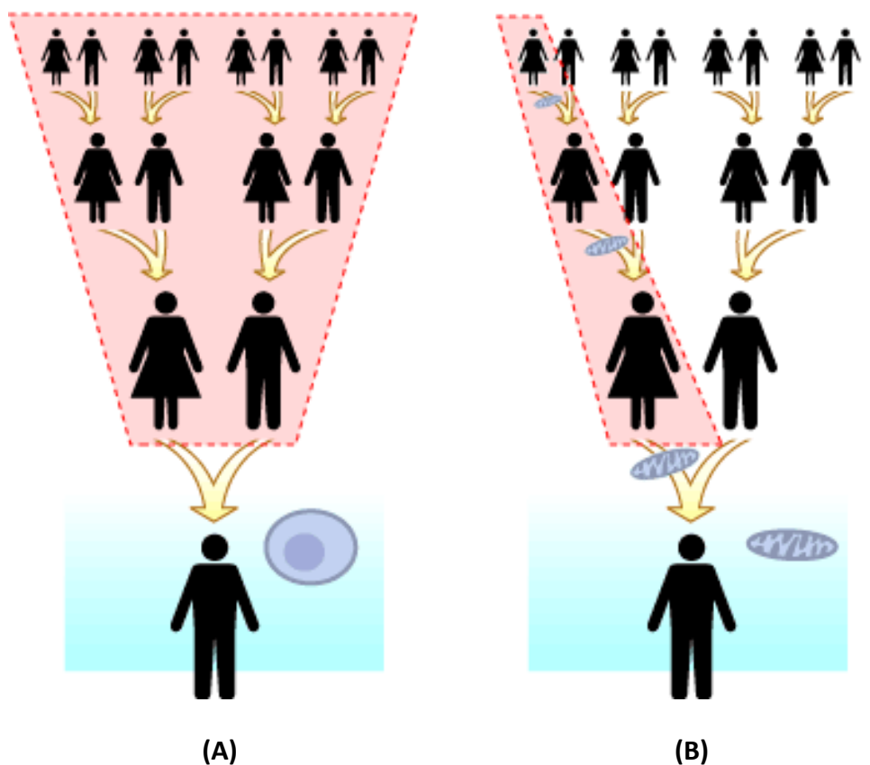
Fig 1.15: Inheritance pattern of nuclear DNA in comparison to mtDNA (University of California Museum of Paleontology's http://www.understandingscience.org ); (A) Nuclear DNA is inherited from all ancestors; one pair of chromosomes from the maternal side and one pair from the paternal side. (B) The mtDNA is only inherited from the maternal side and is an example of single lineage inheritance (Andrews et al. , 1999a,b).
