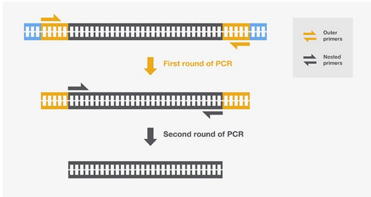
Fig. 1.23: Nested PCR (ThermoFisher Scientific). In cases where nonspecific sections are amplified due to mispriming by the outer primers, it is not very likely for the same nonspecific section to be amplified by the nested primer set, so specificity is still endorsed by the nested set of primers when recognising the intended amplicon.
