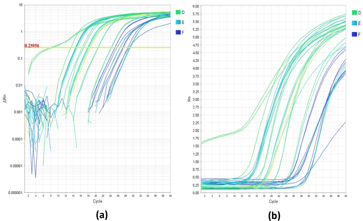
Fig.4.12: Amplification plot of samples with primer set 16S rRNA (138 bp): (a) \Delta Rn vs Cycle amplification plot of samples amplified with 16S rRNA Pig showing the cycle threshold value of 0.26 for the reaction; (b) A normalised report of Rn Vs Cycle amplification plot of samples amplified with 16S rRNA Pig. D (fl. green) - standard sample; E (light blue) - unknown sample; F (dark blue)- unknown sample and negative control (NTC).
