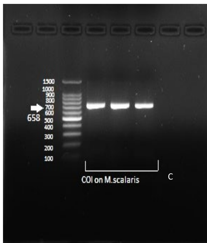
Fig 4.6: Visualisation of agarose gel electrophoresis of M. scalaris DNA with primer set COI (658 bp). 5 \mu\text{l} DNA was stained using Midori Green Advanced stain. C = DNA from gut content.
