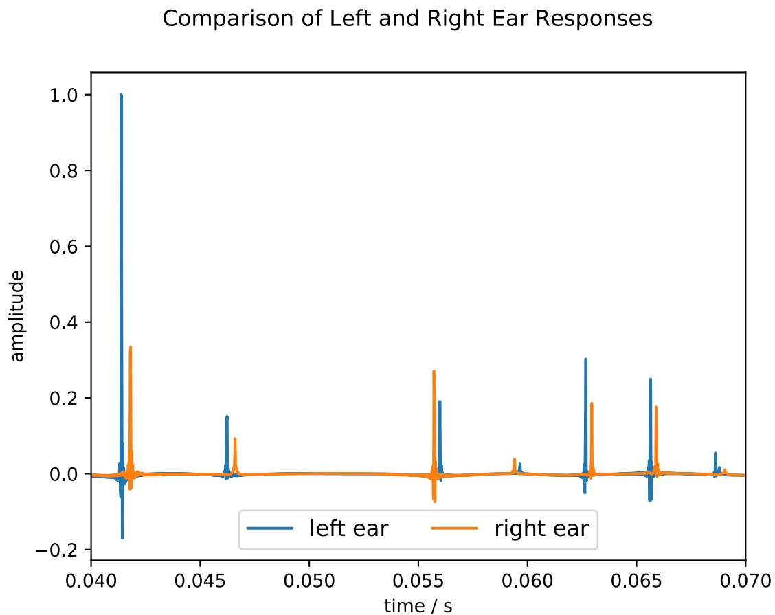
Figure 9.12: Comparison of left- and right-ear responses, when the source is placed to the left of the receiver. Note the amplitude and time differences between the early reflections. The first contribution, in particular, is quieter in the right ear because it is occluded by the listener’s virtual head.
