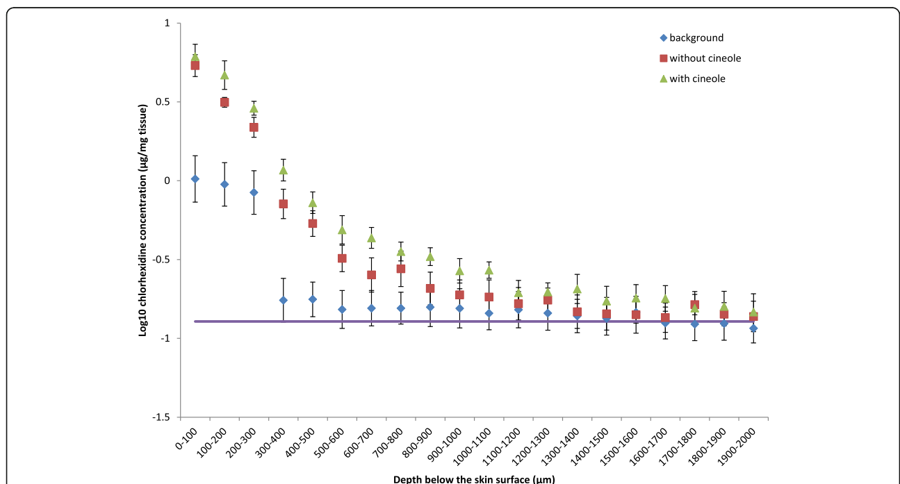
Fig. 1 Concentration of CHG in skin following exposure to 2% CHG/70% IPA with or without 2% (v/v) 1,8-cineole. Penetration profile showing the concentration of CHG in excised human skin (0-2000 µm depth) after exposure to 2% (w/v) CHG in 70% (v/v) IPA with and without 2% (v/v) 1,8-cineole (mean ± SEM). Background levels of CHG derived from preoperative skin antiseptics, without any further CHG added are also presented. The purple line represents the MIC value of CHG against MRSA (N315) in a biofilm [9]. The assumption that 1 g of skin is equal to 1 mL was made. The concentration of CHG in the skin was significantly higher in the CHG/IPA with 1,8-cineole group compared to the CHG/IPA alone ( P = 0.042 ). The size of the effect did not vary according to the depth of penetration into the skin ( P = 0.311 ), indicating that the concentration of CHG was higher at all depths with the addition of 1,8-cineole
