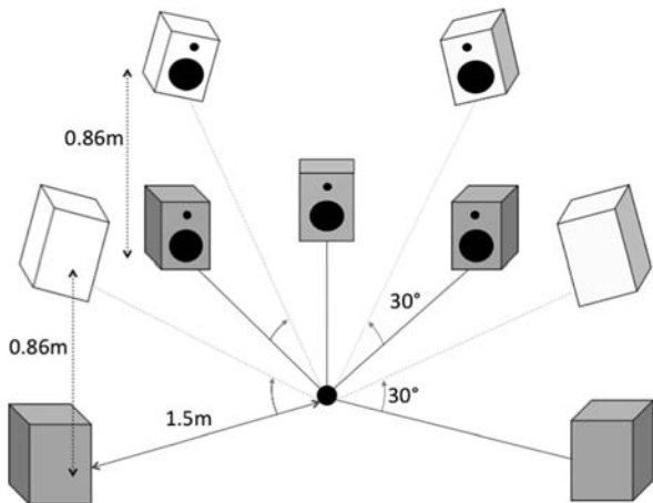
Fig. 2. Loudspeaker setup based on the 9-channel Auro-3D
