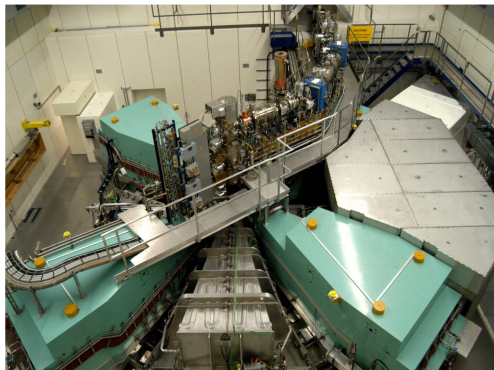
Figure 1: PSI Injector 2.
