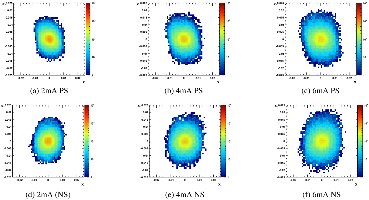
Figure 3: Spatial distribution of the bunch in the x-y plane (in meters). (a-c) shows it for production setup (PS) and (d-f) for future set up for 2, 4 and 6mA beam currents.
