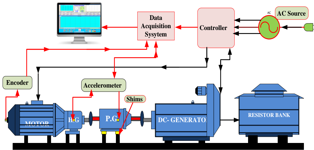
Figure 2. Schematic diagram of planetary gearbox test facility
