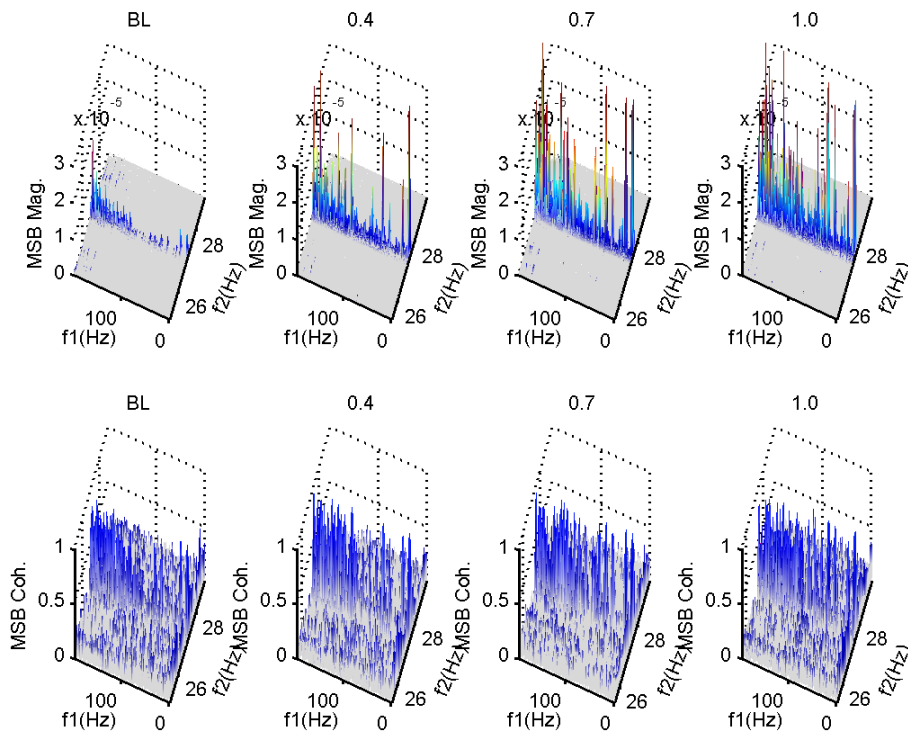
Figure 5 MSB results for different cases at lower speed and high loads
