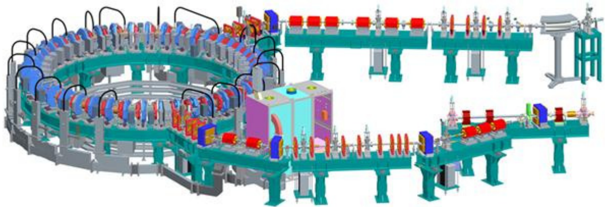
Figure 1: The layout of EMMA. Shown is a short section of the ALICE machine, with a new dipole magnet to steer the beam into the injection line (bottom of the picture). The EMMA ring, showing the 42 cells, is on the left and the diagnostics beam line at the top.
