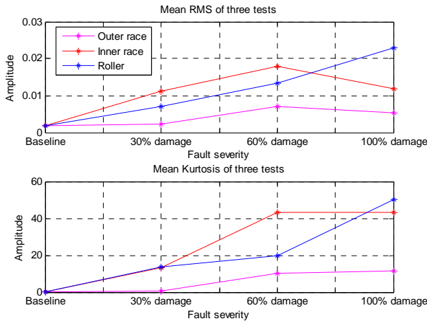
Figure 11. Mean RMS and Kurtosis comparison results
