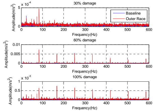
Figure 8. Envelope analysis results for outer race defect
