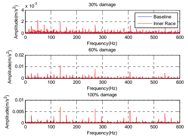
Figure 9. Envelope analysis results for inner race defect
