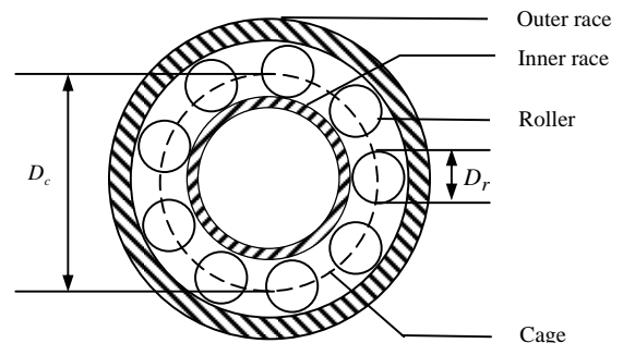
Figure 1. Rolling element bearing components
