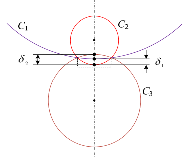
Figure 3. Geometry deformation for two kinds of contact
