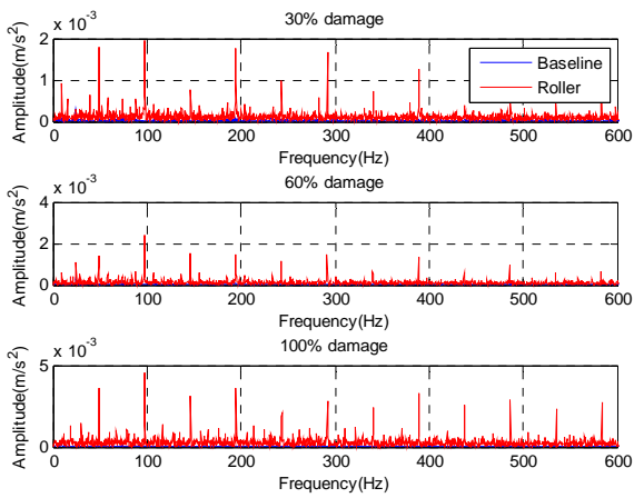
Figure 10. Envelope analysis results for roller defect
