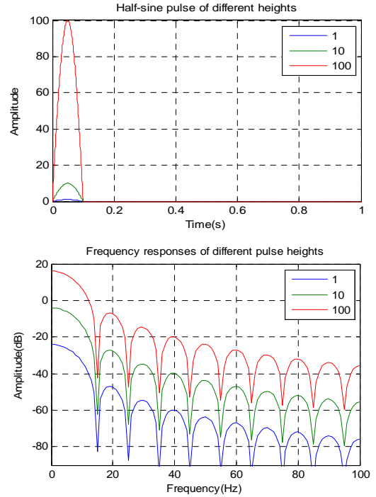
Figure 4. Frequency responses of difference pulse heights
