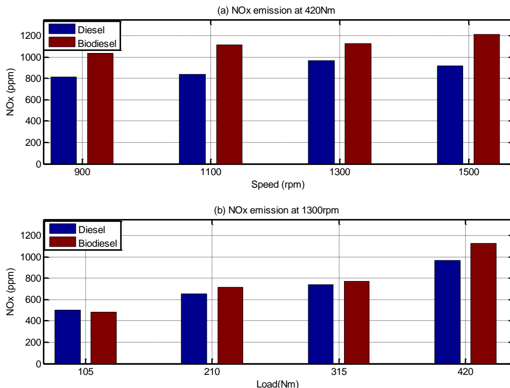
Figure 3 Comparison of diesel and biodiesel NO x emission (a) at 420 Nm range of speeds (b) at 1300rpm range of loads
