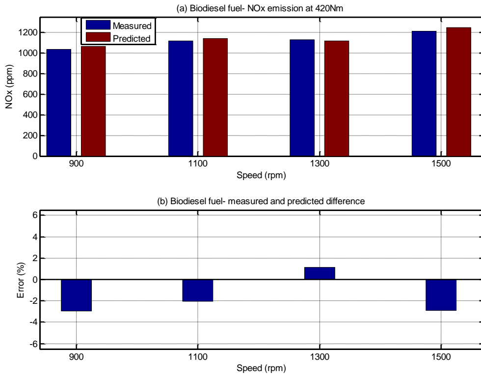
Figure 5 CI engine running with biodiesel at 420Nm (a) Measured and predicted NOx emission values (b) The % error between measured and predicted values
