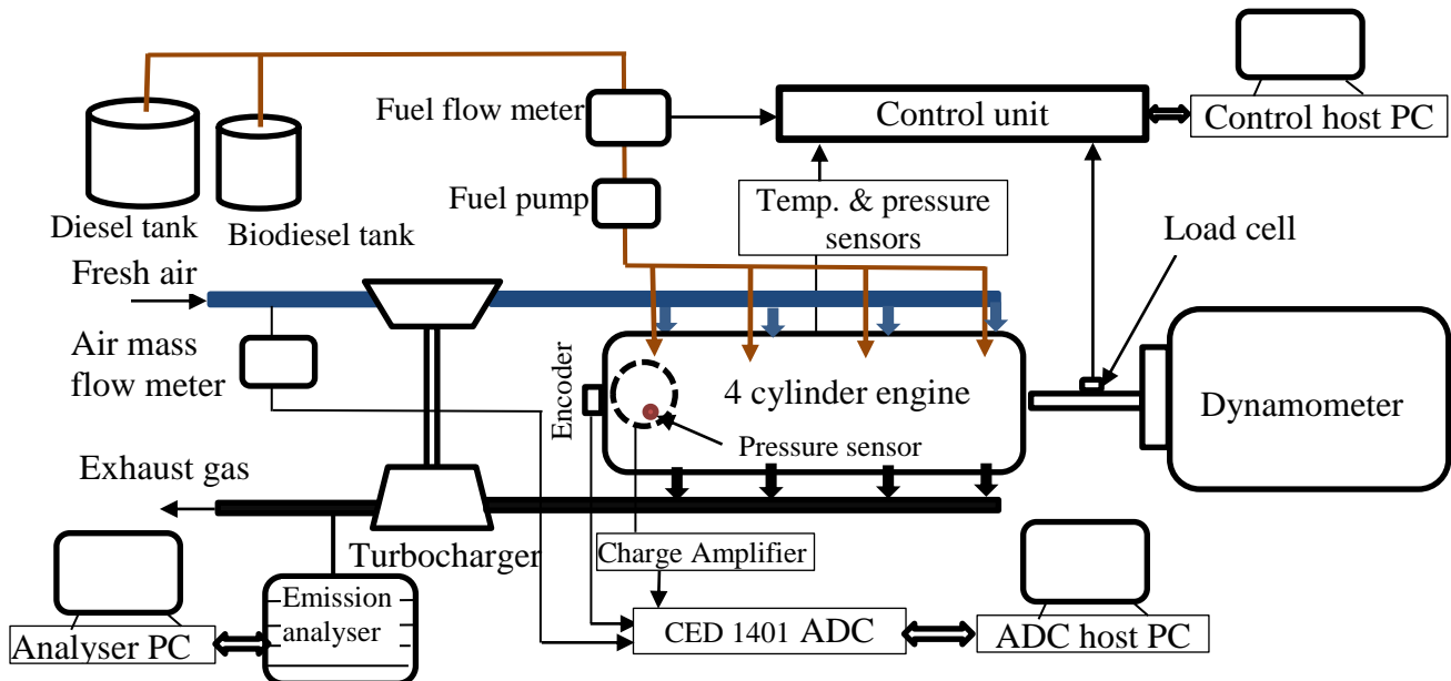
Figure 1 Experimental setup [19]
