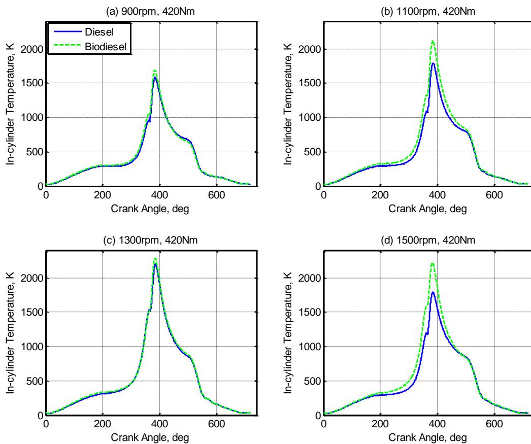
Figure 2 In-cylinder temperatures versus crank angle of CI engine running with diesel and biodiesel for engine loads of 420Nm and range of speeds
