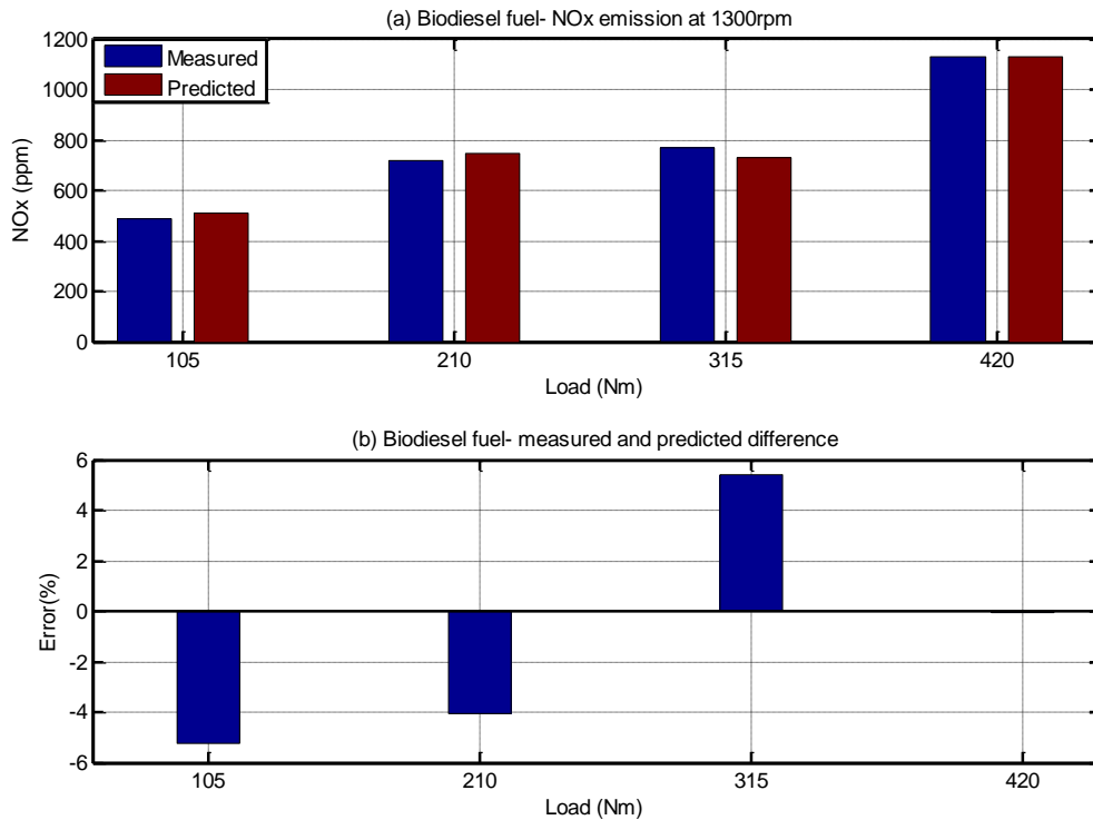
Figure 7 CI engine running with biodiesel at 1300rpm (a) Measured and predicted NOx emission values (b) The measured and predicted % error
