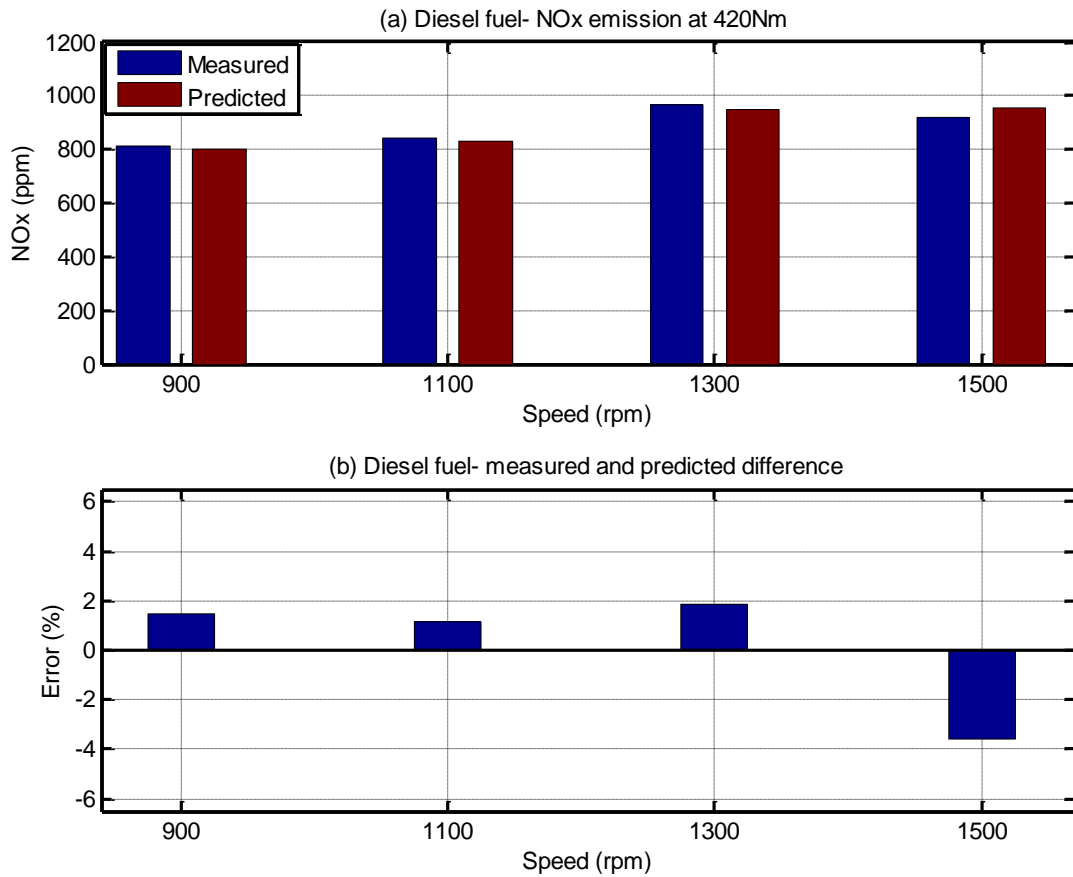
Figure 4 CI engine running with diesel at 420Nm (a) Measured and predicted NO x emission values (b) The % error between measured and predicted values
