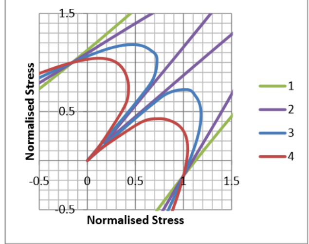
Figure 1. Isochronous rupture loci for KRH formulation (top for plane stress condition and bottom for plane strain condition for v = 0, 1, 2, 3, \text{ and } 4 ). The legends are for stress state index v .
