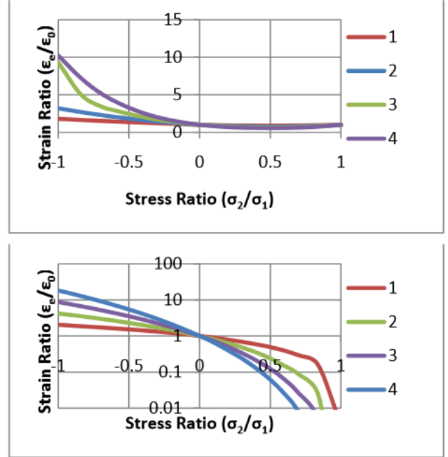
Figure 2. Ratios of strain at failure for KRH formulation (top for plane stress condition and bottom for plane strain condition for v = 0, 1, 2, 3, \text{ and } 4 ). The legends are for stress state index v .
