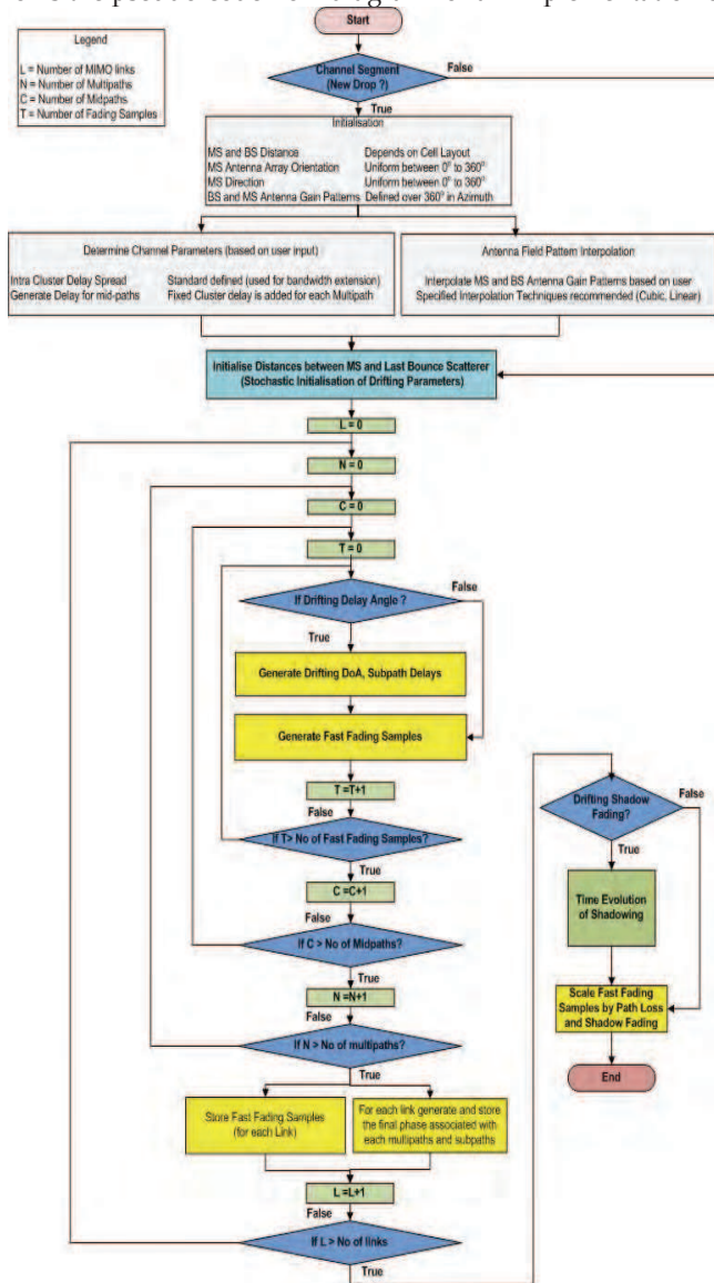
Fig. 12. Pseudo-code flow diagram of SCME channel model.
