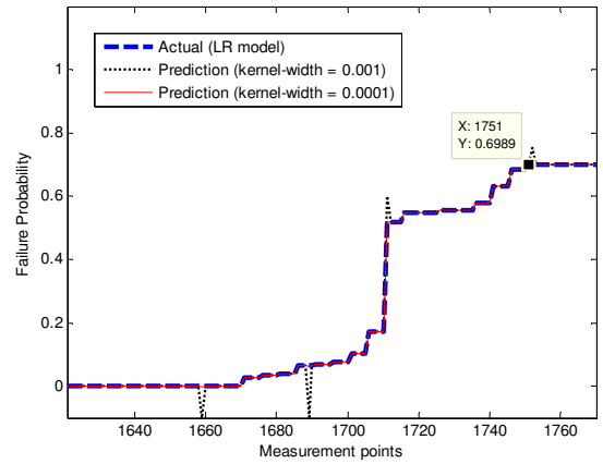
Fig. 12 The result of degradation prediction
