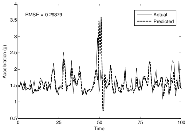
Fig. 8 Predicted results of ANFIS.
