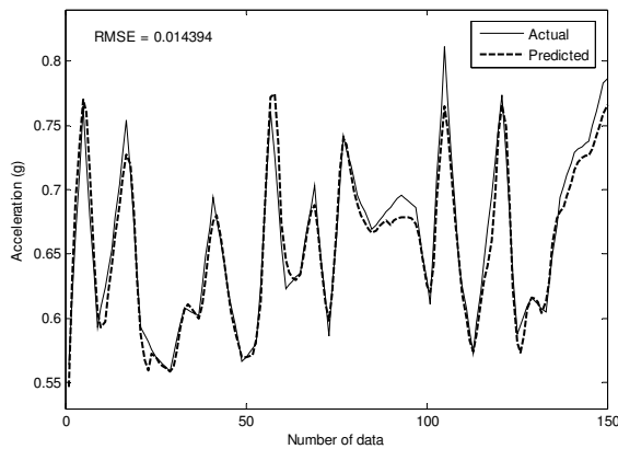
Fig. 4 Predicted results of envelope acceleration data
