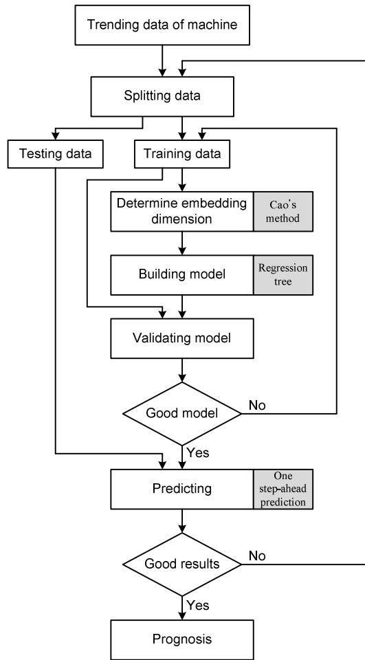
Fig. 3 The prognostic method by DT
