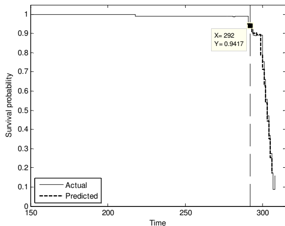
Fig. 15 Predicted results of RUL
