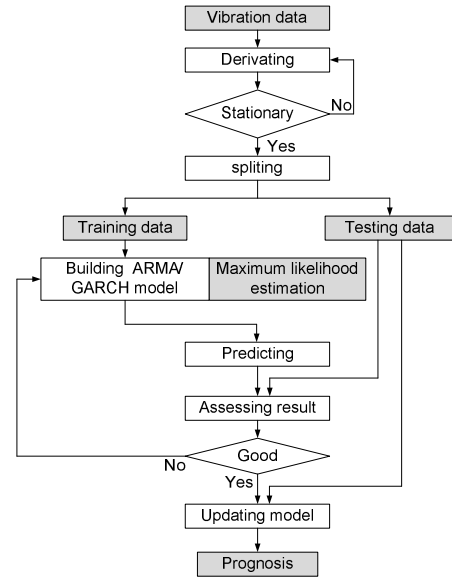
Fig. 9 The ARMA/GARCH prediction model
