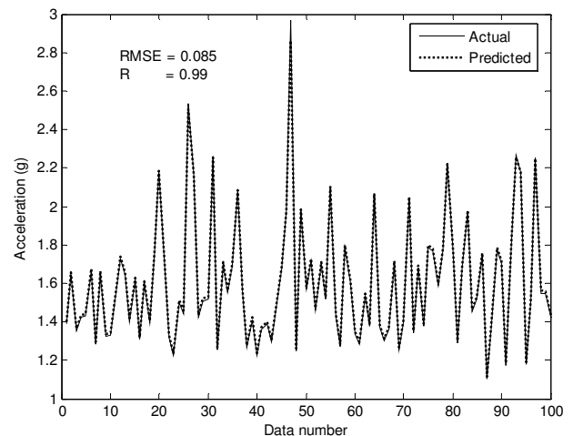
Fig. 2 Prediction of envelope acceleration data
