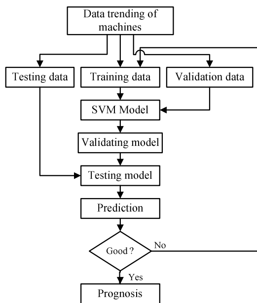
Fig. 1 SVM for prognostics implementation
