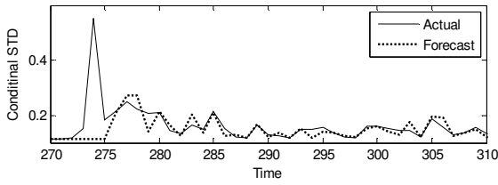
(d) Fig. 10 The conditional standard deviation forecasts of innovations (a ~ d): using 1 ~ 4 step-ahead prediction
