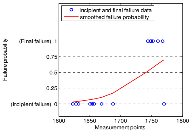
Fig. 11 Logistic regression of data
