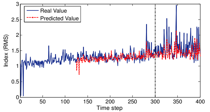
Fig. 5 Prediction of acceleration trend by DSR
