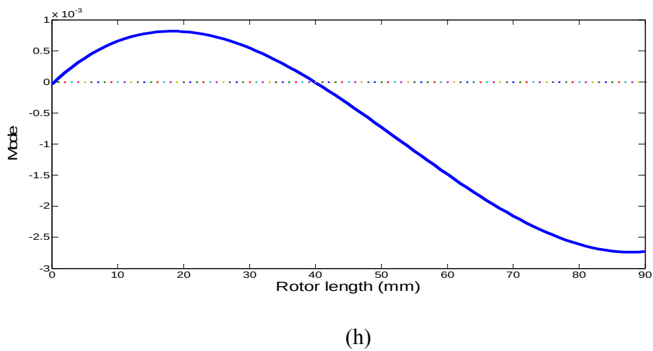
Figure 5. 4. Turbocharger mode shapes with an equivalent bearing stiffness coefficient of 10^{10} N/m at the rotational speed of 8,000 rad/s
