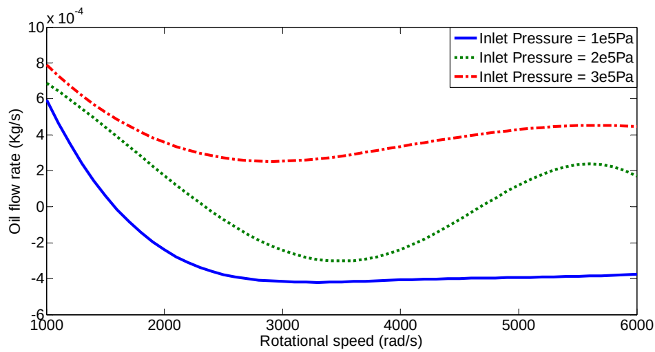
Figure 3. 15. The mean oil flow rate into the inner oil film under
