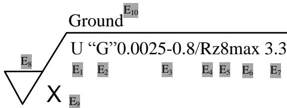
Fig. 2. Control elements in indication of surface texture requirements on engineering drawings
