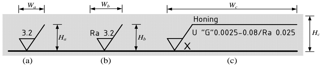
Fig. 1. Different versions of the surface texture symbols in technical drawing. (a) the 1971 version, (b) the 1992 version, (c) the 2002 version.
