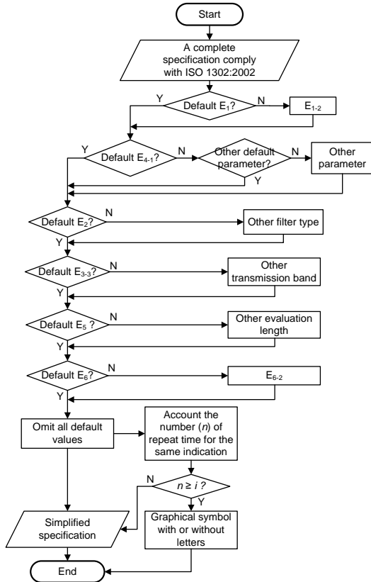
Fig. 3. Flow chart of the simplified procedure for
