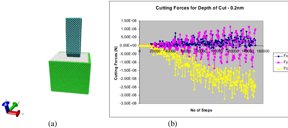
Figure 1: Rubbing Phenomenon
