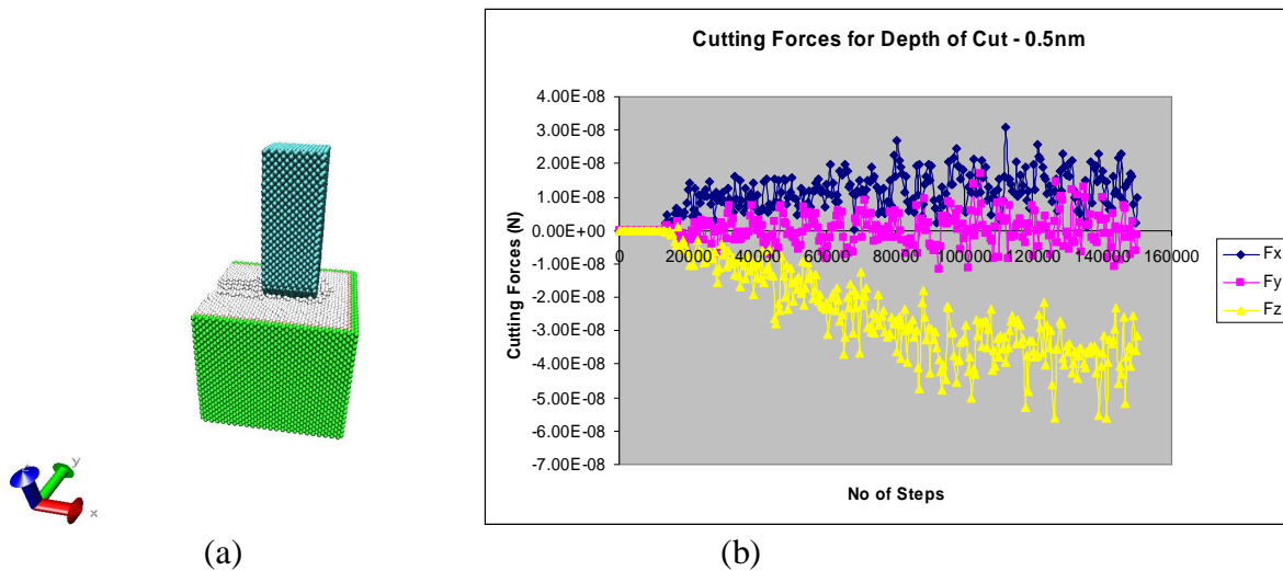
Figure 2: Ploughing Phenomenon
