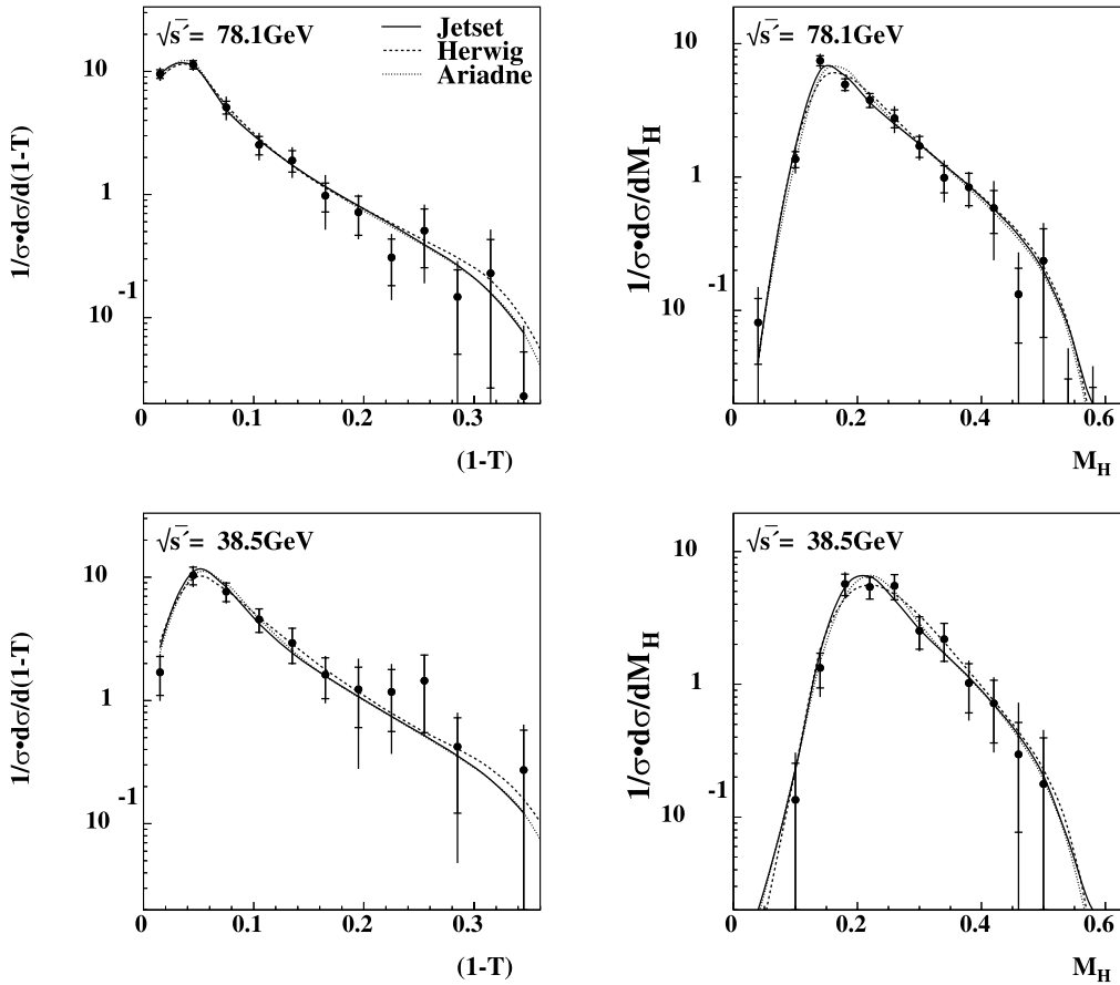
Fig. 5. Event shape distributions at the hadron level. The error bars correspond to the statistical and experimental uncertainties described in Sect. 6.1.1. Two of the six event shape observables, 1-T and M_H , are shown for the low (38.5 GeV) and high (78.1 GeV) \sqrt{s'} samples. The small lines on the error bars show the extent of the statistical uncertainty. The data points are placed at the centres of the corresponding bins. The predictions of JETSET, HERWIG and ARIADNE at the corresponding \sqrt{s'} values are also shown as lines
