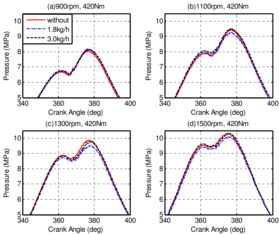
Figure 5 Cylinder pressure at 420Nm and at different engine speeds
