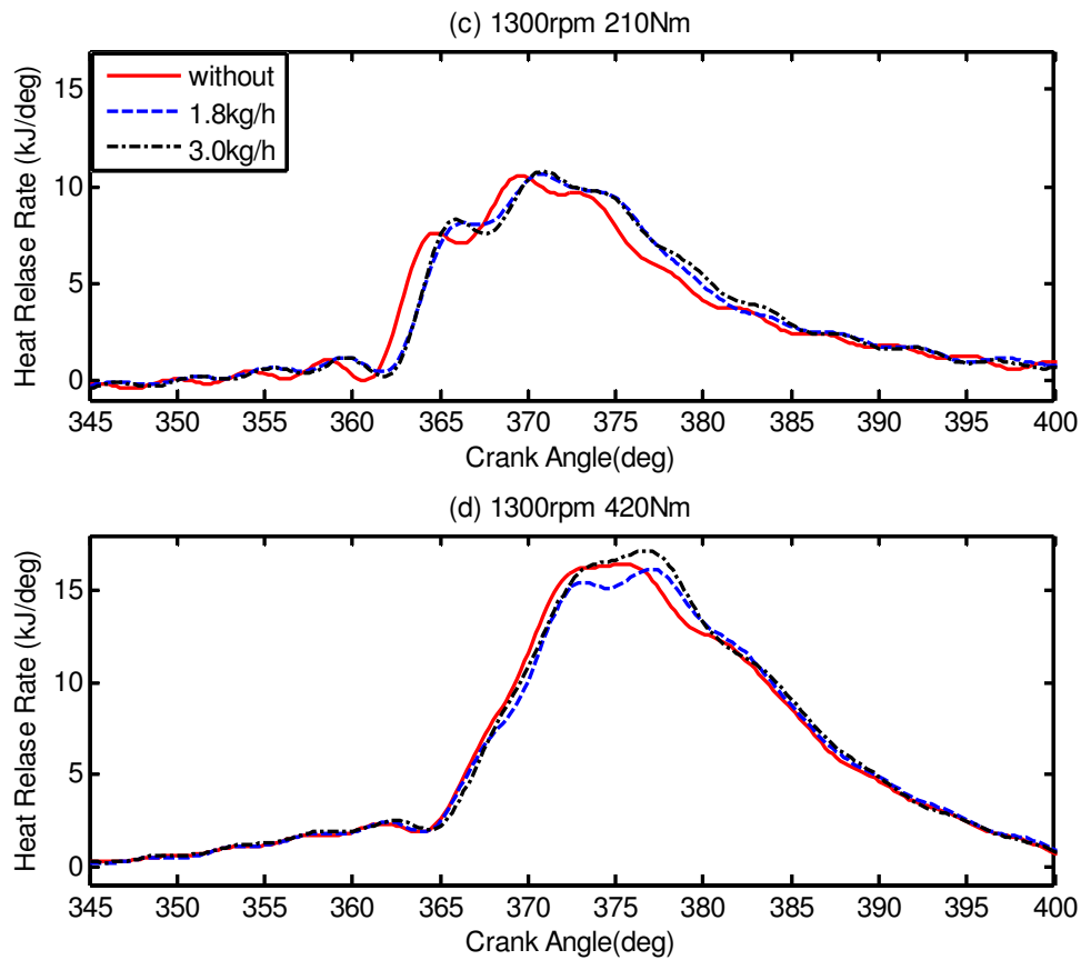
Figure 6 Heat releases rate at 1300rpm and different loads
