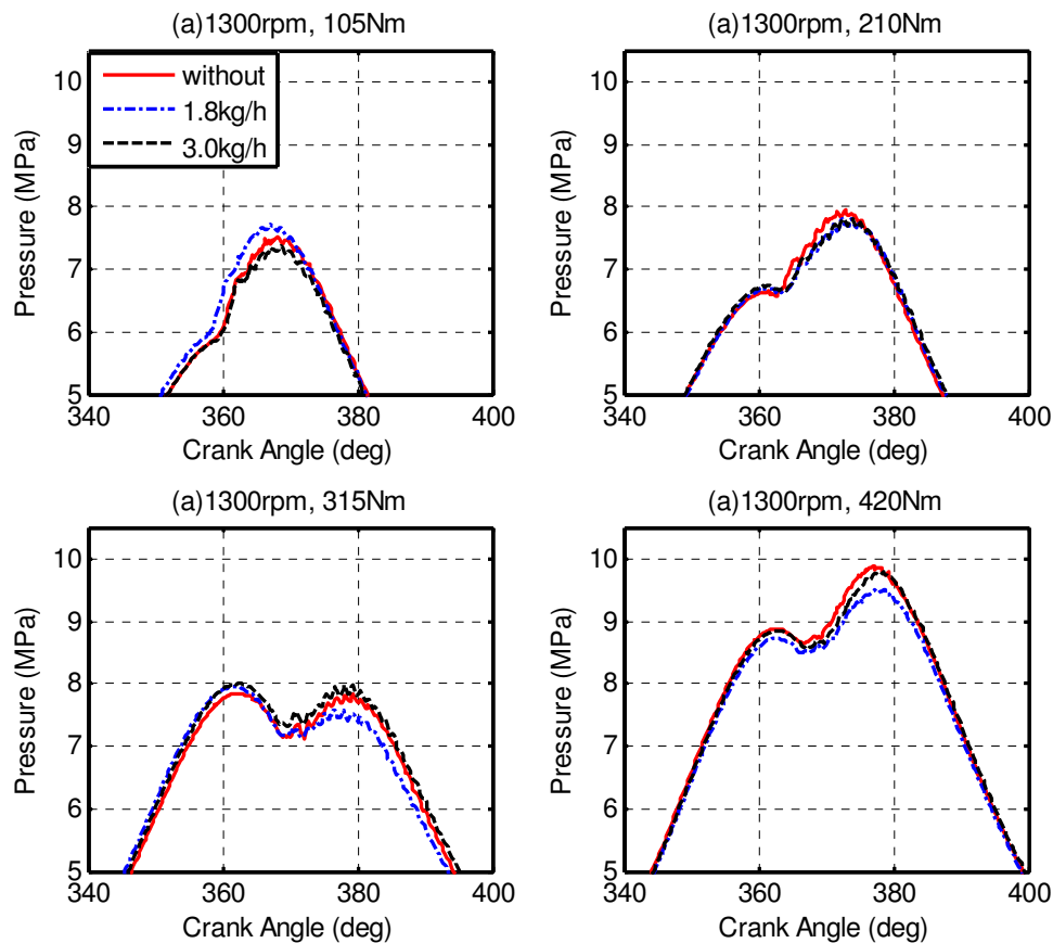
Figure 4 Cylinder pressure at 1300rpm and at different loads
