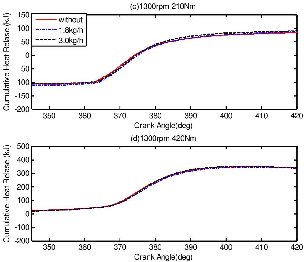
Figure 7 Cumulative heat releases at 1300rpm and different loads
