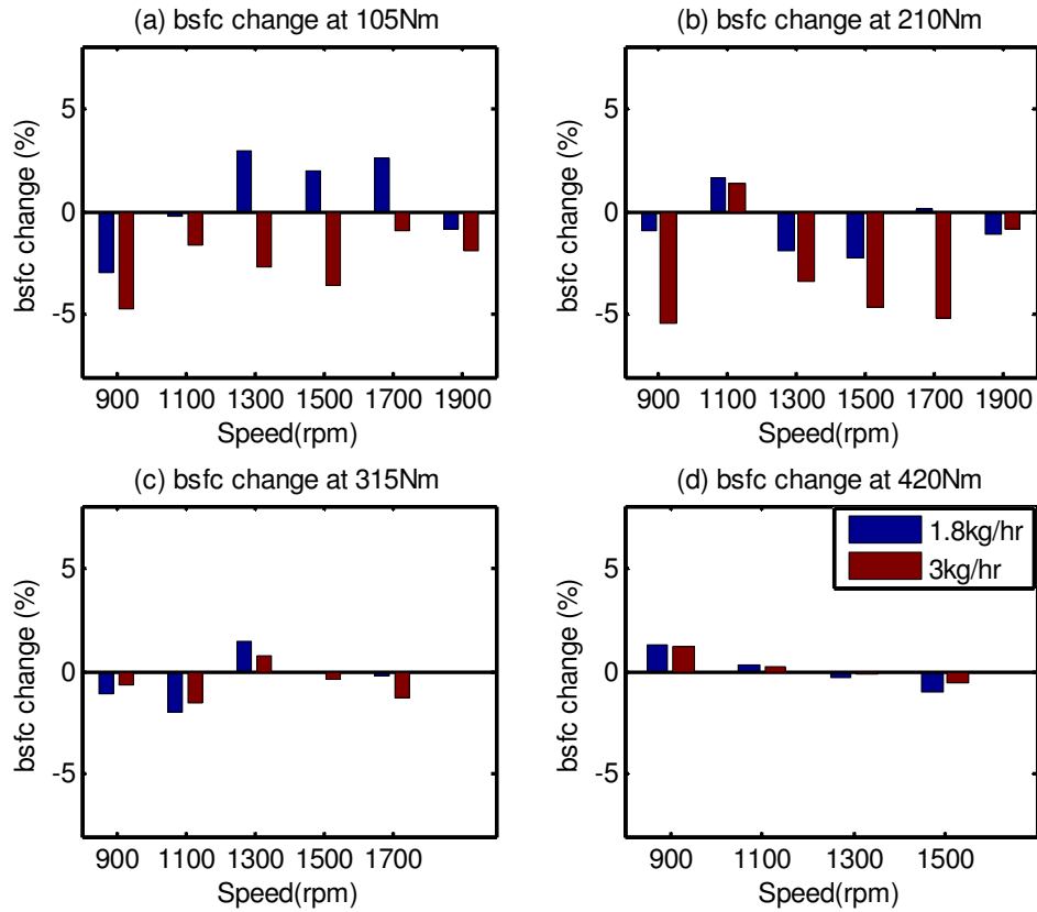
Figure 9 Brake specific fuel consumption (bsfc) at different loads
