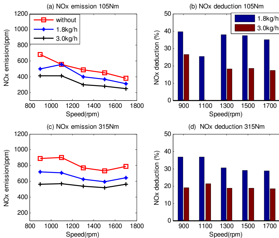
Figure 12 NO x emission and percentage reduction
