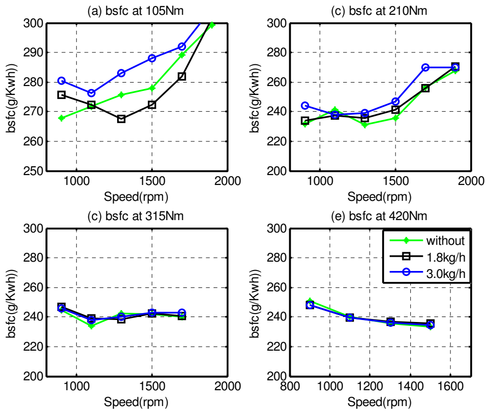
Figure 8 Brake specific fuel consumption (bsfc) at different loads
