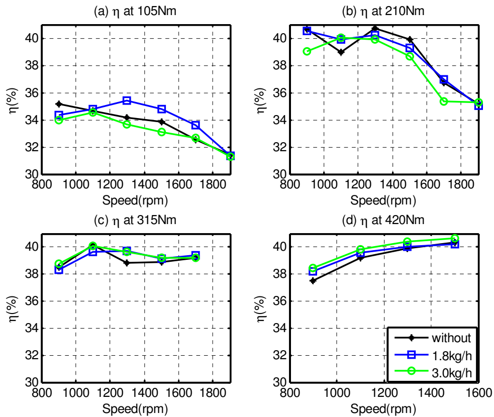
Figure 10 Brake specific fuel consumption (bsfc) at different loads
