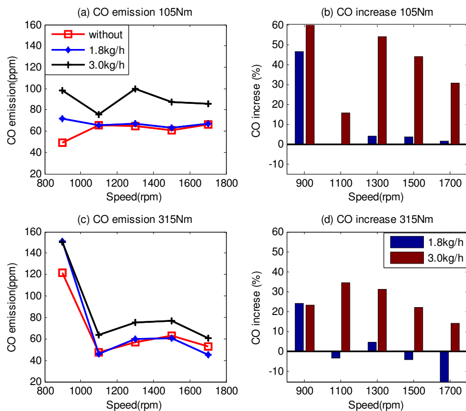
Figure 13 CO emission and percentage increase
