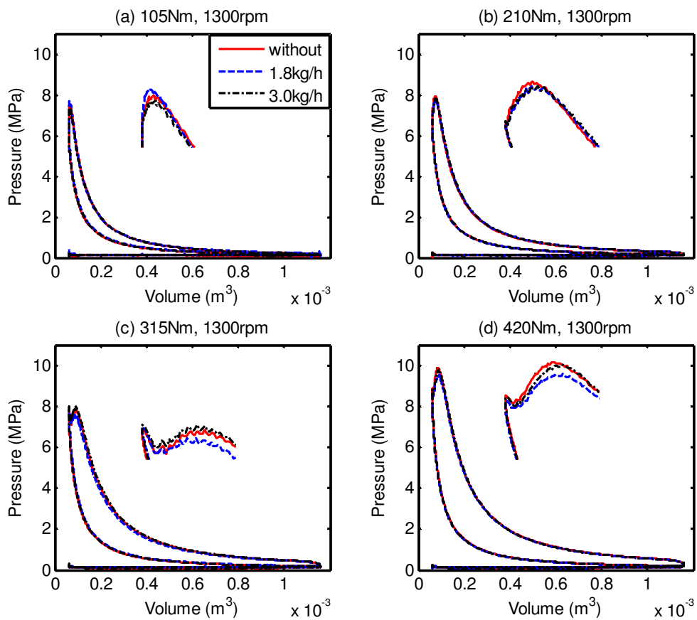
Figure 3 P-V diagram of CI engine at 1300rpm and various engine loads
