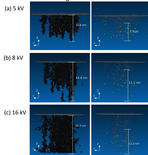
Figure 2. Residual damaged layer (left) and the range of implant Ga^+ (right) formed under different beam voltages.
