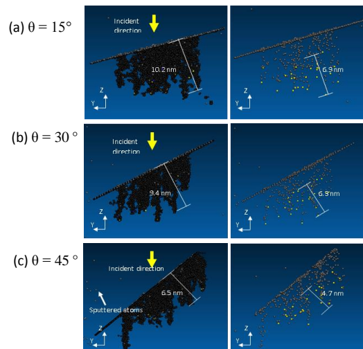
Figure 3. Residual damaged layer (left) and the range of implant Ga^+ (right) formed under different incident angles.
