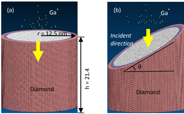
Figure 1. The MD model of FIB milling process. (a) Model I; (b) Model II.
