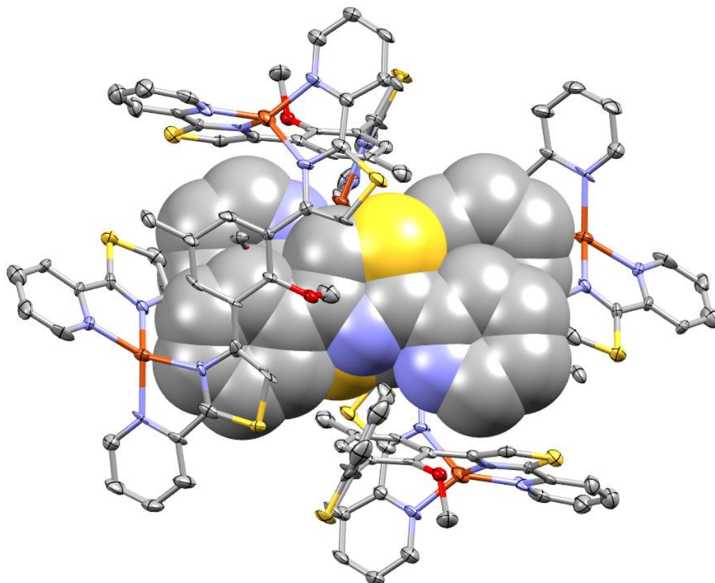
Fig. 78: X-ray crystal structure of [\text{Cu}_6(\text{L}^7)_6]^{6+} with the \pi -stacking interactions between the pyridyl-thiazole-aromatic rings of the central ligands strands shown within the centre of the assembly in spacefilling view. a. Side view of the assembly and b. a birds eye view. Thermal ellipsoids are shown at 50% probability and hydrogen atoms have been omitted for clarity.
