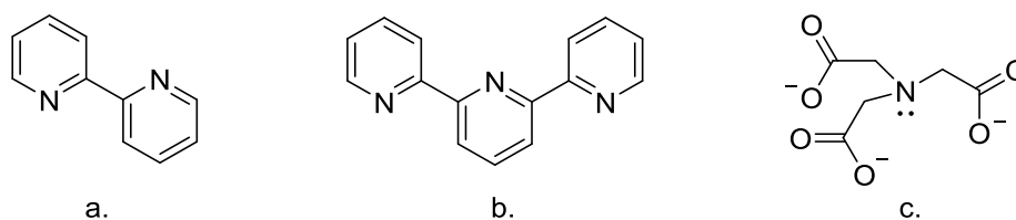
Fig. 12: Examples of various ligands with energetically accessible lone-pairs of electrons. a. The bidentate ligand bipyridine, b. the tridentate ligand terpyridine and c. the tetradentate ligand nitrilotriacetate. 34
