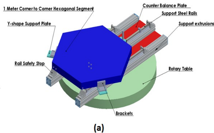
Figure 1. Swinging Part Profilometer; schematic design (a) and prototype (b)
