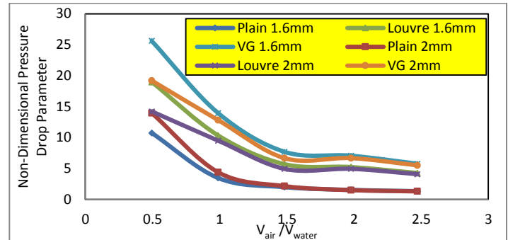
Fig.7 Effect of Velocity Ratio and Area Ratio on the Non-Dimensional Pressure Drop Parameter
