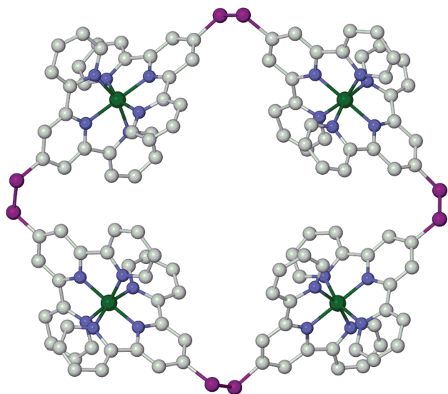
Fig. 1 Crystallographic structure of the \{\text{Fe}(\mu\text{-terpySSterpy})\}_4^{8+} metallacycle (data taken from ref. 20). The \{\text{M}(\mu\text{-bppSSbpp})\}_4^{8+} ( \text{M} = \text{Fe} or \text{Zn} ) assemblies in this work are proposed to have the same connectivity as this structure. Colour code: C, white; Fe, green; N, blue; S, pink.
