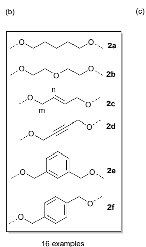
Fig. 2. (a) Synthesis of new flexicates; (b) linking groups used in this study; (c) Sections of 1 H NMR spectra of Λ Zn -[Zn 2 L 2e ] 3 [ClO 4 ] 4 ·4H 2 O at 253 – 353 K in d 2 -acetonitrile showing the higher equilibrium population of a minor asymmetric conformer at higher temperatures.
