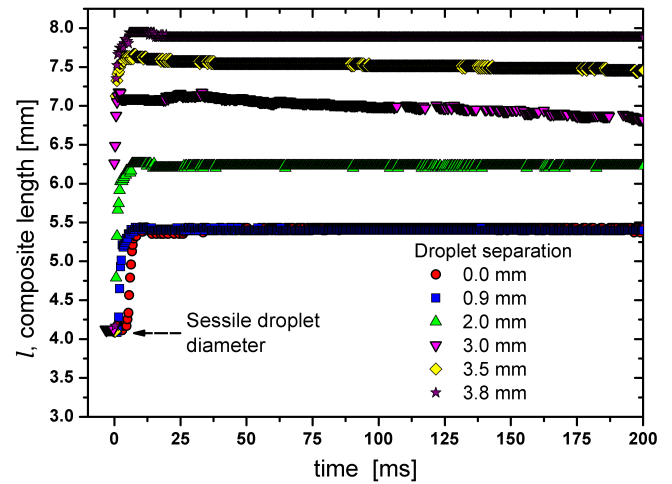
FIG. 12: (Colour online) Temporal evolution of the composite length ( l ) for various droplet separations.
