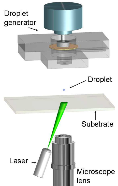
FIG. 1: (Colour online) Schematic view of the experimental arrangement.
