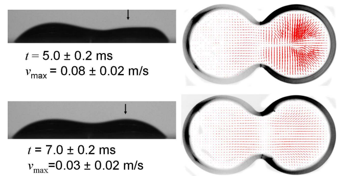
FIG. 9: (Colour online) Velocity fields for the coalescence of two droplets whose centers are separated by 3.80 \pm 0.03 mm. On the left, a shadowgraph image shows a side-view of the coalescence stage at the same time. The reported maximum speed corresponds to the magnitude of the longest vector on the field.
