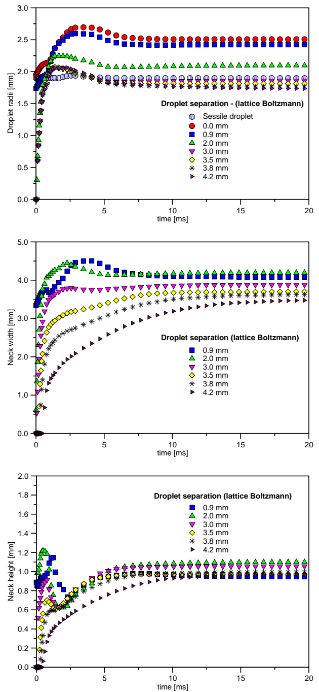
FIG. 14: (Colour online) Evolution of the droplet and neck features calculated from the lattice Boltzmann simulation.
