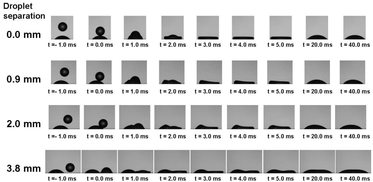
FIG. 10: (Colour online) Side-view shadowgraph imaging of the coalescence of an impacting and a sessile droplet. The droplet separation corresponds to the droplet center to center distance.
