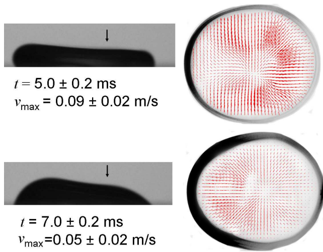
FIG. 7: (Colour online) Velocity fields for the coalescence of two glycerol/water droplets. The center to center separation between the sessile (left) and the impacting (right) droplet is 1.30 \pm 0.03 mm. On the left, a shadowgraph image shows the side-view of the coalescence at the same time. The reported maximum speed corresponds to the magnitude of the longest vector on the field. Note that the downward vertical arrow in the shadowgraphs indicates the center of the impacting droplet.
