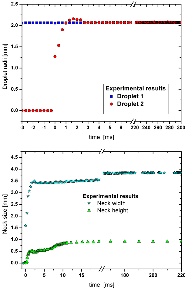
FIG. 11: (Colour online) Temporal evolution of the measured droplet and neck features determined from image processing for a system with a droplet separation of 3.00 mm.
