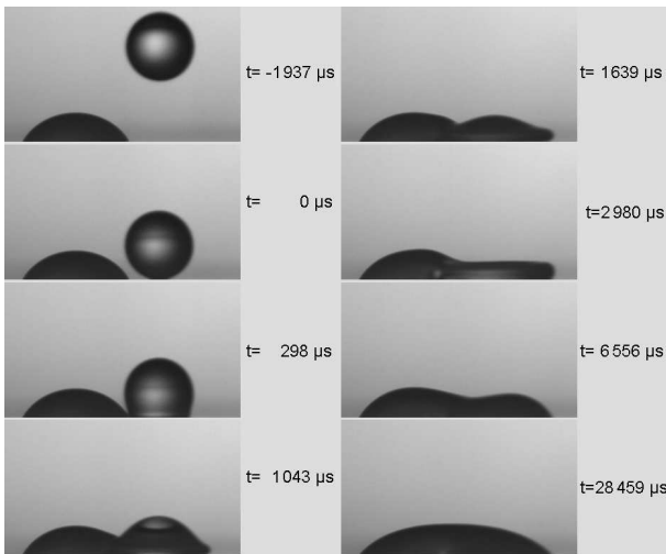
FIG. 3: (Colour online) Examples of images of drop impact and coalescence obtained by high-speed shadowgraphy. In these images the droplet offset is 3.00 \pm 0.05 mm. In both this series and the one in Fig. 2, the time t = 0 \mu s corresponds to the image showing the impacting droplet at the closest position to the substrate. As a consequence, a systematic timing error of up to 150 \mu s can exist between this side view and the bottom view shown in Fig. 2.
