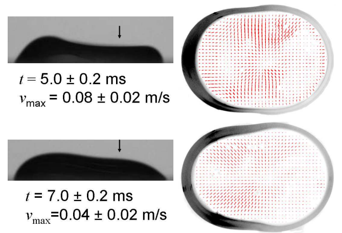
FIG. 8: (Colour online) Velocity fields for the coalescence of two droplets whose centers are separated by 2.00 \pm 0.03 mm. On the left, a shadowgraph image shows the side-view of the coalescence at the same time. The reported maximum speed corresponds to the magnitude of the longest vector on the field.
