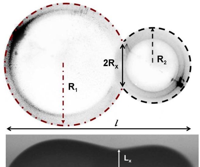
FIG. 4: (Colour online) Diagram showing the quantities determined by the image processing. The dotted line indicates the position of the contact line. R_1 is the radius of the sessile drop, R_2 is the radius of the impacting drop, R_x is the neck width, l is the composite length and L_x is the neck height.
