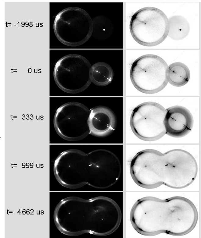
FIG. 2: (Colour online) Examples of images of drop impact and coalescence obtained from the high speed imaging setup for the case of a droplet separation of 3.00 \pm 0.05 \text{ mm} . The left-hand images are the original images. The right-hand images are digital negatives which assist the visualization of the contact line position.
