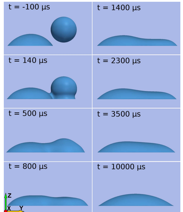
FIG. 5: (Colour online) Lattice Boltzmann simulation of droplet impact and coalescence corresponding to that in Fig. 3.
