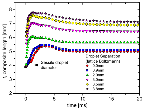
FIG. 16: (Colour online) Evolution of composite droplet length calculated from the lattice Boltzmann simulation.
