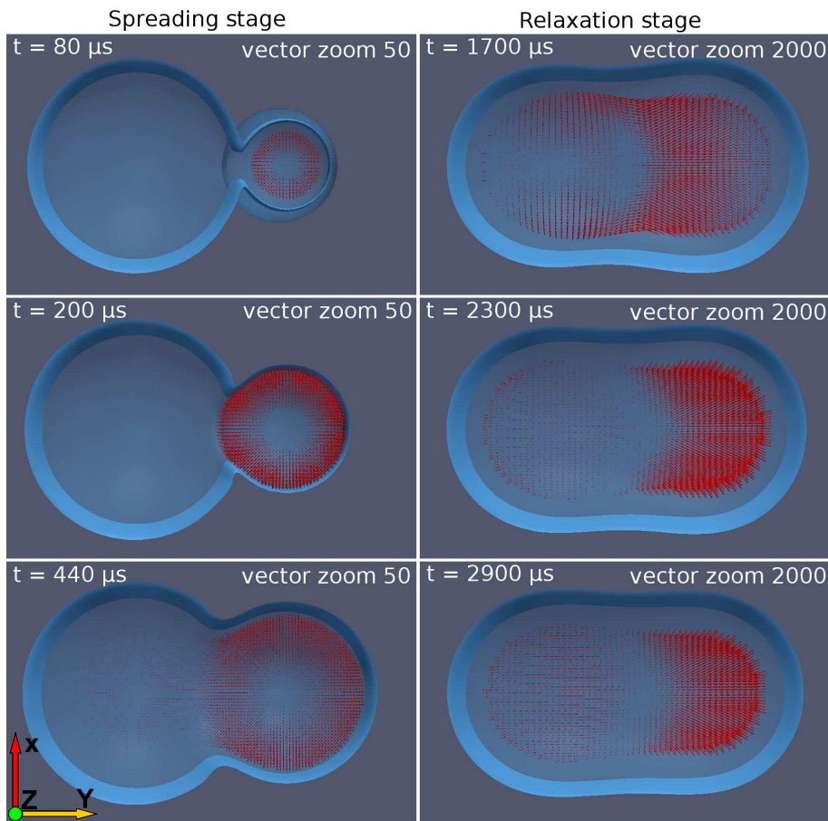
FIG. 15: (Colour online) Velocity fields calculated from the Lattice Boltzmann simulation of the coalescence of two droplets. The droplet on the right had impacted the substrate at a time = 0 \mu\text{s} , the droplet on the left was deposited in a previous simulation and is considered sessile; the droplet separation is 3.00 mm. Note that for clarity the velocity vectors are shown at different scales in the two columns. The longest vector in the left-hand column corresponds to a speed of 1.5 \text{ m s}^{-1} ; the longest vector in the right-hand column represents 0.05 \text{ m s}^{-1}
