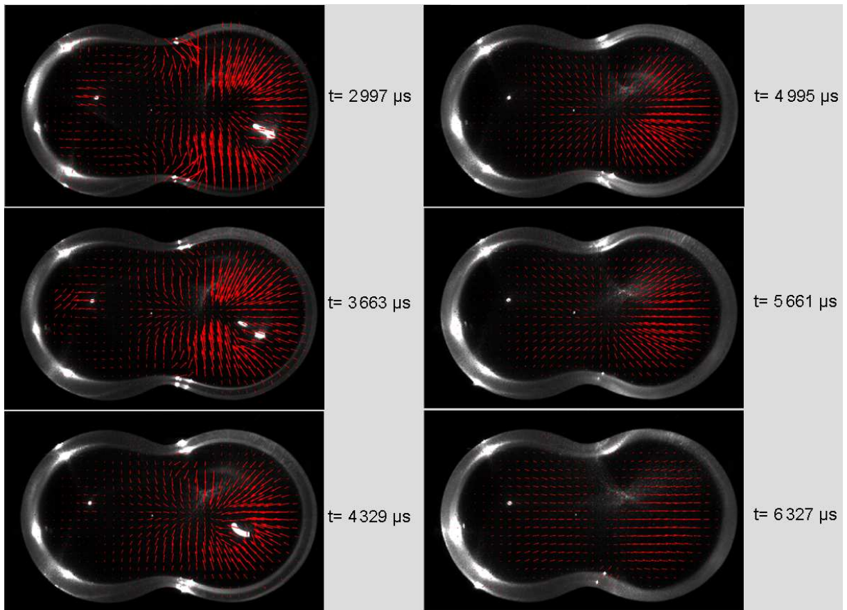
FIG. 6: (Colour online) Velocity fields for the coalescence of two glycerol/water droplets. The droplet on the right had impacted the substrate at a time t = 0 \mu\text{s} ; the droplet on the left had been deposited 10 s earlier and can be considered sessile. The droplet separation is of 3.00 \pm 0.05 \text{ mm} . The velocity vectors around the laser reflections are spurious and should be ignored.
