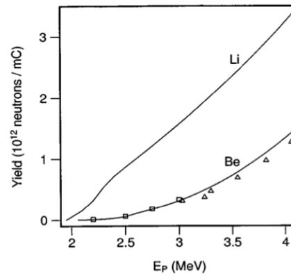
Figure 4: Total experimental neutron yields for a thick lithium target from cross-sections from [9] and a beryllium with data from [10]. Direct neutron yields for a beryllium target are from [8] (squares) and [11] (triangles).
