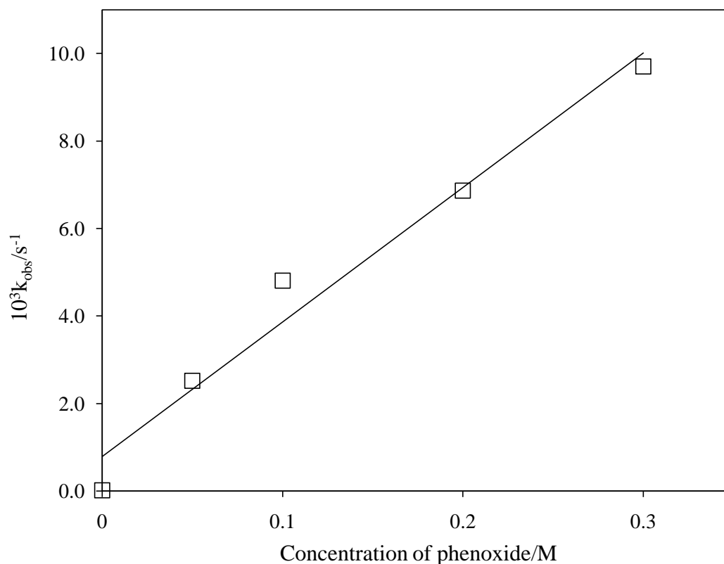
Figure 4.1 The dependence of the pseudo first order rate constants on the concentration of phenoxide ion for the reaction between 4-NFB and sodium phenoxide in \text{LNH}_3 at 25\text{ }^\circ\text{C} ( I = 0.3\text{M} , \text{KClO}_4 ).
