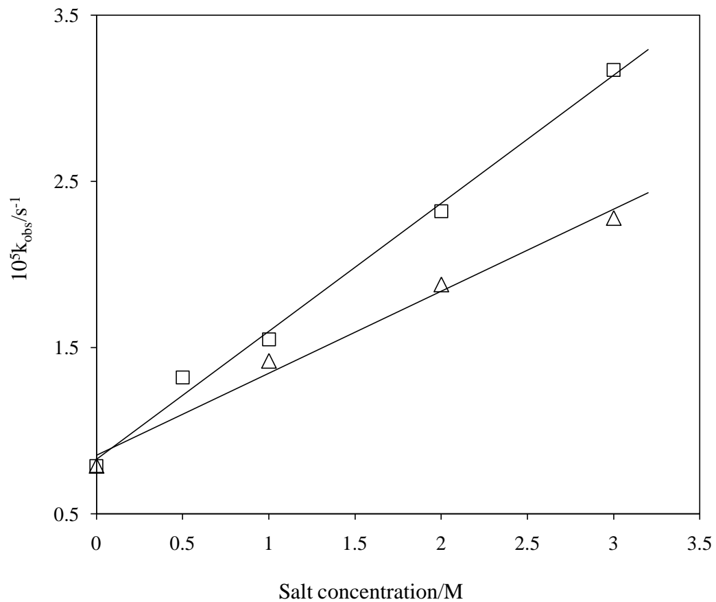
Figure 2.5 The first order rate constants for the solvolysis of 4-NFB as a function of added salt concentration in \text{LNH}_3 at 25\text{ }^\circ\text{C} . ( \Delta ) \text{NH}_4\text{Cl} ; ( \square ) \text{NaNO}_3
