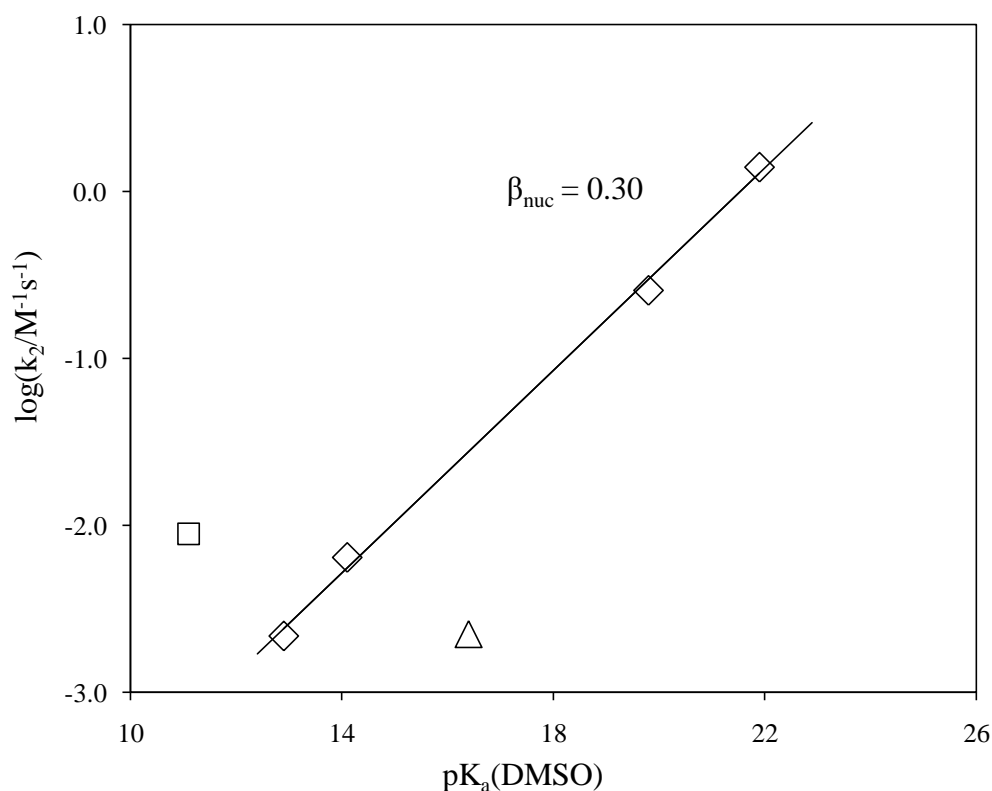
Figure 3.9 Brønsted plot for the reactions of some carbanions with benzyl chloride in liquid ammonia at 25 °C using the pK_a of their conjugate acids in DMSO. ( \square ) Shows malonodinitrile positively deviated from the line, and ( \triangle ) shows malonate diethyl ester negatively deviated from the line.
