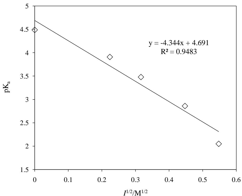
Figure A8 Linear relationship of \text{pK}_a of 4-chlorophenol ( 1 \times 10^{-4} \text{M} ) with the square root of ionic strength ( I , \text{KClO}_4 ) in \text{LNH}_3 at room temperature
