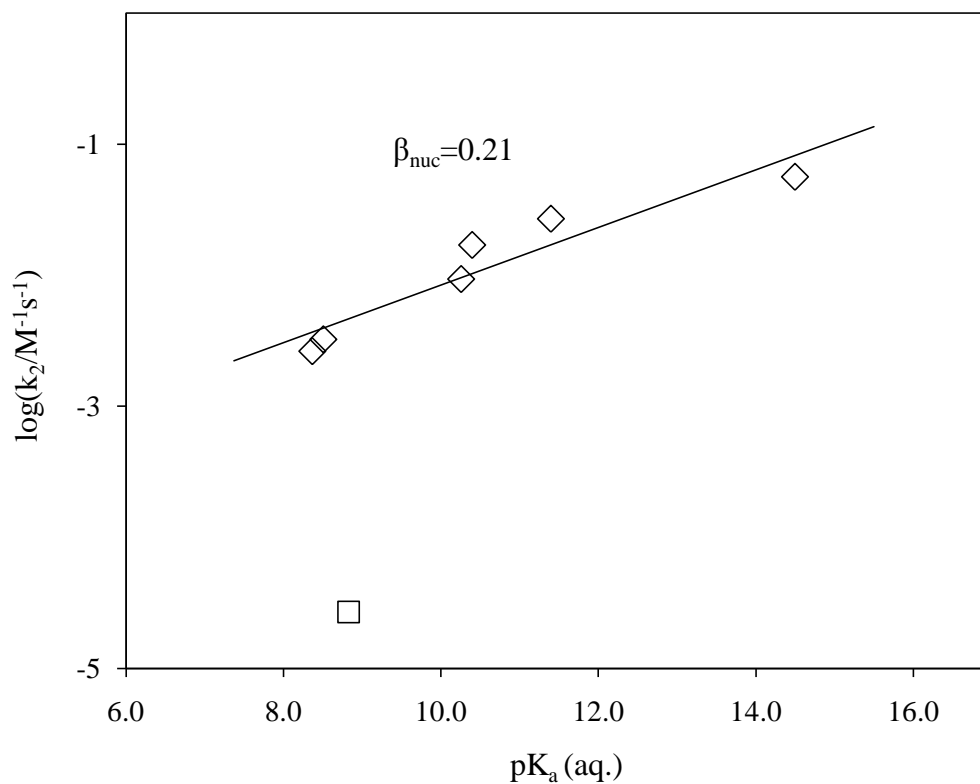
Figure 3.7 The Brønsted plot for the substitution of benzyl chloride by various amines in \text{LNH}_3 at 25 °C, ammonia (□) is negatively deviated from the line, but the positive deviation of azide anion is not shown.
