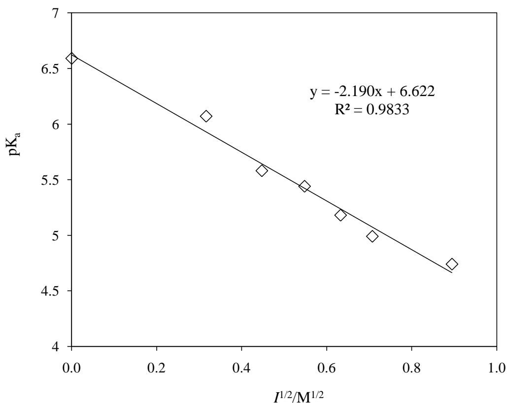
Figure A5 Linear relationship of \text{pK}_a of 4-methoxyphenol ( 3 \times 10^{-4} \text{M} ) with the square root of ionic strength ( I , \text{KClO}_4 ) in \text{LNH}_3 at room temperature
