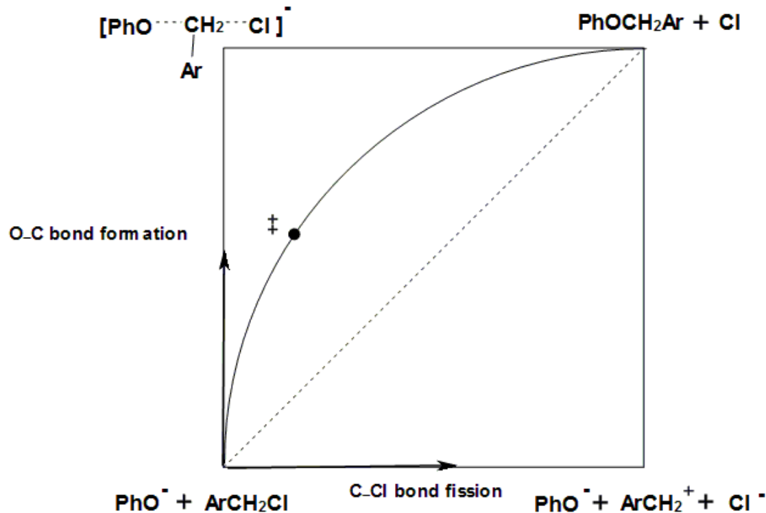
Figure 3.5 Jencks-More O'Ferrall reaction diagram for the reaction between phenoxide anion and benzyl chlorides in \text{LNH}_3 at 25^\circ\text{C}
