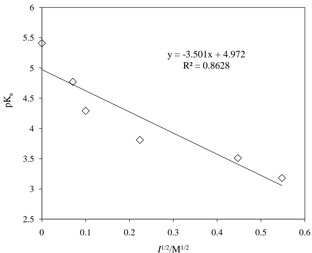
Figure A7 Linear relationship of \text{pK}_a of 1-naphthol ( 1 \times 10^{-4} \text{M} ) with the square root of ionic strength ( I , \text{KClO}_4 ) in \text{LNH}_3 at room temperature
