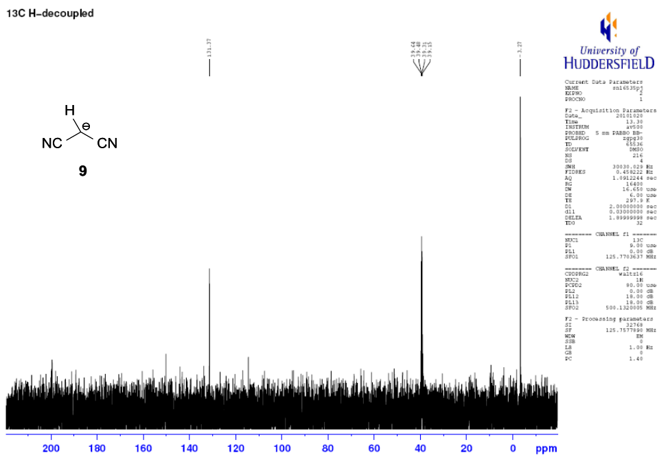
Figure N26 13 C H-decoupled NMR Spectrum of 0.1M malononitrile with 2 eq. NaNH 2 in liquid ammonia at 25 °C
