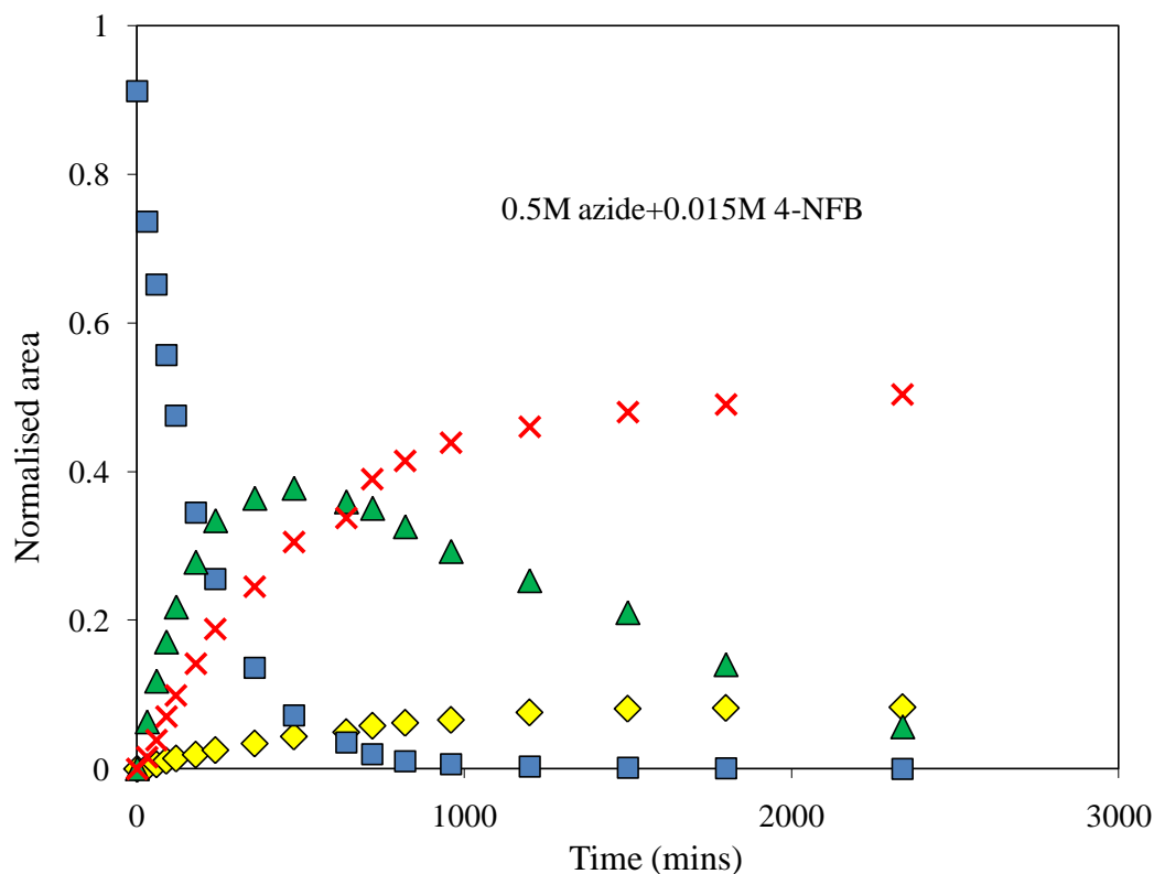
Figure 4.7 The reaction profile for 4-NFB reacting with sodium azide in \text{LNH}_3 at 25^\circ\text{C} (■ : 4-NFB; × : 4-nitroaniline; ▲ : 4-NAB; ◆ : nitrobenzene)
