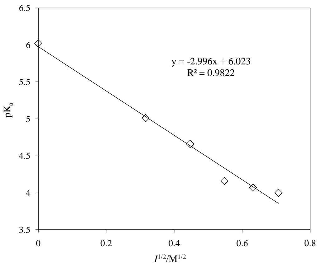
Figure A6 Linear relationship of pK_a of phenol ( 3 \times 10^{-4} M ) with the square root of ionic strength ( I , KClO_4 ) in LNH_3 at room temperature
