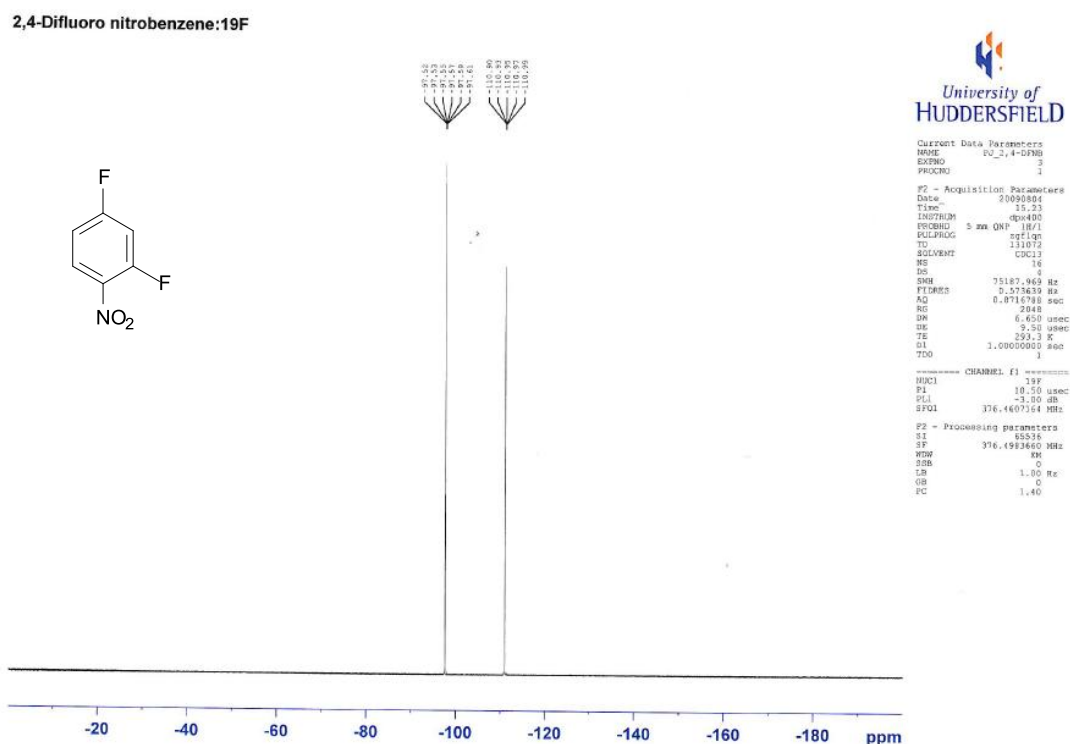
Figure N28 19 F NMR Spectrum of 2,4-difluoronitrobenzene in DMSO-d 6 at 25 °C
