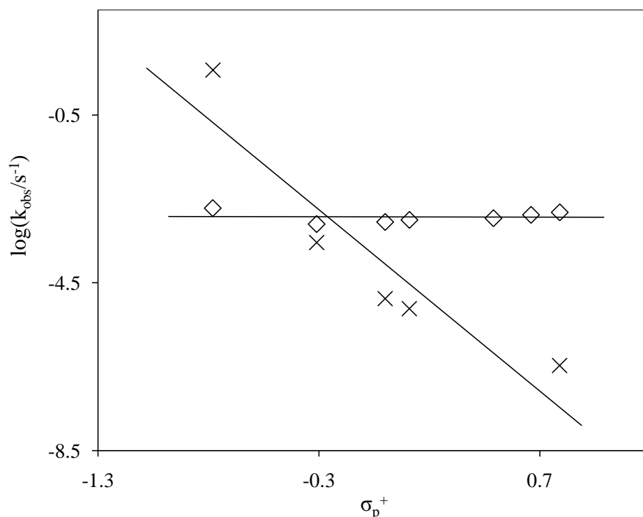
Figure 2.1 The Hammett plot for the solvolysis of 4-substituted benzyl chlorides in LNH_3 ( \diamond ) and water ( \times ) at 25 °C.
