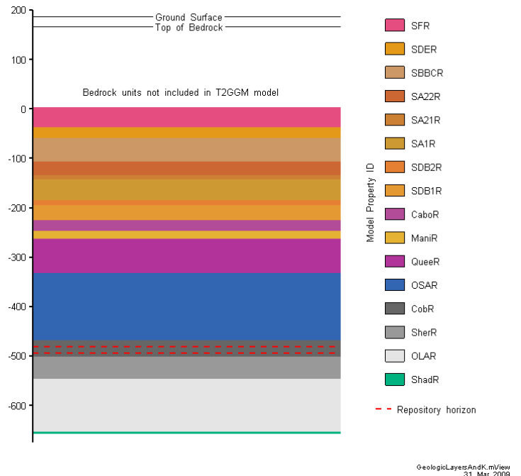
Figure 4: Geologic layering in the gas transport model
