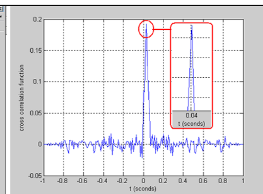
Figure 13: The cross-correlation signal for the two signals
