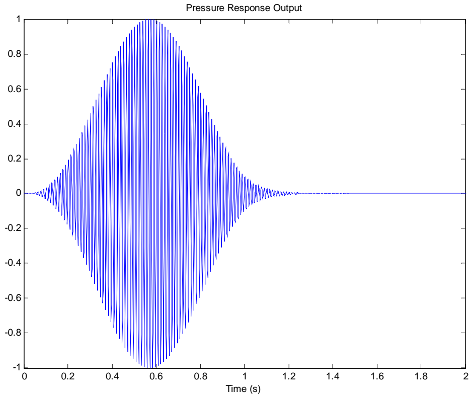
Figure 7.7 – Output response of a single resonance at 80 Hz when subjected to a smoothly varying 80 Hz sine burst.
