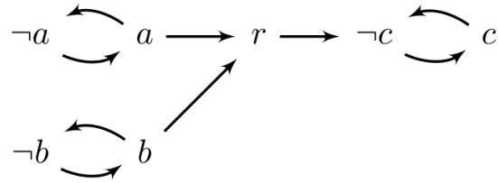
Figure 4 AF derived from r : \neg a, \neg b \rightarrow c .
