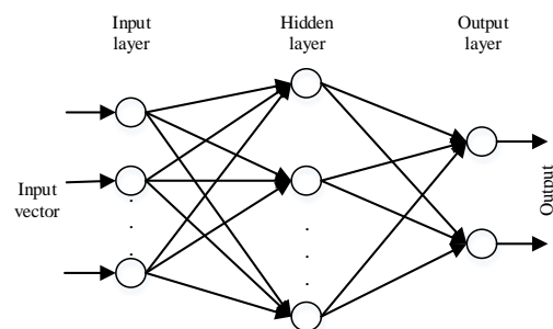
Fig. 1. MLP Architecture
