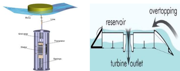
Fig. 11. Swedish heaving buoy Fig. 12. Overtopping WEC: the Wave Dragon The typical devices of Poly wave reservoir include Wave Dragon, developed by Denmark Wave Company, Mighty whale, the Wave power generation device in Japanese, and Agucadoura wave power station in Portugal [40-42].
