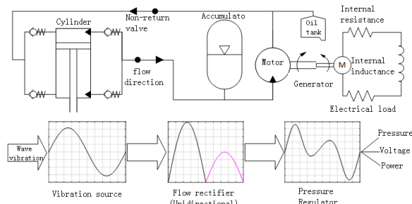
Fig. 1. Schematic diagram of VEH power generation
