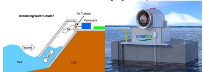
Fig. 2. Schematic diagram of OWC structure Fig. 3. Oceanlinx OWC device
