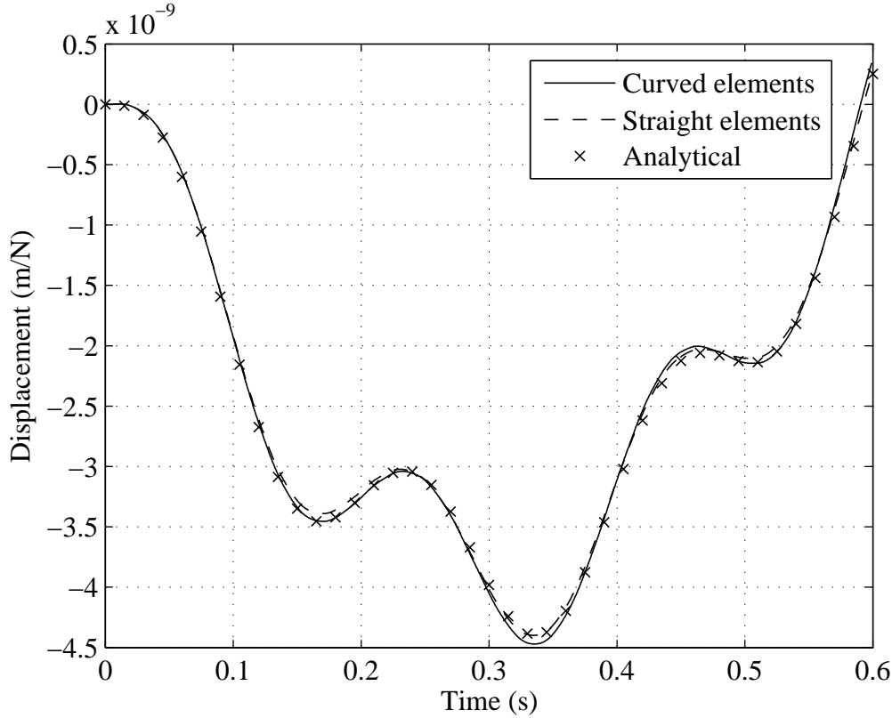
Figure 5: Transfer function for the comparison of the curved track using curved and straight beam elements against the analytical solution for a constant moving load with velocity V = 40m/s on a track of length L_t = 24m over an angle \phi = 30^\circ
