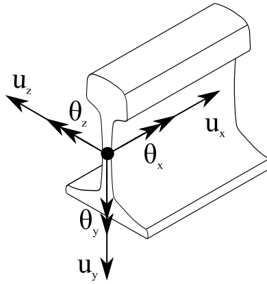
Figure 3: Degrees of freedom per node.
