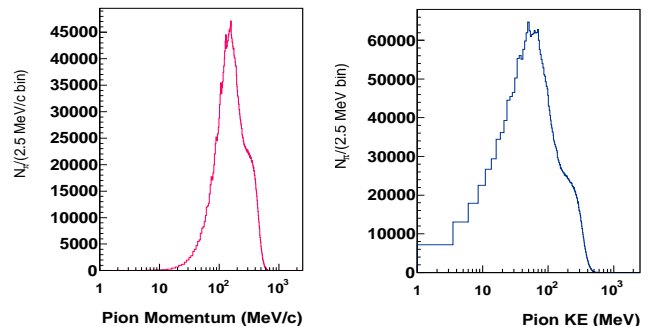
(a) 750 MeV
