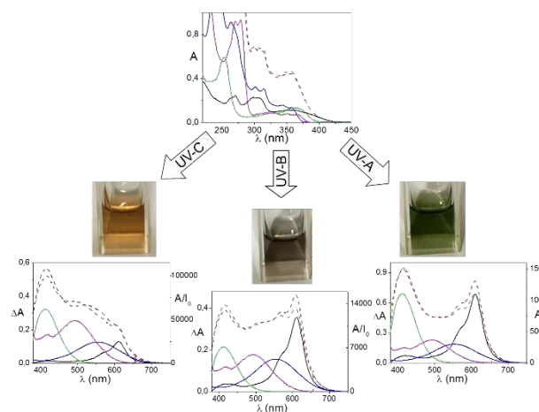
Figure 3. Response of the quaternary photochromic Fuzzy Logic System to electromagnetic radiation belonging to the UV-A, UV-B and UV-C regions, respectively. Continuous traces represent the calculated spectral contribution of 1 (black), 4 (green), 2 (magenta), 5 (blue); their algebraic sum gives the red dashed traces. The grey dashed traces represent the spectra recorded experimentally using 125 W Xe lamp as irradiation source. In the three plots, \Delta A is obtained by subtracting the spectrum recorded at the photo-stationary state from the initial one; A/I_0 represents the total absorbance in the visible calculated by equation (2), divided by the total intensity ( I_0 ) at \lambda_{irr} .
