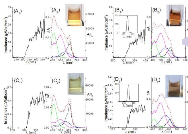
Figure 4. Response of the quaternary Photochromic Fuzzy Logic System to electromagnetic radiation belonging to different regions of UV. In each panel the left-hand side plot represents the spectrum of the irradiation source, whereas the plot on the right shows the experimental spectrum (grey dashed trace) compared with the calculated spectrum (red dashed trace) obtained by summing the contributions of 1 (black continuous trace), 4 (green continuous trace), 2 (magenta continuous trace) and 5 (blue continuous trace). On the right-hand plot of each panel there is also a picture of the irradiated solution. The top-left panel is relative to direct sunlight at 11 a.m.; the top-right panel is relative to direct sunlight at 11 a.m. plus irradiation at 254 nm emitted by a Hg lamp; the bottom-left-hand panel is relative to skylight and the bottom-right panel is relative to skylight plus irradiation at 254 nm emitted by a Hg lamp.
