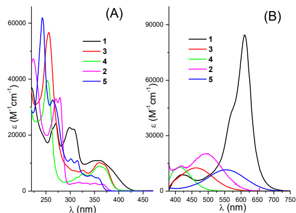
Figure 2. Quantitative absorption spectra (recorded in MeCN) of the closed uncoloured (A) and open coloured (B) forms of 1 (black traces), 3 (red traces), 4 (green traces), 2 (magenta traces), and 5 (blue traces).
