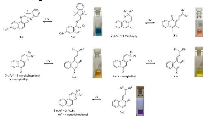
Figure 1. Structures of the five closed uncoloured ( 1c – 5c ) photochromic compounds and their ring-opened coloured forms ( 1o – 5o ). The pictures show the colours they produce in MeCN solutions upon UV irradiation.
