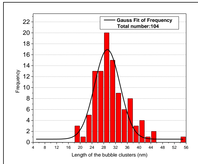
Fig 4.10: Final length distribution of bubble discs at 900 °C at a fluence of 6.1 \times 10^{16} \text{ ions.cm}^{-2}
