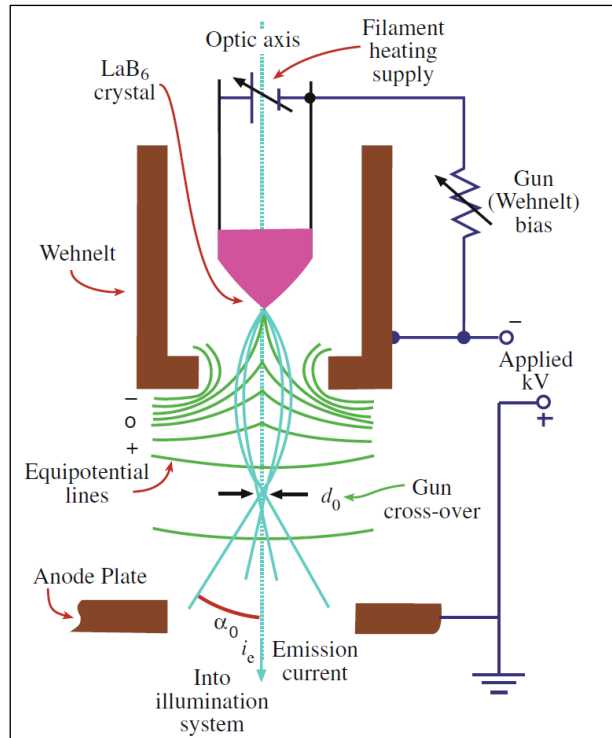
Fig 3.7: Schematic of the thermionic electron source ( \text{LaB}_6 ) (reproduce from [72])
