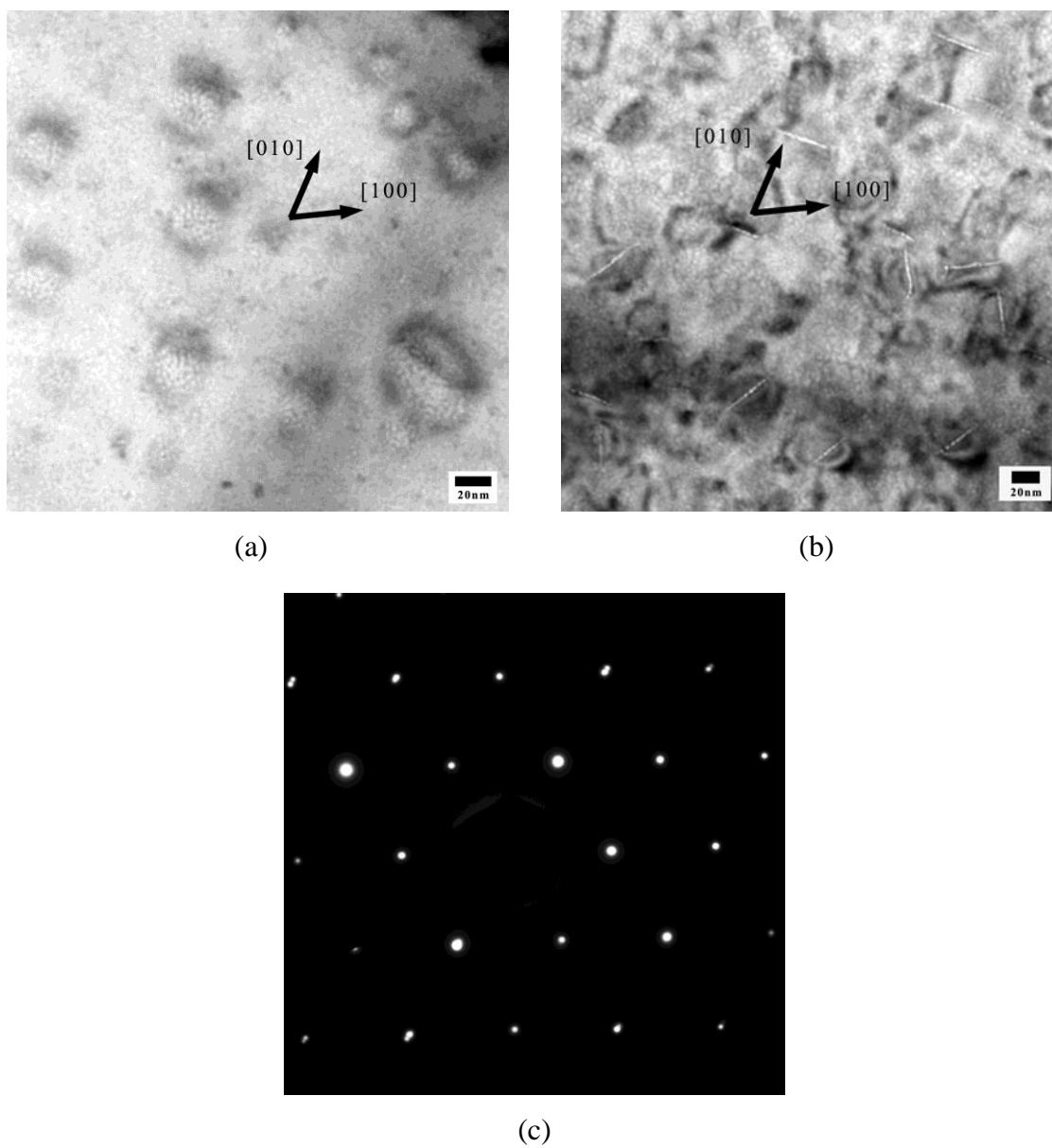
Fig 4.4: Plan-view (a) and edge-on (b) bubble discs at a fluence of 6.1 \times 10^{16} ions.cm -2 at 900 °C; (c) the corresponding diffraction pattern.
