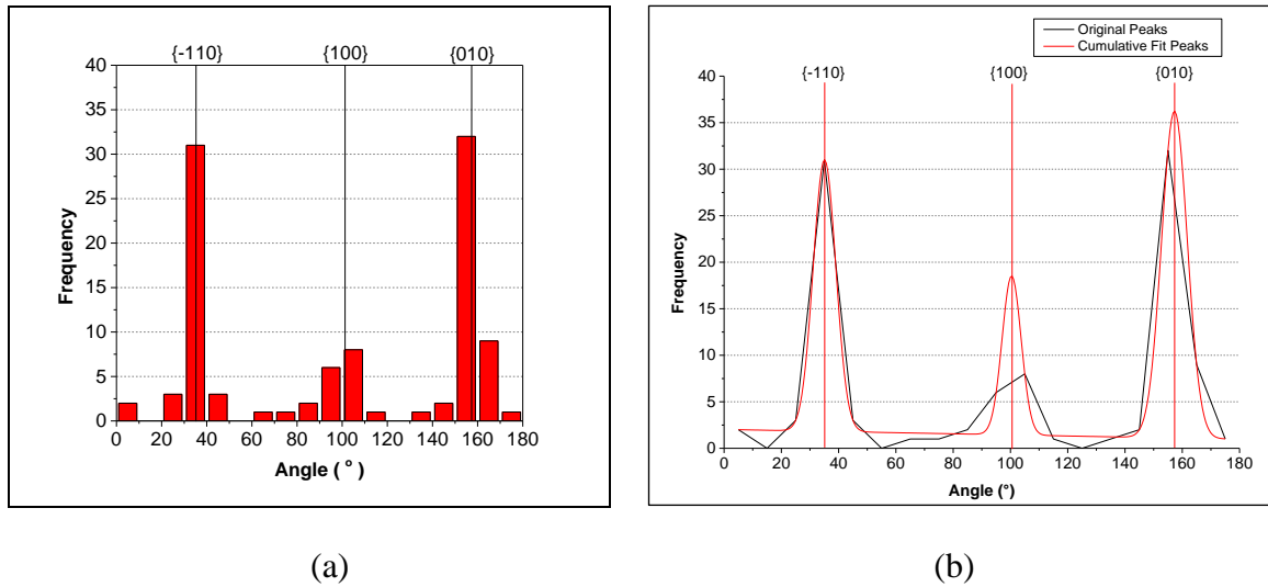
Fig 4.12: Distribution of the angles of the bubble discs and fitting curve at 900 °C at a fluence of 6.1 \times 10^{16} \text{ ions.cm}^{-2}
