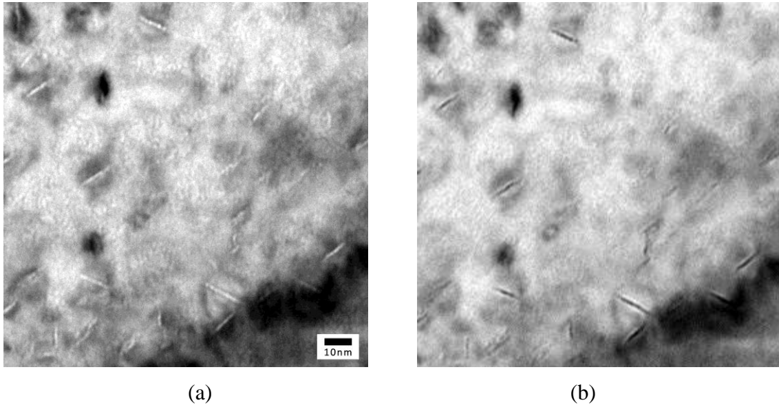
Fig 4.3: TEM images of bubbles and edge-on bubble discs at 6.1 \times 10^{16} \text{ ions.cm}^{-2} at 800 °C viewed close to [001] zone-axis. (a) underfocus (-60 nm), (b) overfocus (+60 nm). Scale bar applies to both images.
