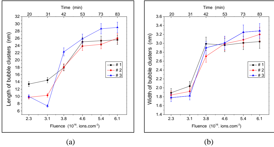
Fig 4.7: The length (a) and width (b) increase of bubble discs at 800 °C with increasing He fluence. Note that the time on the upper axis includes irradiation time and the holding time required for image capture (during which irradiation was not performed but the sample was held at temperature).
