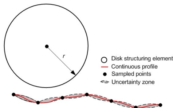
Figure 18. Uncertainty zone for continuous surface profile reconstruction with the disk
