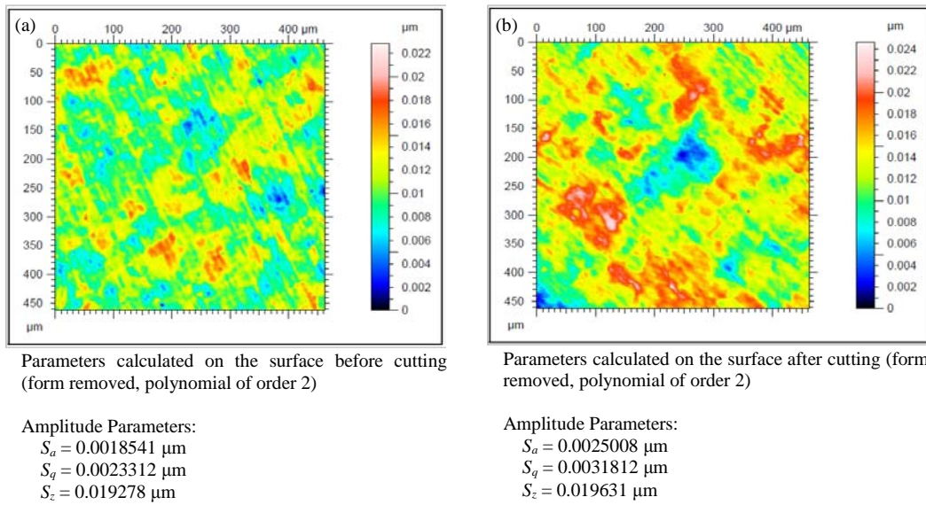
Figure 3: The surface roughness of workpiece (a) before nanoscale multi-tip tool cutting, and (b) after nanoscale multi-tip tool cutting (the lens was focused on the surface region between each cutting pass).
