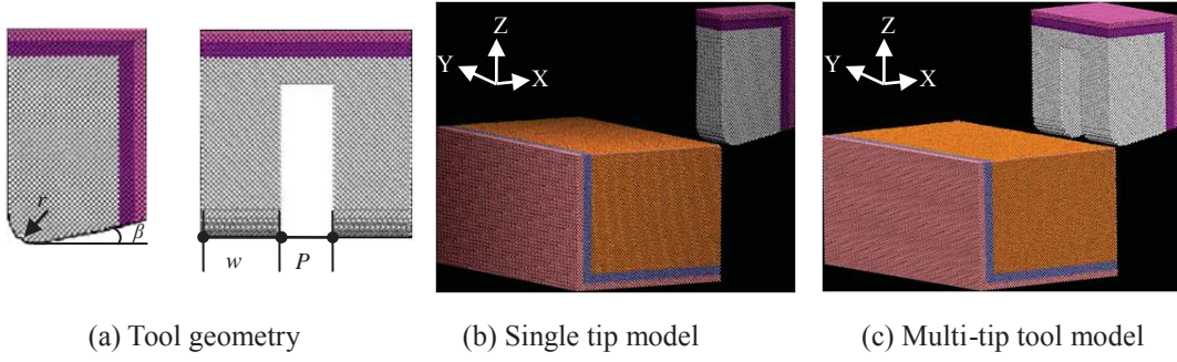
Figure 1. Models of MD cutting simulation
