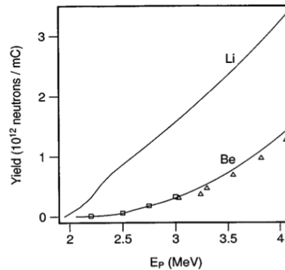
Figure 4: Total experimental neutron yields for a thick lithium target from cross-sections from [9] and a beryllium target with data from [10]. Direct neutron yields for a beryllium target are from [8] (squares) and [11] (triangles).
