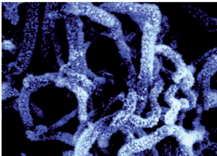
Figure 1. Scanning electron micrograph showing zinc nanoparticle decoration of polycyanoacrylate in a fingerprint developed with multiple techniques, revealed by backscattered electron contrast.
