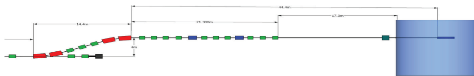
Figure 1: The HEFT-S3 - 2D layout which includes the magnets - quadrupoles (green), dipoles (red) and octupoles (blue), the fixed collimator (cyan) and the target monolith (including the proton beam window and the target wheel).
