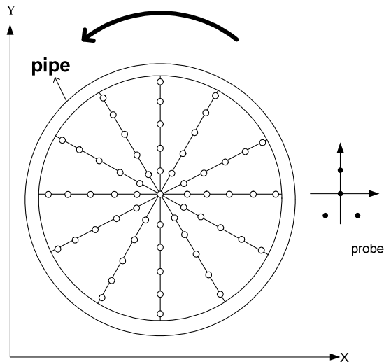
Figure 15 Data collection points in the flow loop
