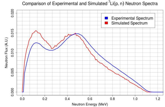
Figure 2: The simulated (red line) and experimental (blue line) neutron spectrum from the {}^7\text{Li}(p, n) reaction.
