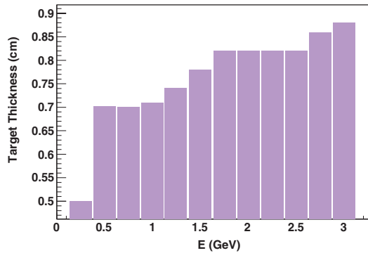
FIG. 6. Target thickness for 96% proton transmission through the muon target as a function of proton beam energy.
