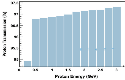
FIG. 5. Proton transmission through the muon target as a function of the proton beam energy.
