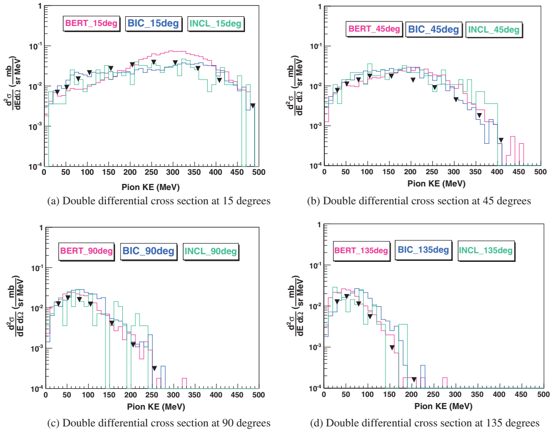
FIG. 3. Double differential cross section for positive pion production at 15, 45, 90, and 135 degrees with respect to the proton beam. Simulations using three physics lists (QGSP-BERT, QGSP-BIC, QGSP-INCL-ABLA) and experimental data are compared.
