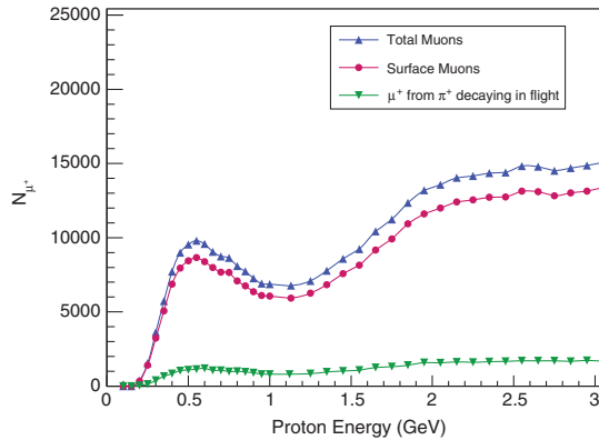
FIG. 11. Variation of muon yield with proton energy.
