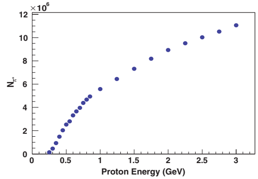
FIG. 7. Variation of pion yield with proton energy.
