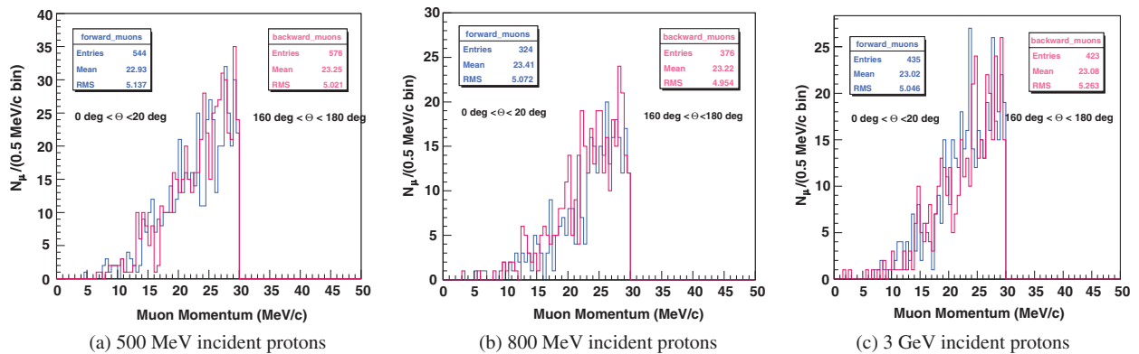
FIG. 16. Surface muon momentum distributions for various incident proton energies.
