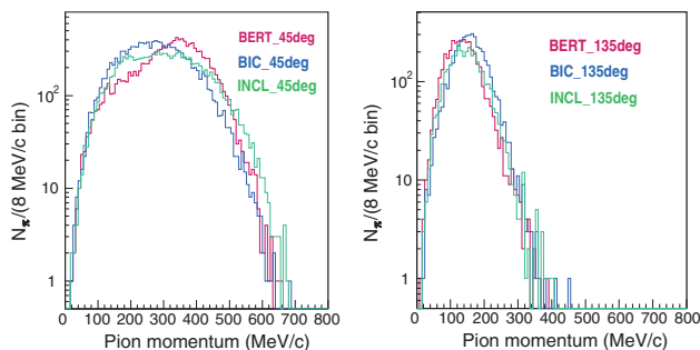
FIG. 4. Pion momentum spectra predicted by three hadronic models, Bertini, Binary, and INCL-ABLA. Detectors are placed diagonally opposed at 45 and 135 degrees with respect to the proton beam.
