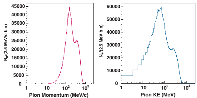
FIG. 9. Pion momentum and energy spectra for incident proton energy of 1 GeV.
