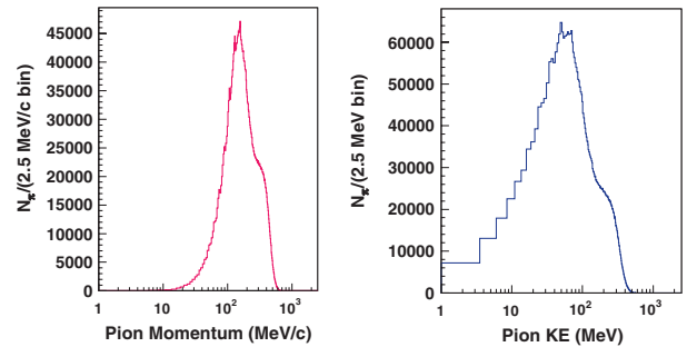
FIG. 8. Pion momentum and energy spectra for incident proton energy of 750 MeV.
