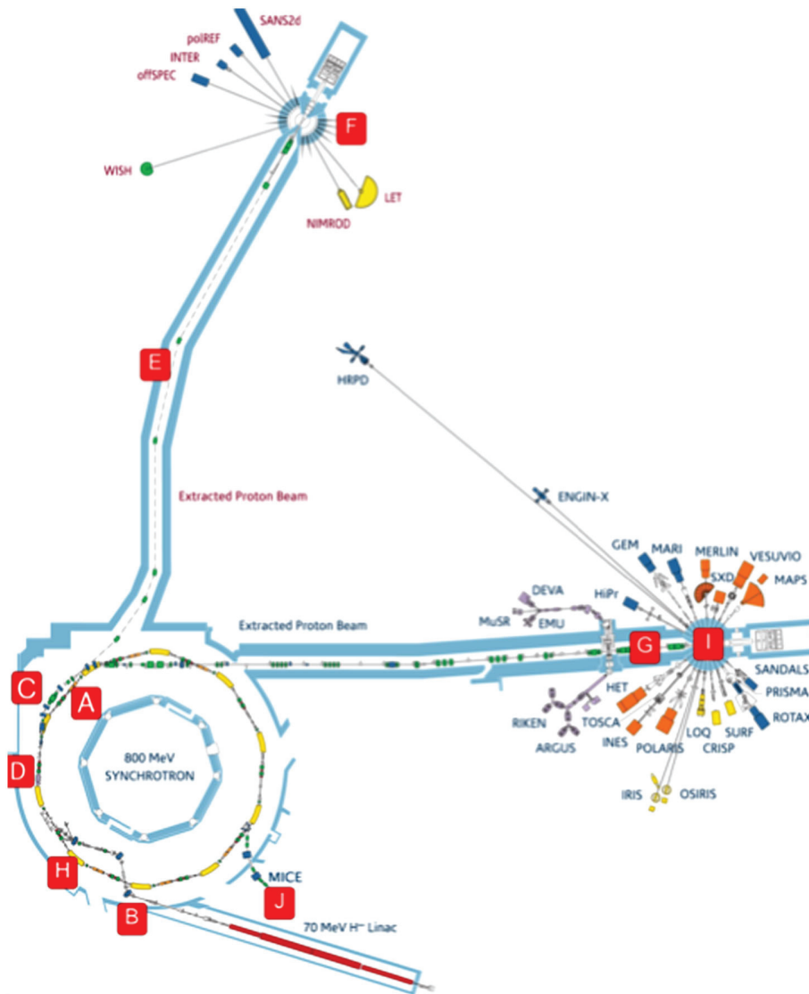
FIG. 1. Layout of the ISIS facility at the Rutherford Laboratory. The muon target (G) is situated 20 m upstream of the neutron target (I). The second neutron target is also shown (F).
