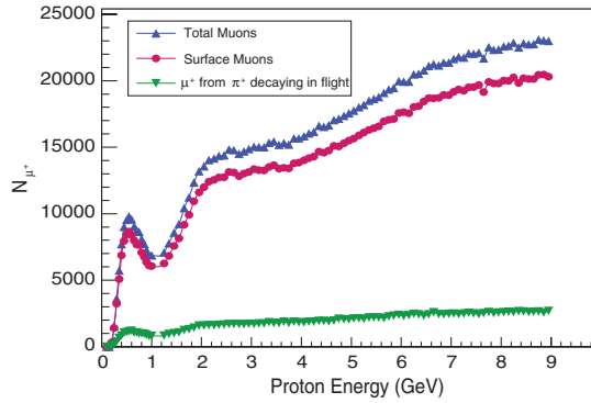
FIG. 14. Variation of muon yield with proton energy at higher energies.
