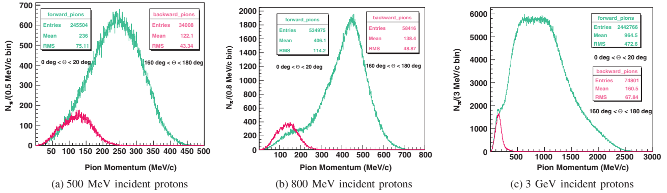
FIG. 10. Pion momentum distributions at various incident proton energies.
